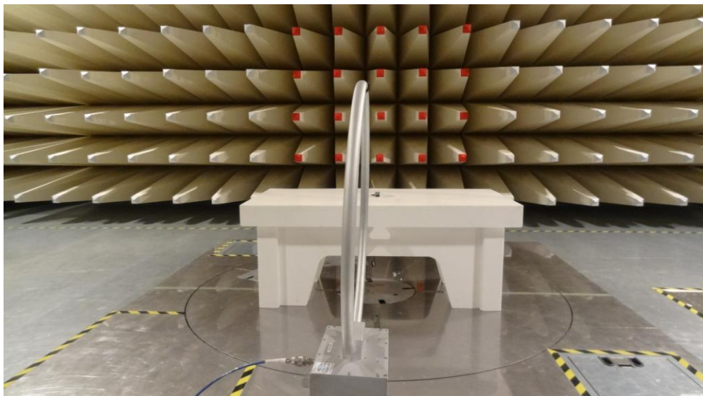
Test setup
