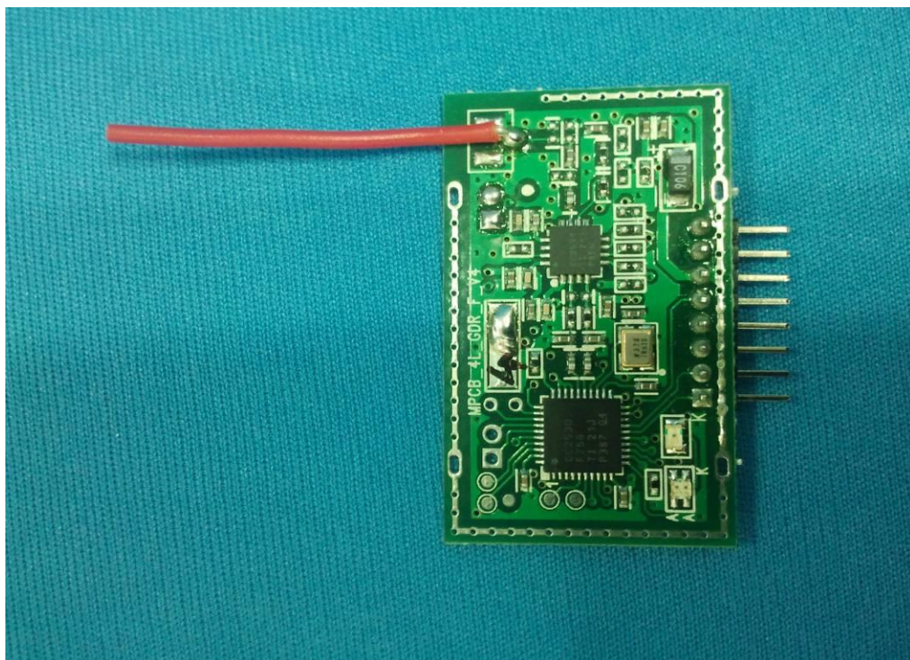
RF Module Top View (Shield Removed)
