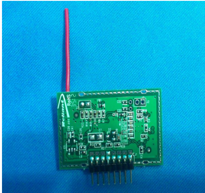
RF Module Bottom View
