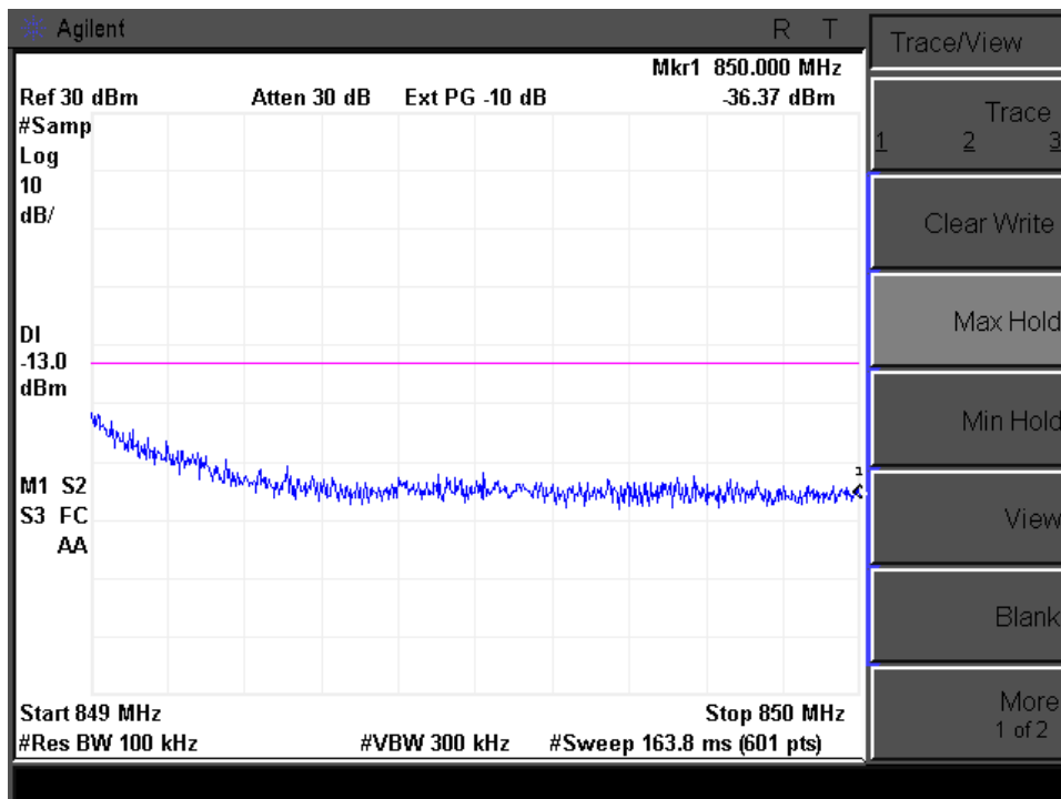
Conducted Band Edge plot on channel 4233
