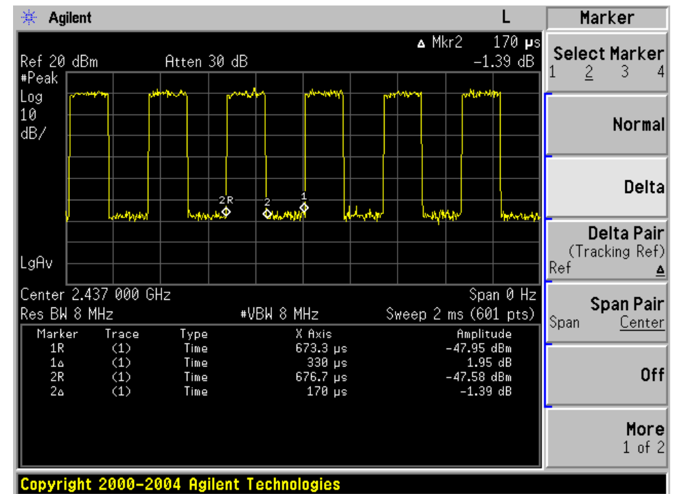
Duty Cycle plot on channel 6
