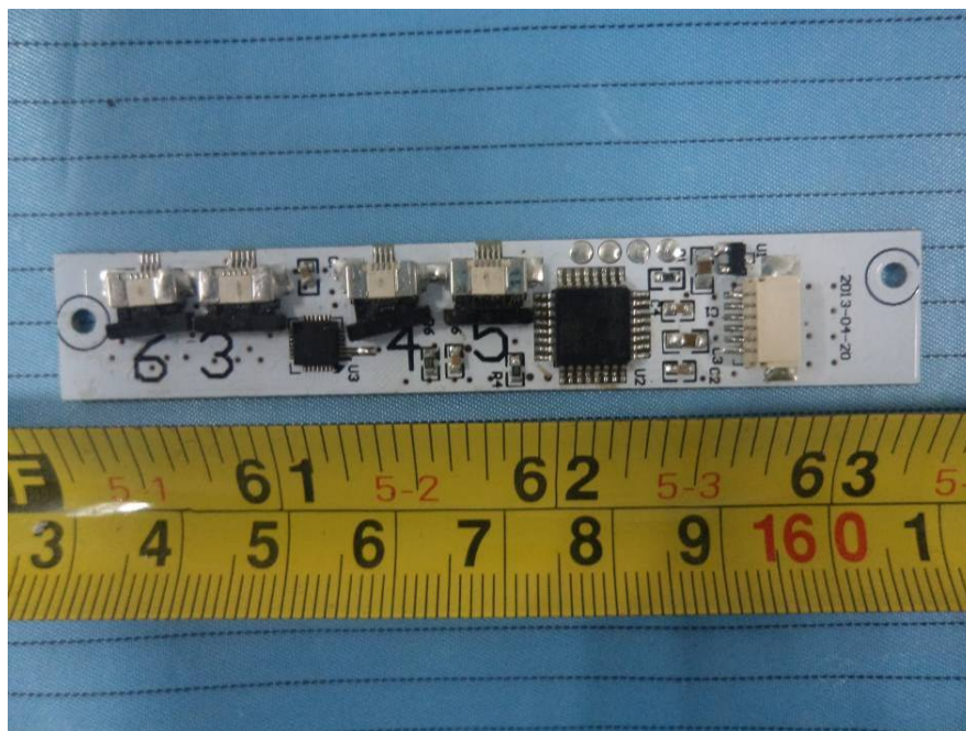
EUT – Halo LED Board Top View
