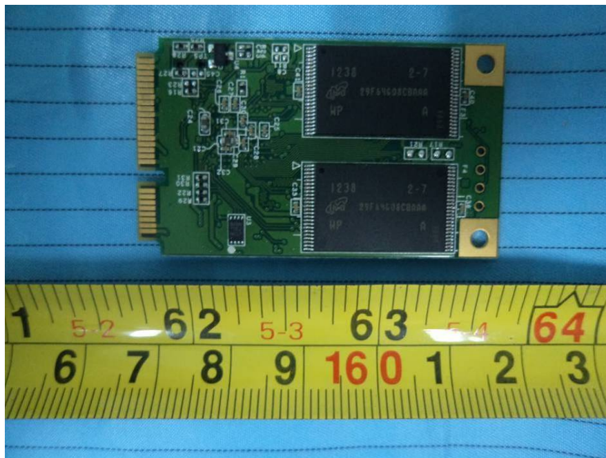
EUT – 32G Disk Board Bottom View
