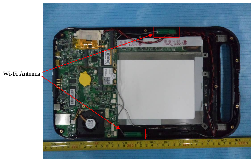
EUT – Cover off View (8pin, without Halo LED)
