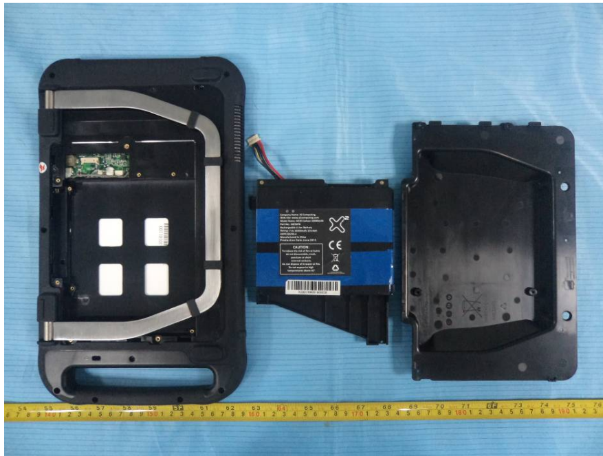
EUT – Battery off View (with 16000mAh Battery)
