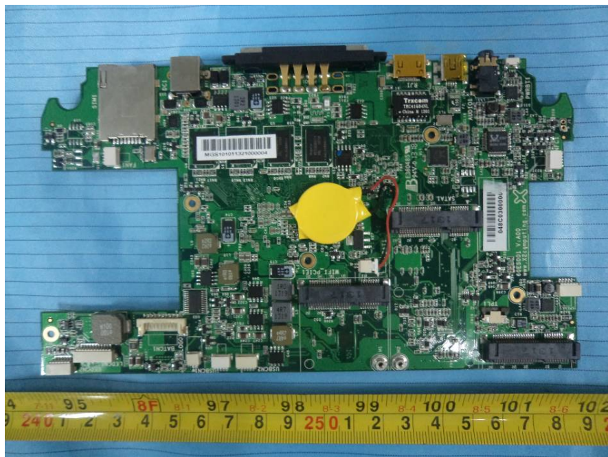
EUT – 8pin Main Board Top View
