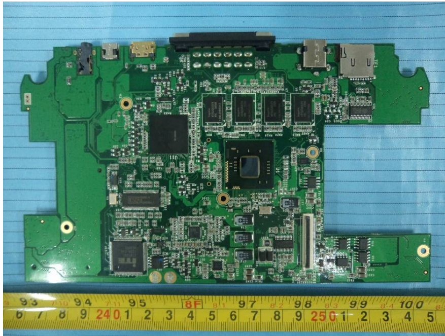
EUT – 12pin Main Board Bottom View
