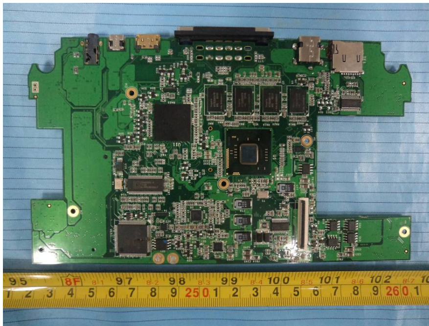
EUT – 8pin Main Board Bottom View
