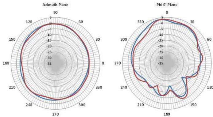
1950 MHz
