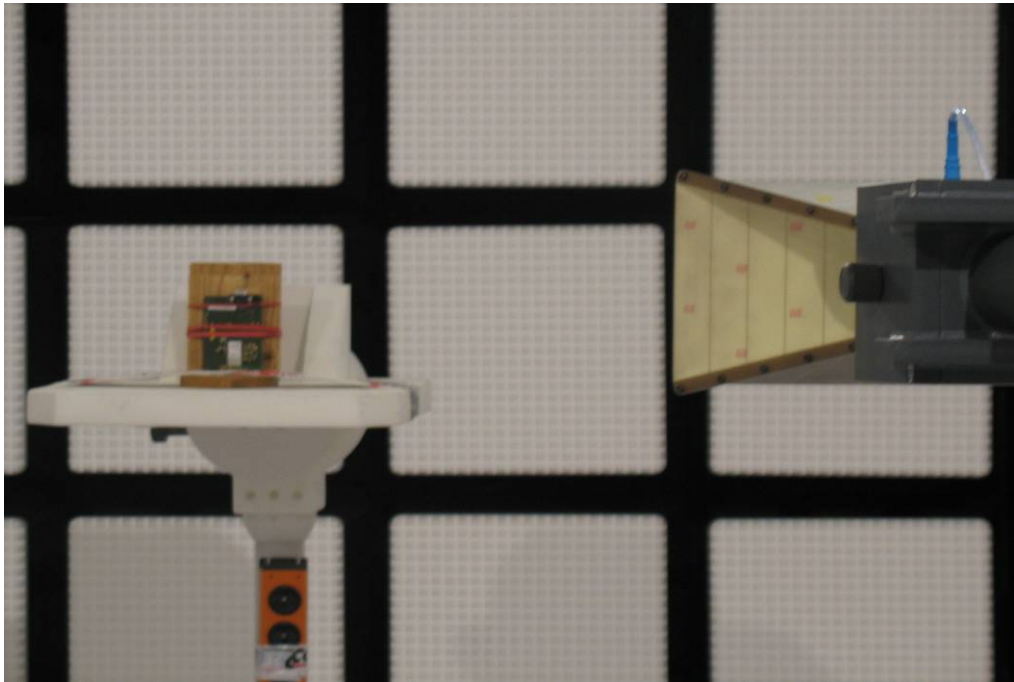
Photo 5: Pre-scan position for spurious radiated measurements >1GHz
