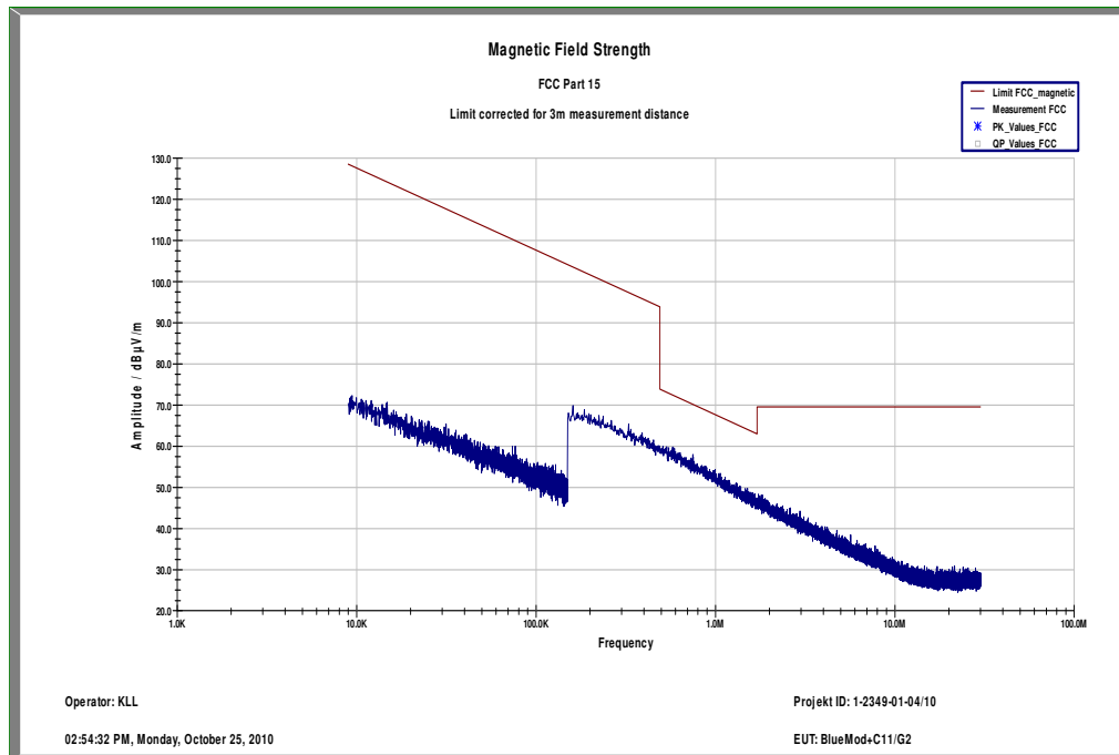
Plot 1: 9 kHz to 30 MHz / channel 00, GFSK (valid for all channels and modes)
