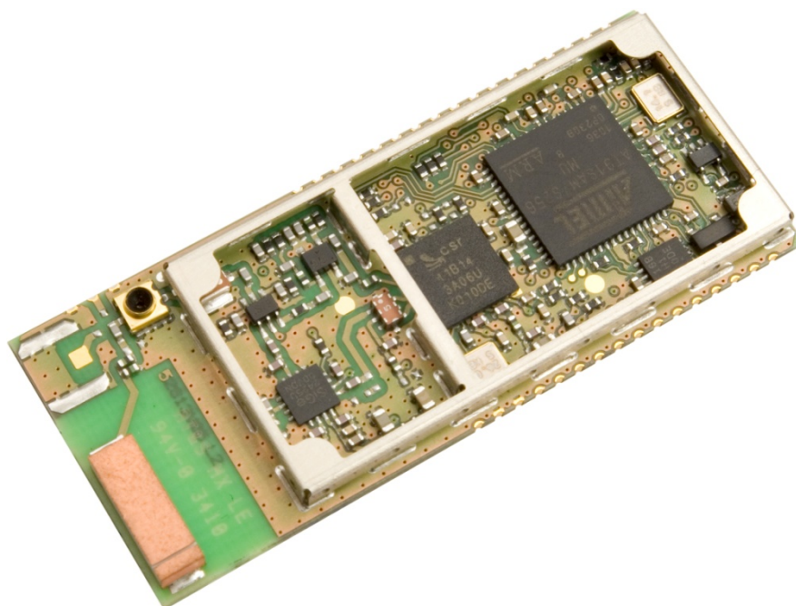
BlueMod+C11/G2/AI without Shield
