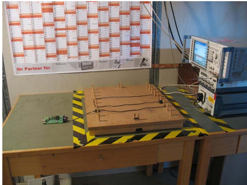
Photo 3: Conducted Emissions
