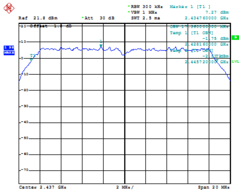
Mode 8 : 99% Occupied Bandwidth Plot on 802.11n Channel 06
