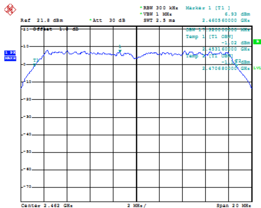
Mode 9 : 99% Occupied Bandwidth Plot on 802.11n Channel 11
