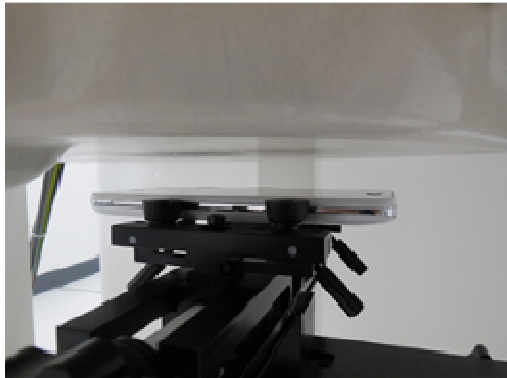
Body position Front with gap 10mm
