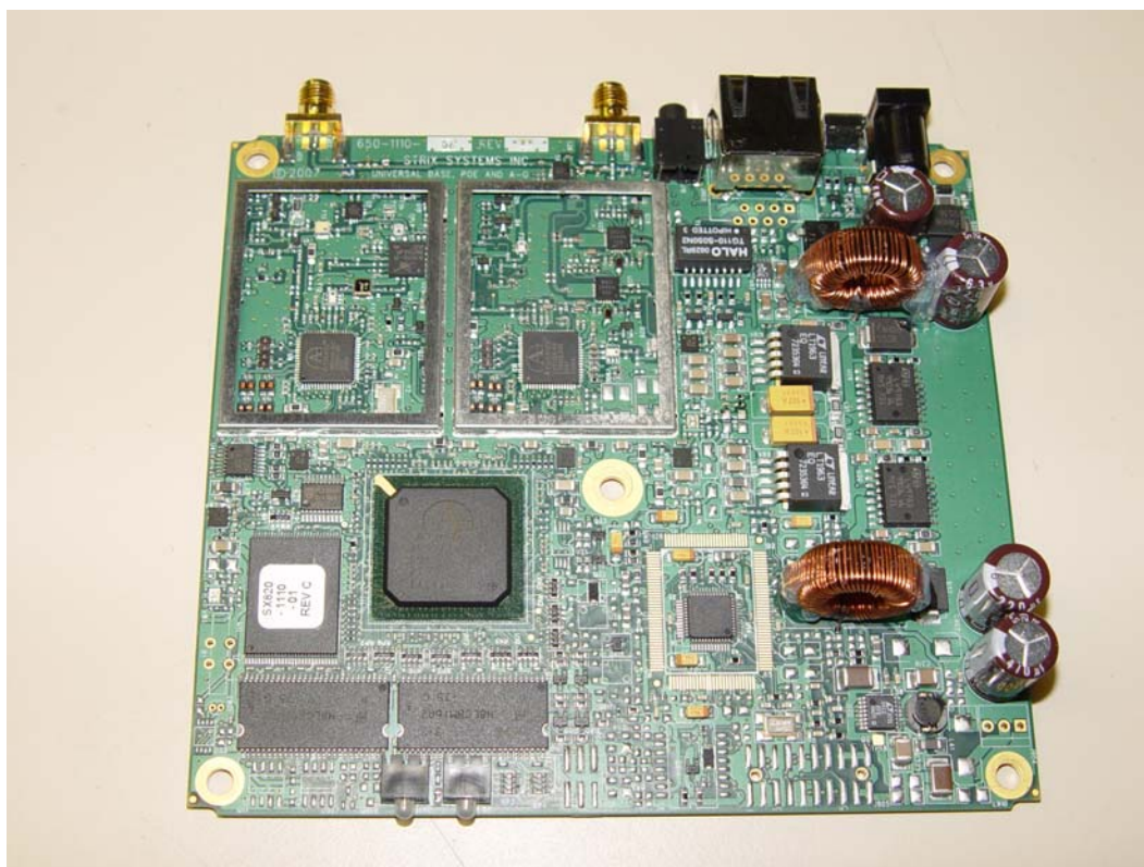
RF Assembly Top
