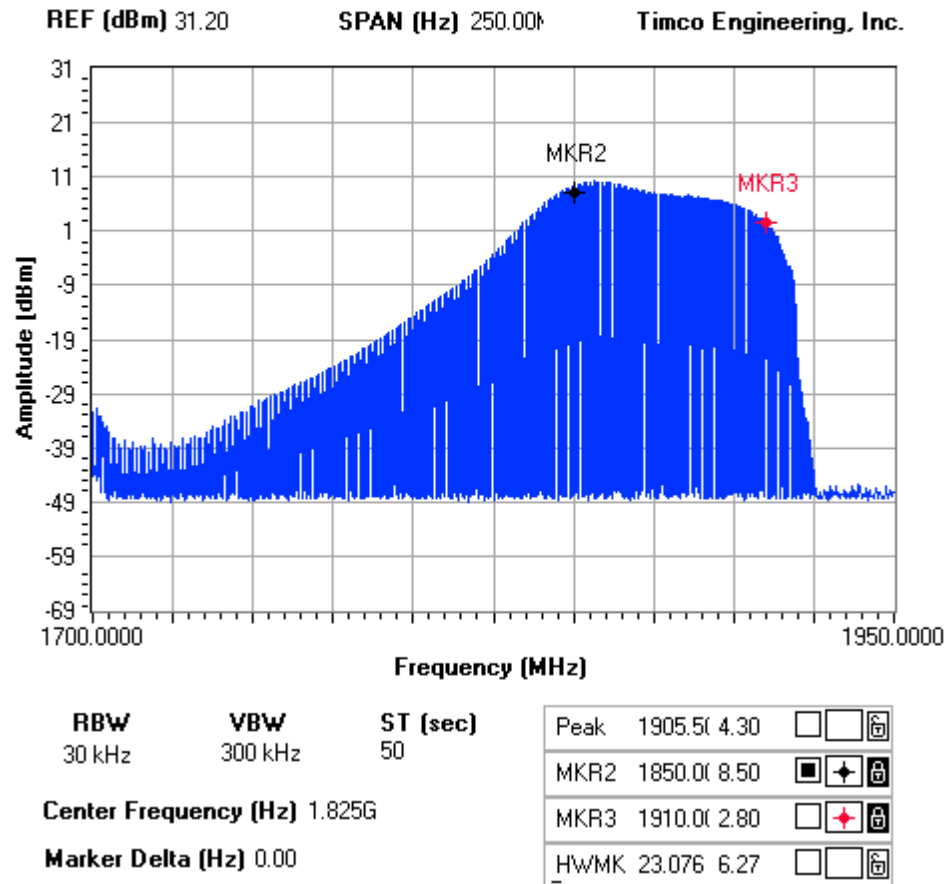
Figure 9. Filter frequency response PCS band
