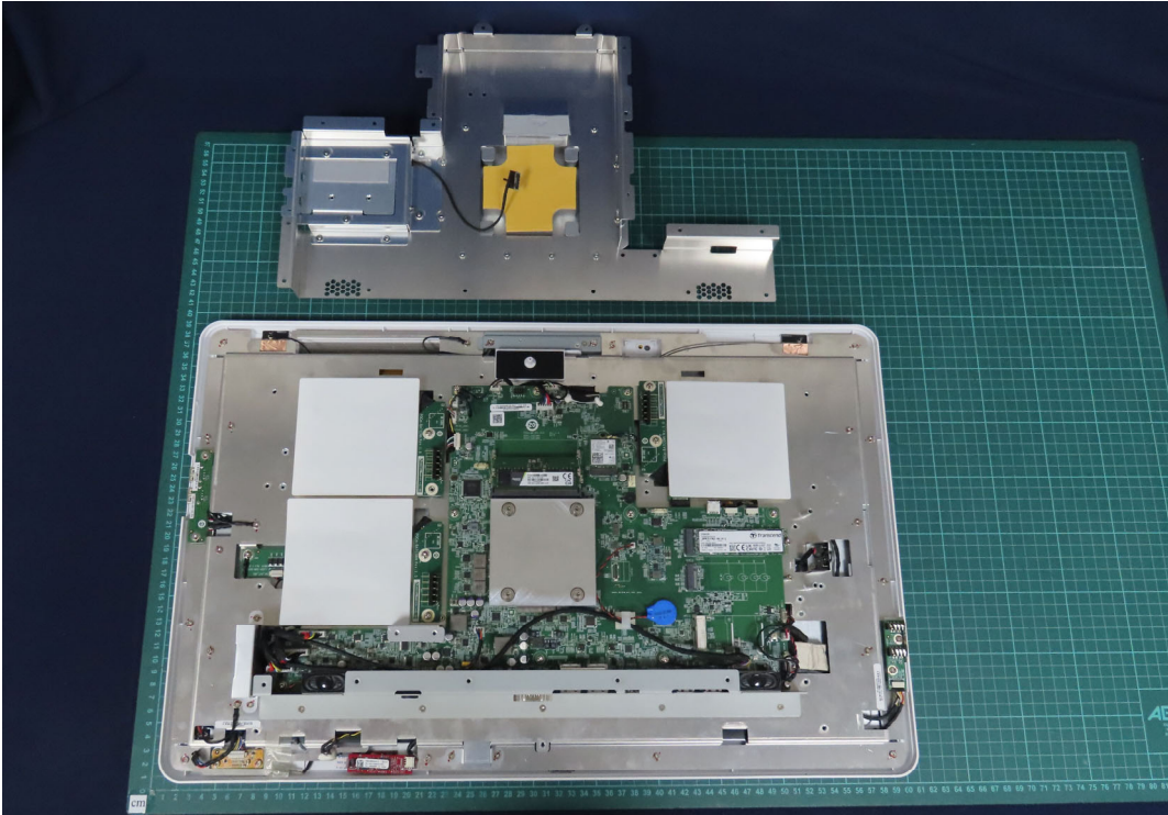
(7) EUT Photo
