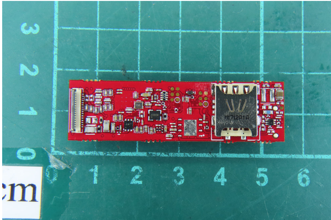
(39) EUT Photo
