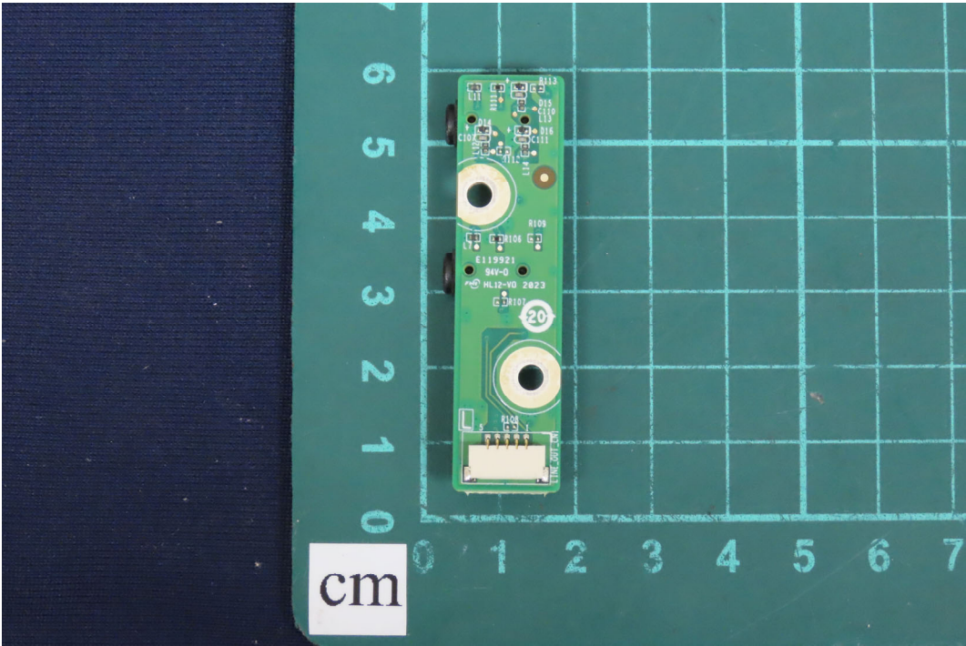
(27) EUT Photo
