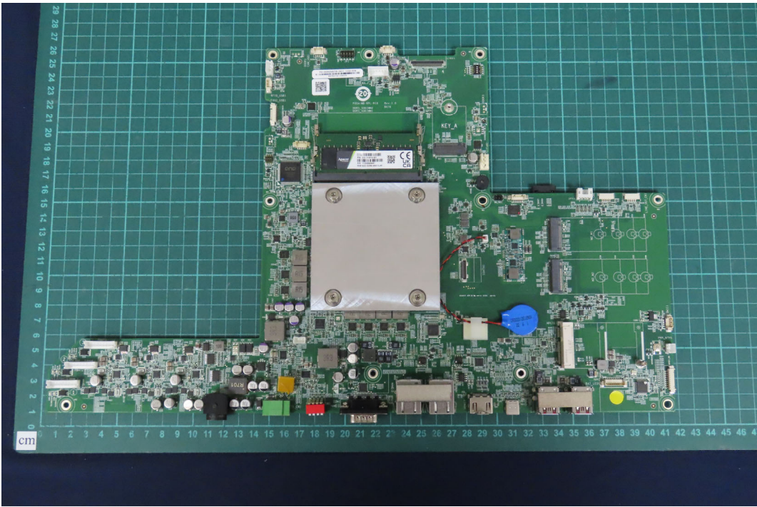
(28) EUT Photo
