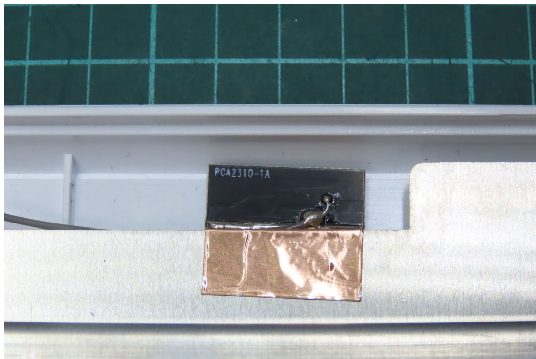
(34) EUT Photo
