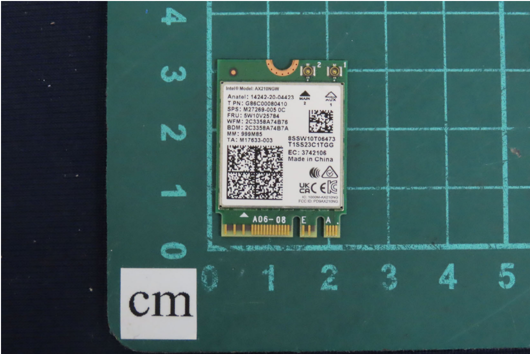
(92)EUT Photo
