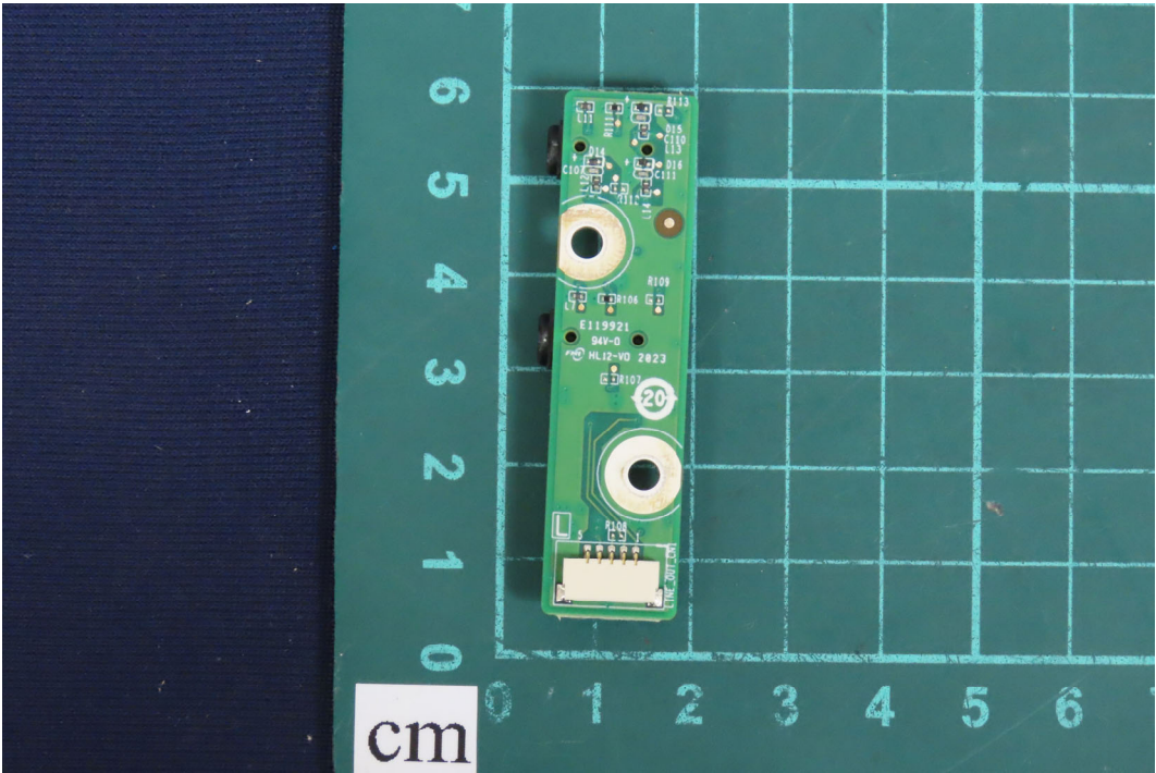
(109)EUT Photo
