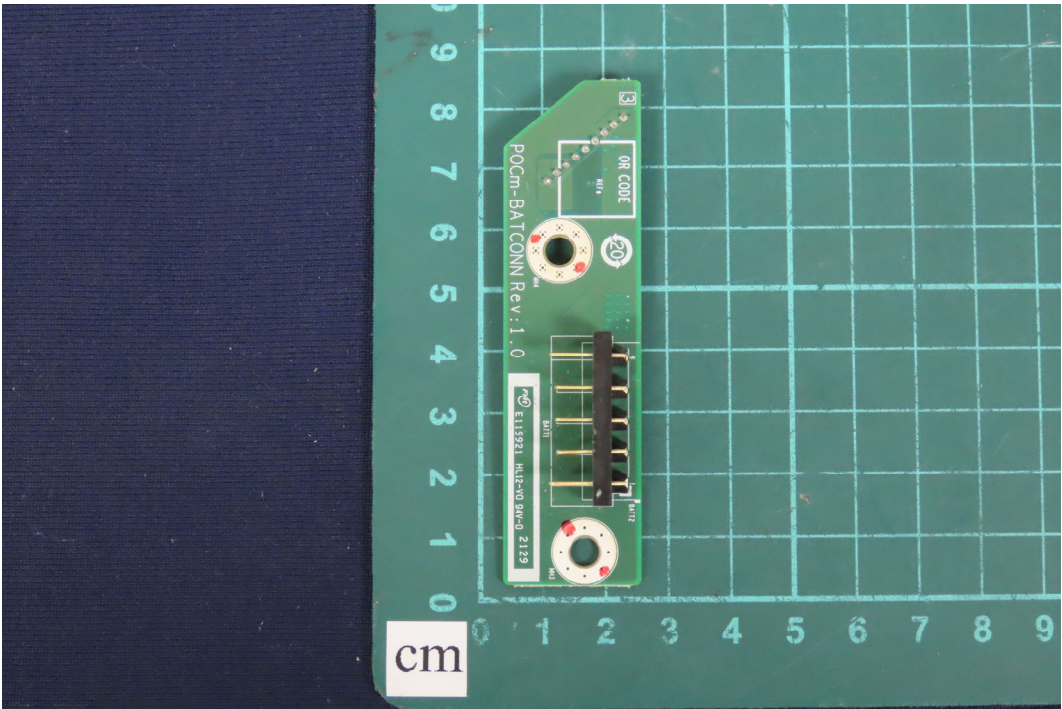
(102)EUT Photo
