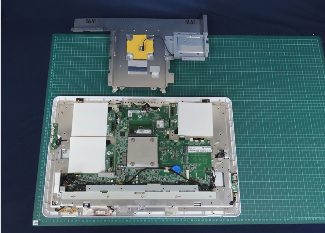
(89) EUT Photo
