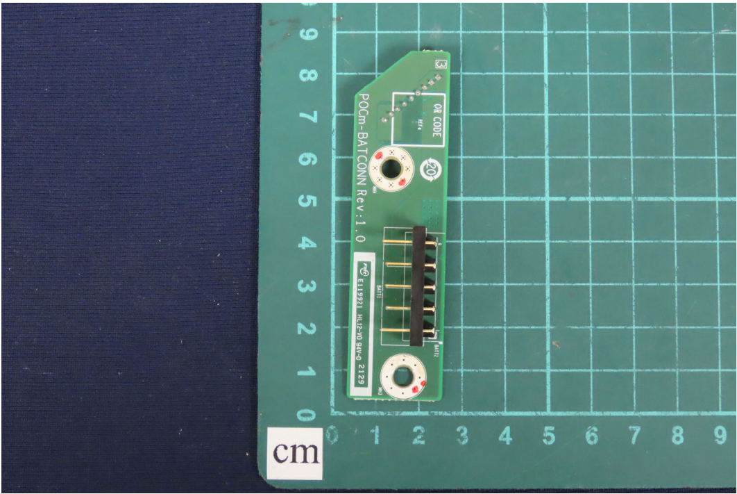
(100)EUT Photo
