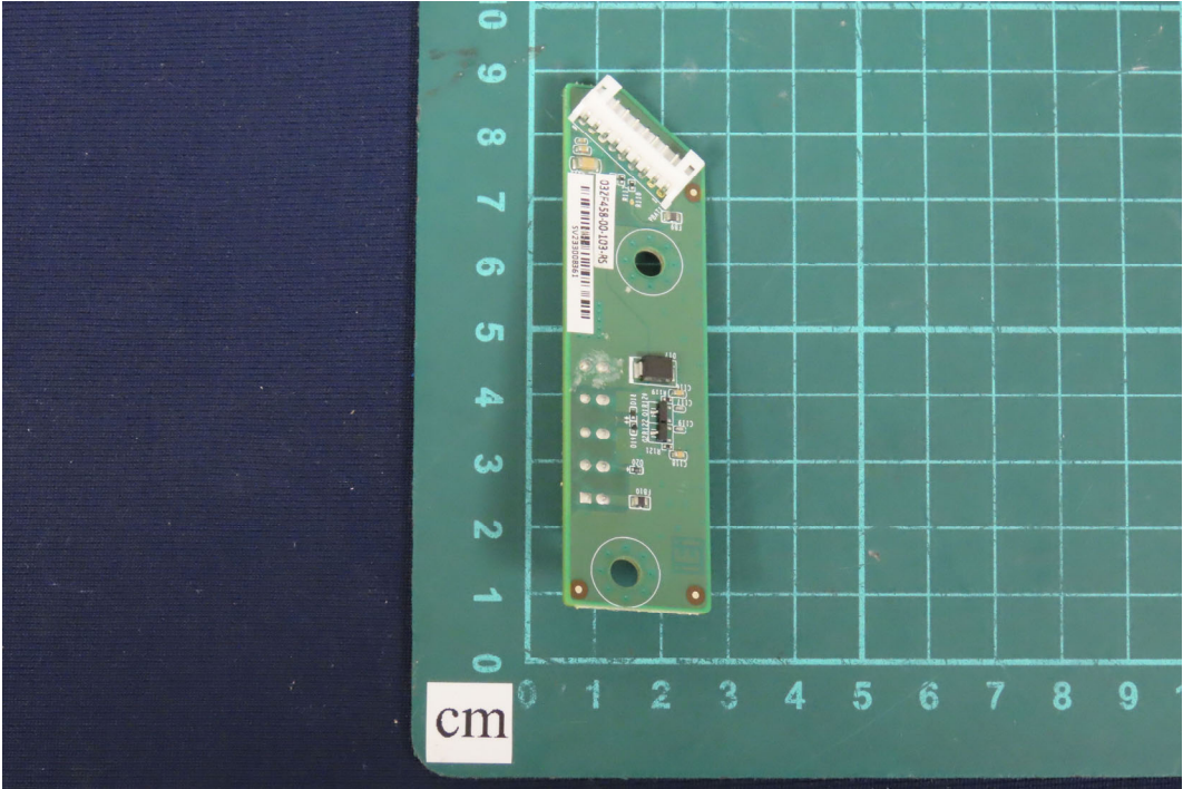
(103)EUT Photo
