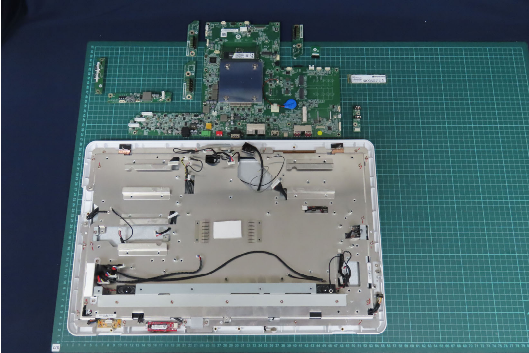
(95)EUT Photo
