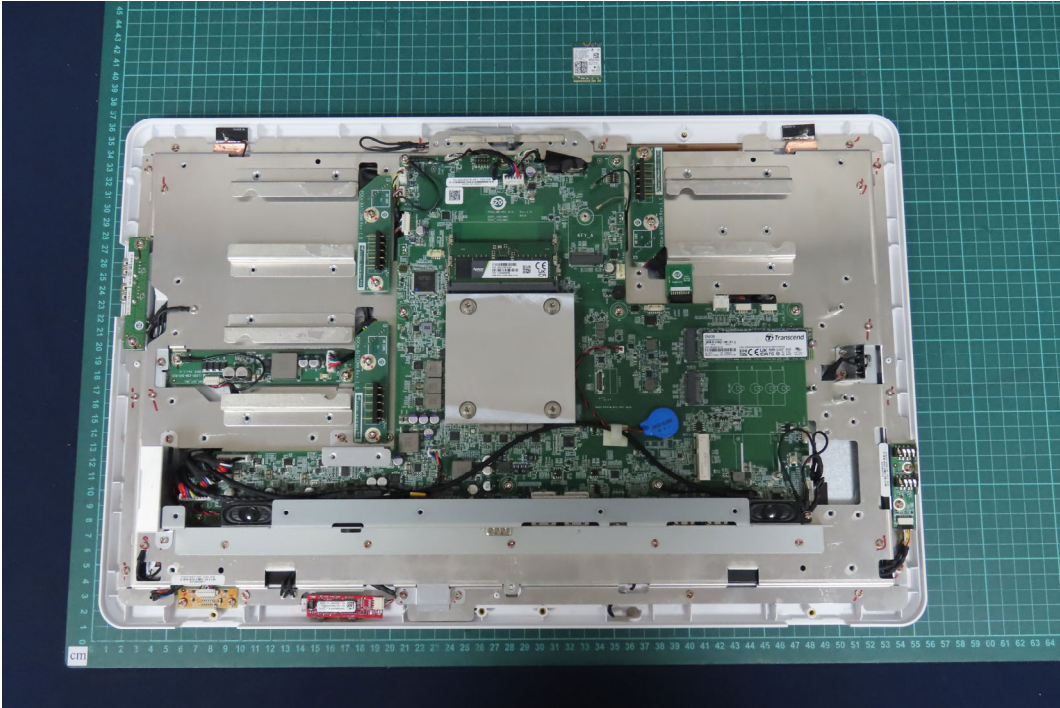
(91)EUT Photo
