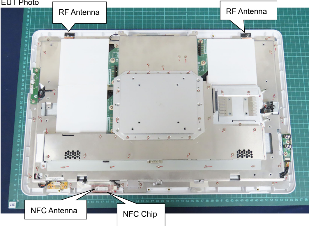
(129)EUT Photo
