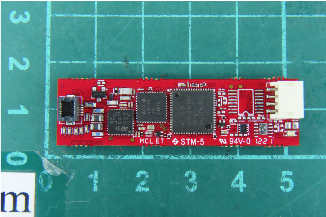
(161)EUT Photo
