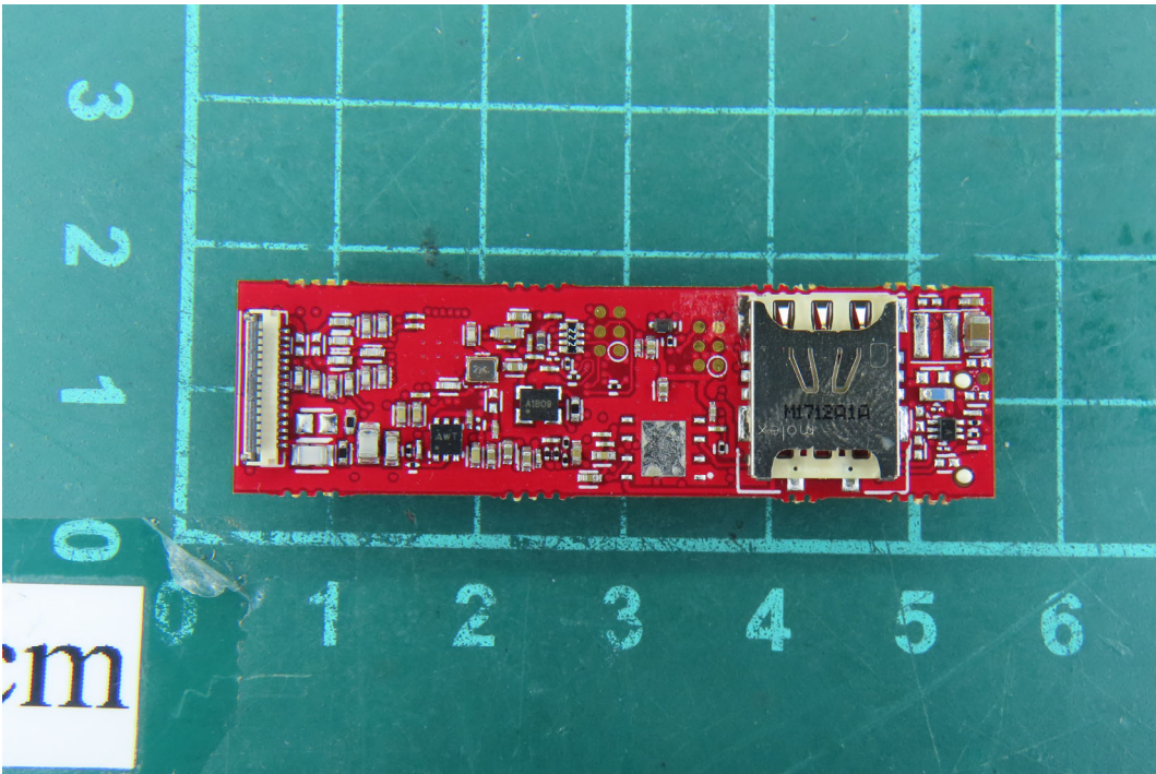
(162)EUT Photo
