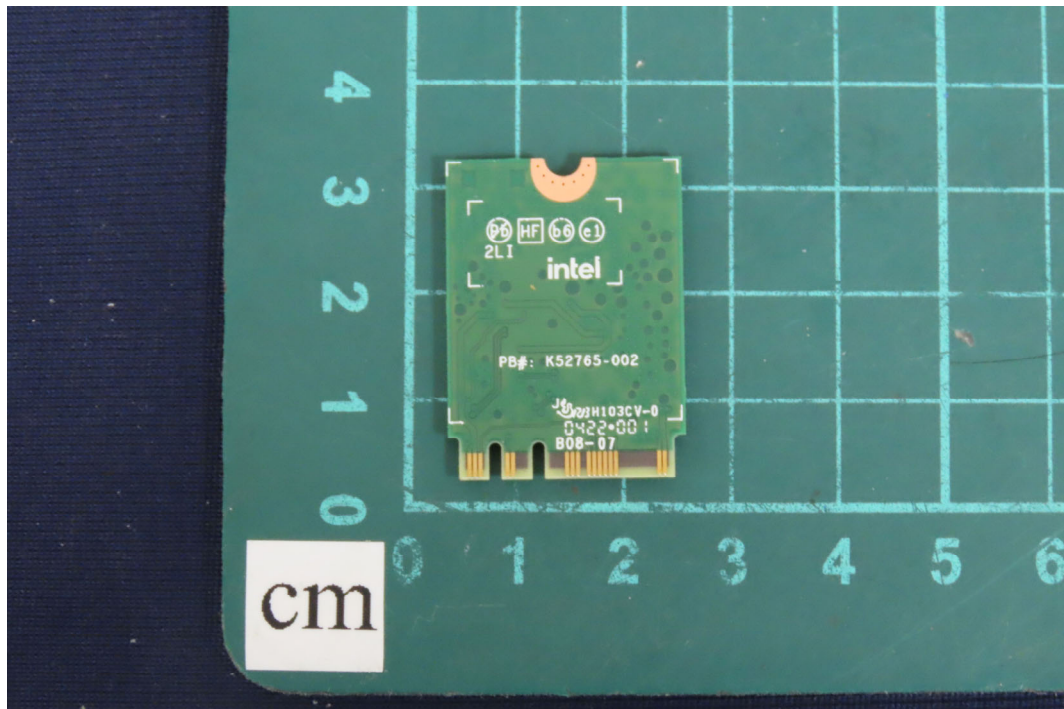
(43) EUT Photo
