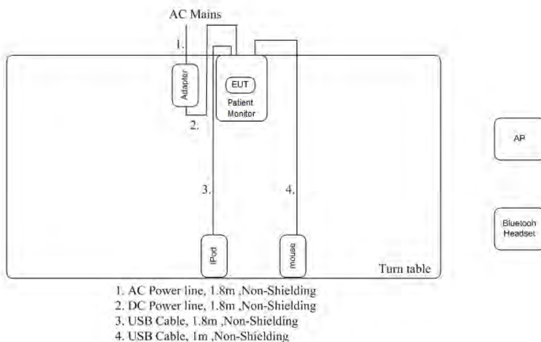
Test Setup Diagram –Radiated Test (below 1GHz)
