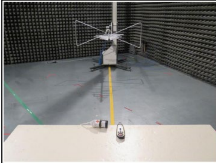
TEST SETUP 30 – 1000 MHz - CONFIGURATION 2
