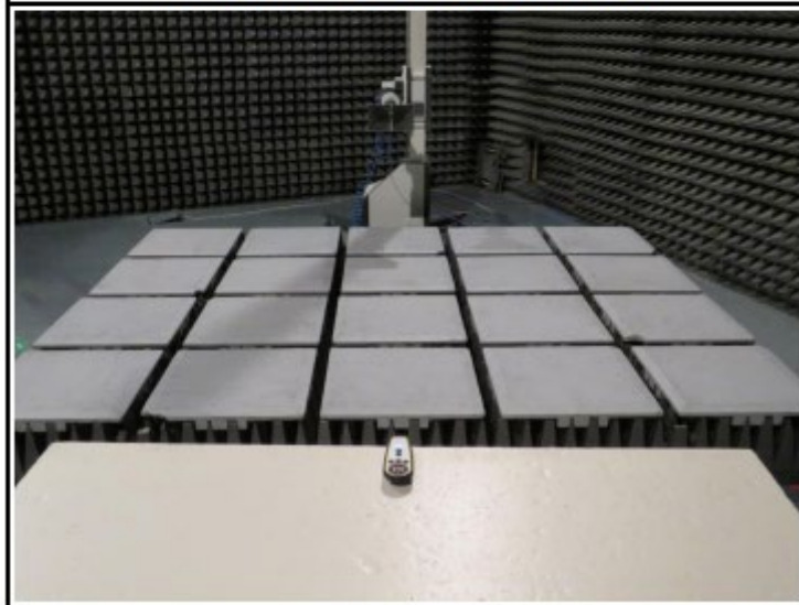
TEST SETUP 1 – 13 GHz - CONFIGURATION 1
