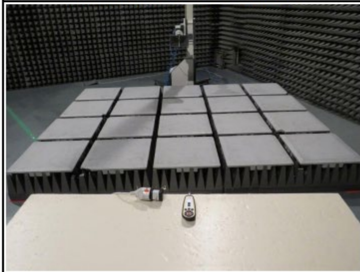
TEST SETUP 1 – 13 GHz - CONFIGURATION 2
