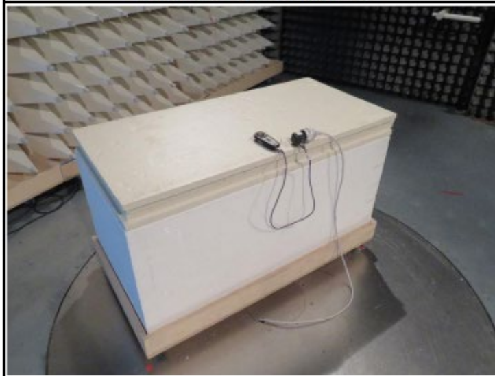
TEST SETUP – CONFIGURATION 2
