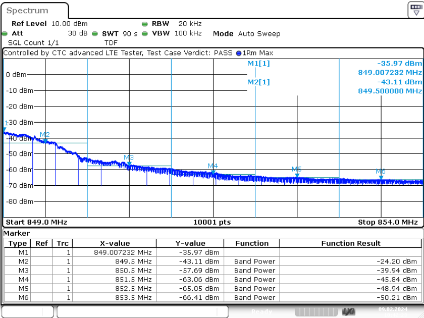
Plot 4: Highest channel – 16-QAM
