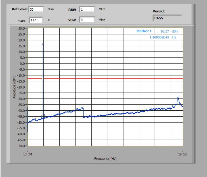
Plot 3: Highest Channel (10 MHz – 19.5 GHz)
