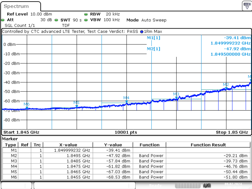
Plot 3: Lowest channel – 16-QAM
