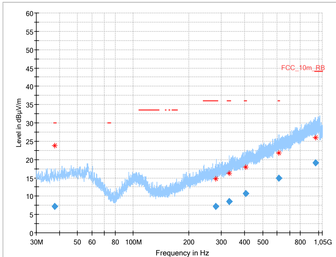
Plot 4: 30 MHz to 1 GHz, TX mode, vertical & horizontal polarization, 2 Msps, vvalid for all channels
