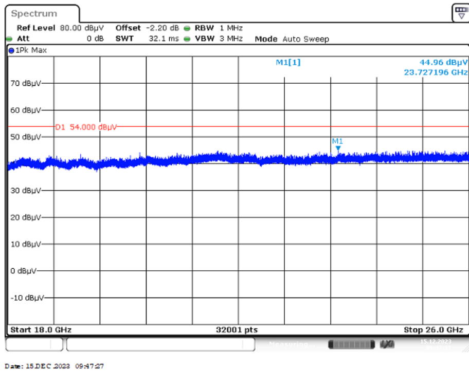
Plot 7: 18 GHz to 26 GHz, TX mode, 2478 MHz, vertical & horizontal polarization, 2 Msps
