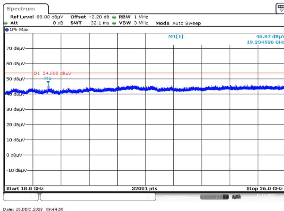
Plot 6: 18 GHz to 26 GHz, TX mode, vertical & horizontal polarization, valid for all channels
