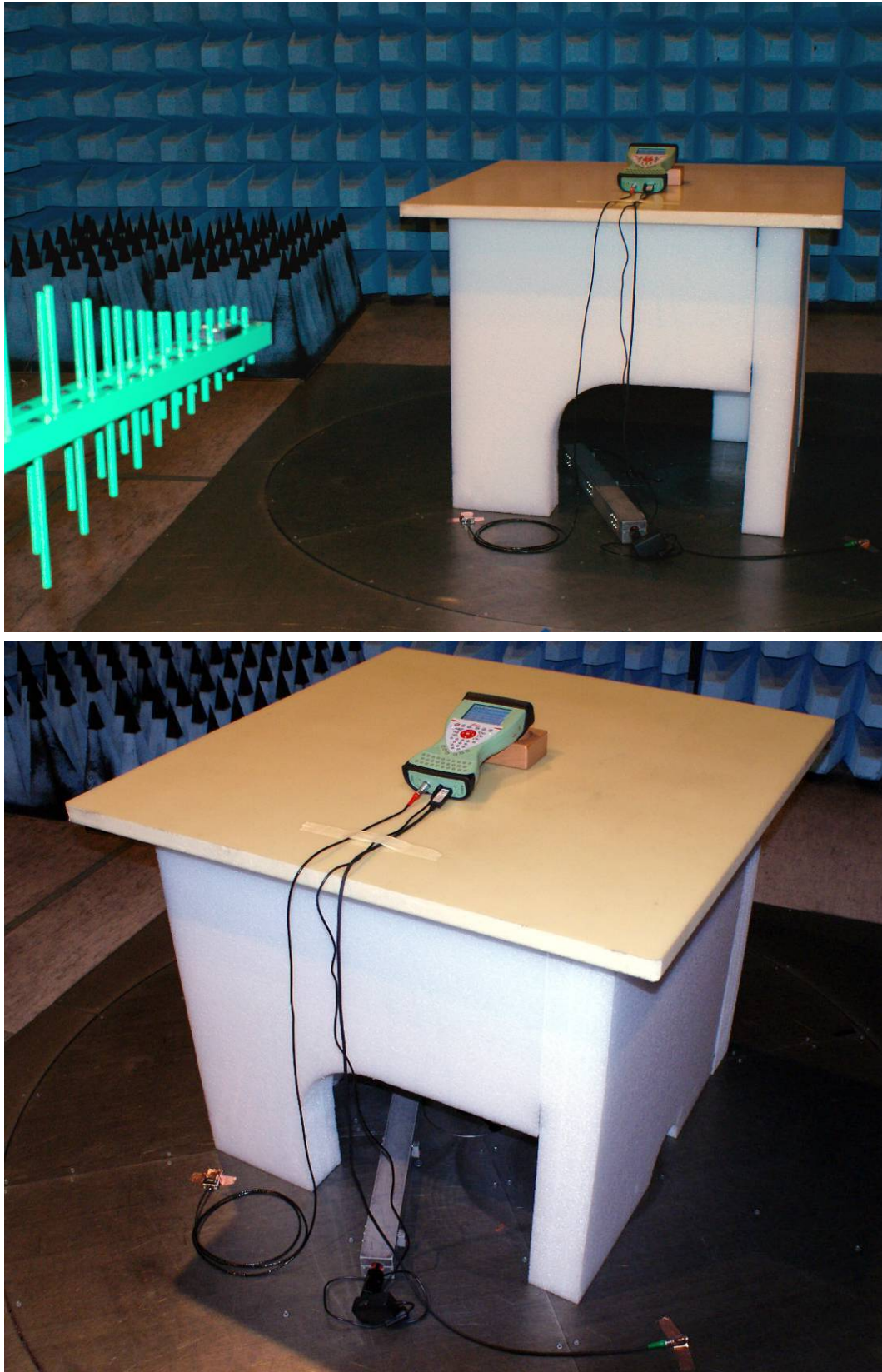
Photo 2: Measurement setup for radiated Emission
