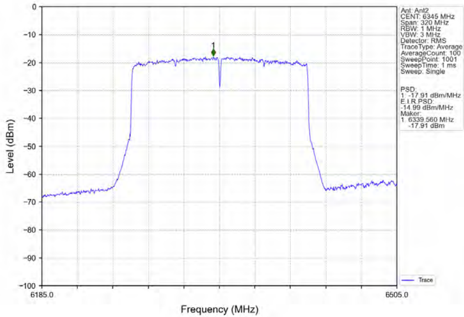
802.11ax(HEW160)_HCH_6345MHz_2xRU996_Left_MIMO_NTNV
