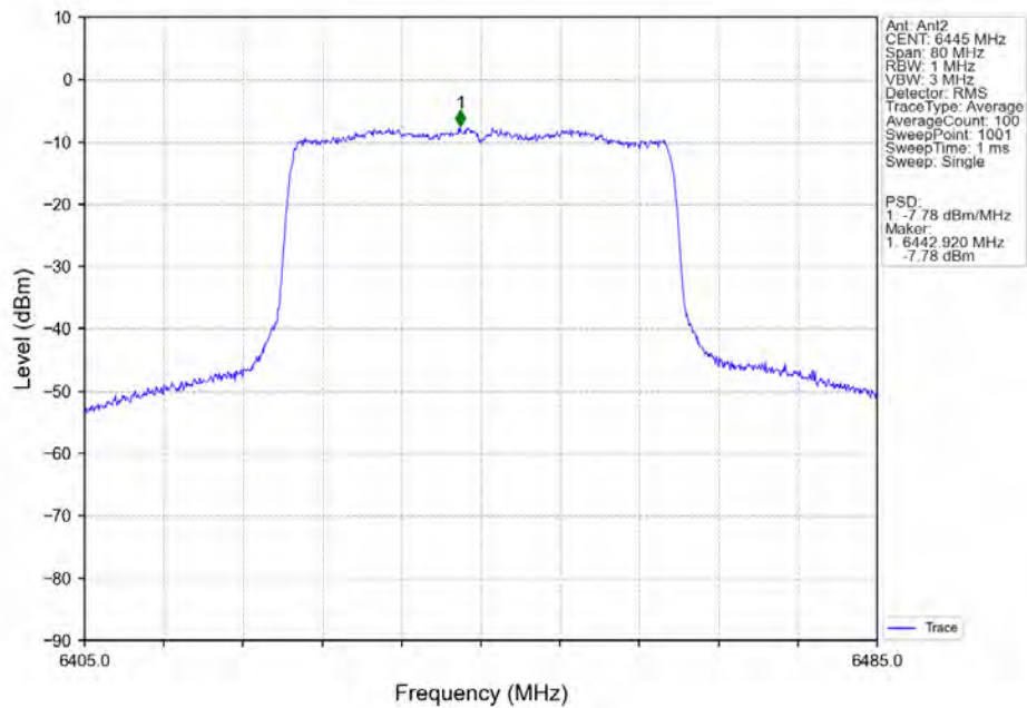
802.11ax(HEW40)_LCH_6445MHz_RU484_Left_MIMO_NTNV
