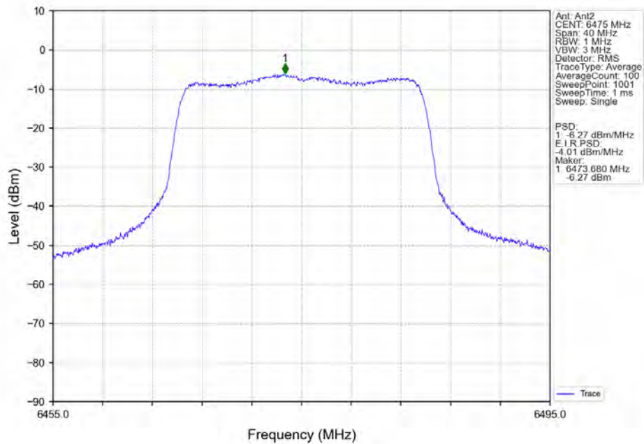
802.11ax(HEW20)_MCH_6475MHz_RU242_Left_MIMO_NTNV
