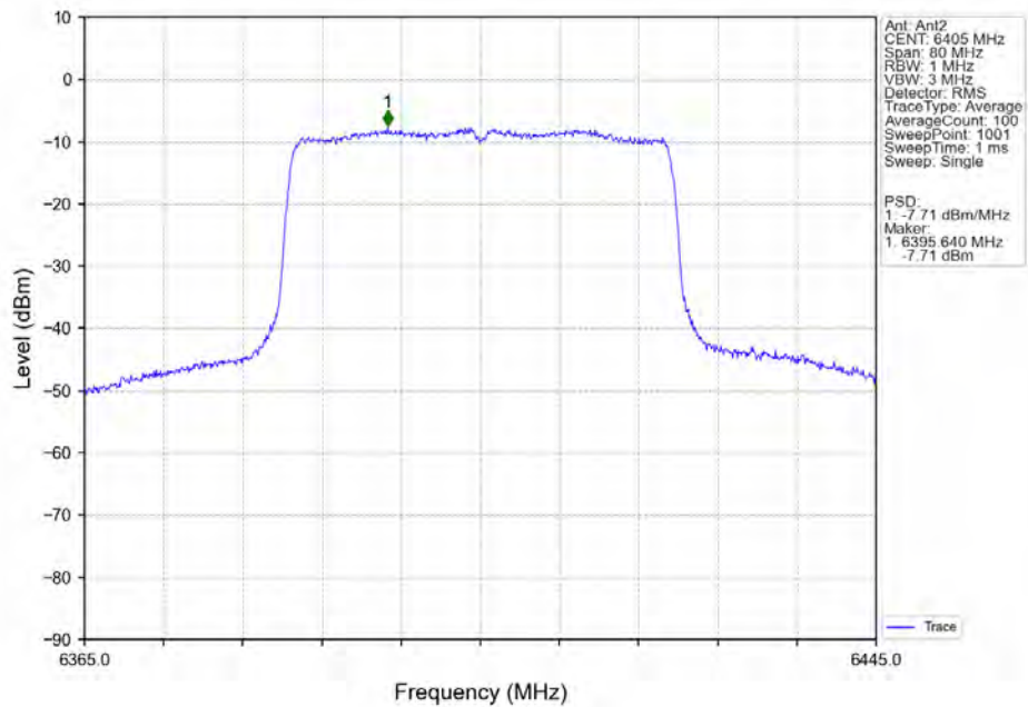
802.11ax(HEW40)_HCH_6405MHz_RU484_Left_MIMO_NTNV
