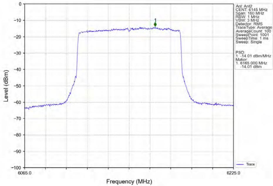
802.11ax(HEW80)_MCH_6145MHz_RU996_Left_MIMO_NTNV
