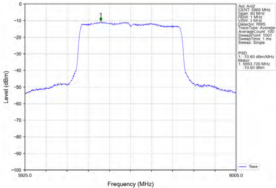
802.11ax(HEW40)_LCH_5965MHz_RU484_Left_MIMO_NTNV
