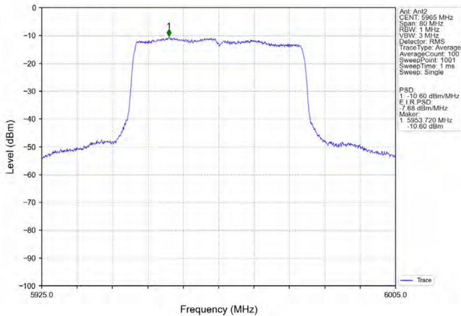
802.11ax(HEW40)_LCH_5965MHz_RU484_Left_MIMO_NTNV
