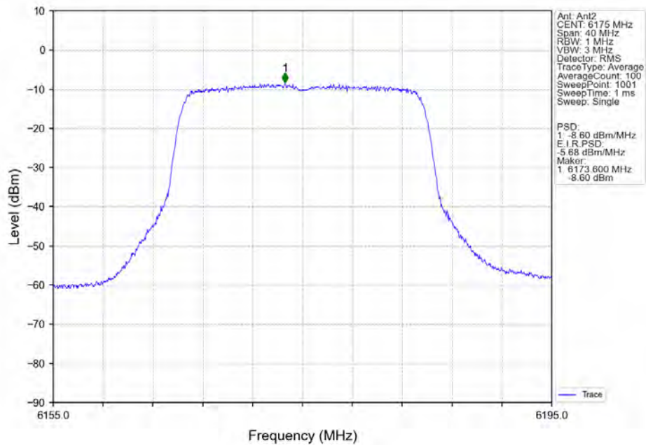
802.11ax(HEW20)_MCH_6175MHz_RU242_Left_MIMO_NTNV
