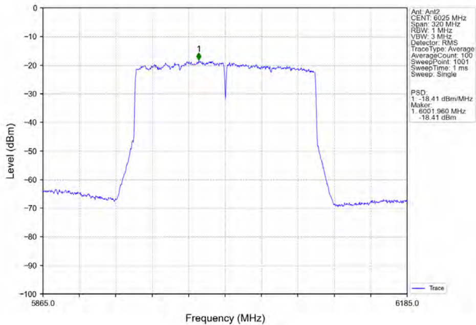
802.11ax(HEW160)_LCH_6025MHz_2xRU996_Left_MIMO_NTNV
