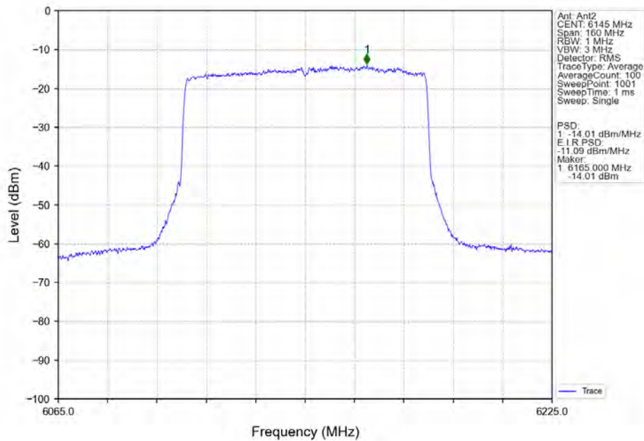
802.11ax(HEW80)_MCH_6145MHz_RU996_Left_MIMO_NTNV
