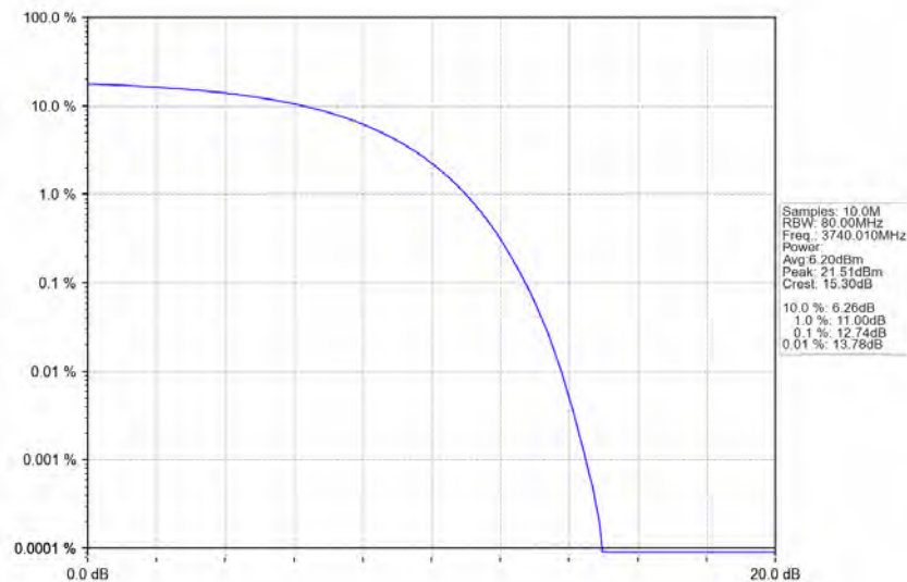
n77a 30kHz SISO NTN 80MHz CP-OFDM 64 QAM 3740.01MHz Outer Full Ant1
