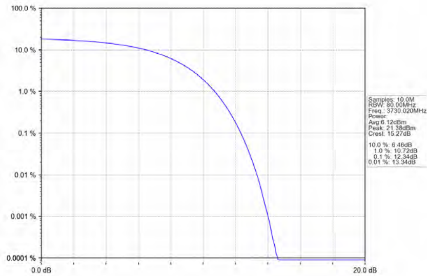
n77a_30kHz_SISO_NTNV_60MHz_CP-OFDM_64_QAM_3730.02MHz_Outer_Full_Ant1
