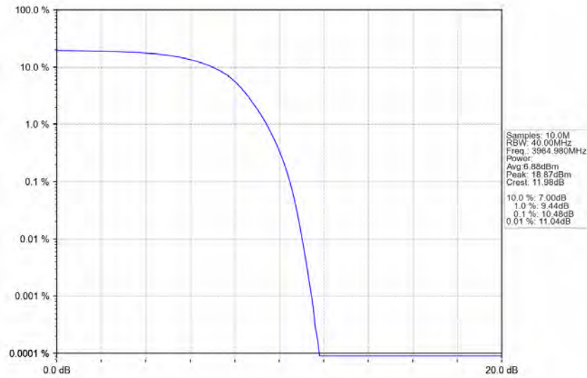
n77a_30kHz_SISO_NTNV_30MHz_DFT-s-OFDM_64_QAM_3964.98MHz_Outer_Full_Ant1
