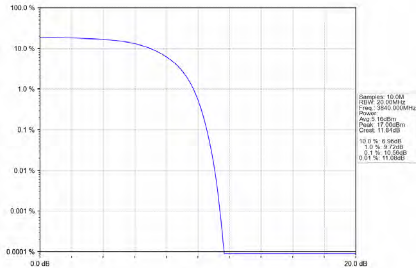
n77a_30kHz_SISO_NTNV_20MHz_CP-OFDM_16_QAM_3840MHz_Outer_Full_Ant1
