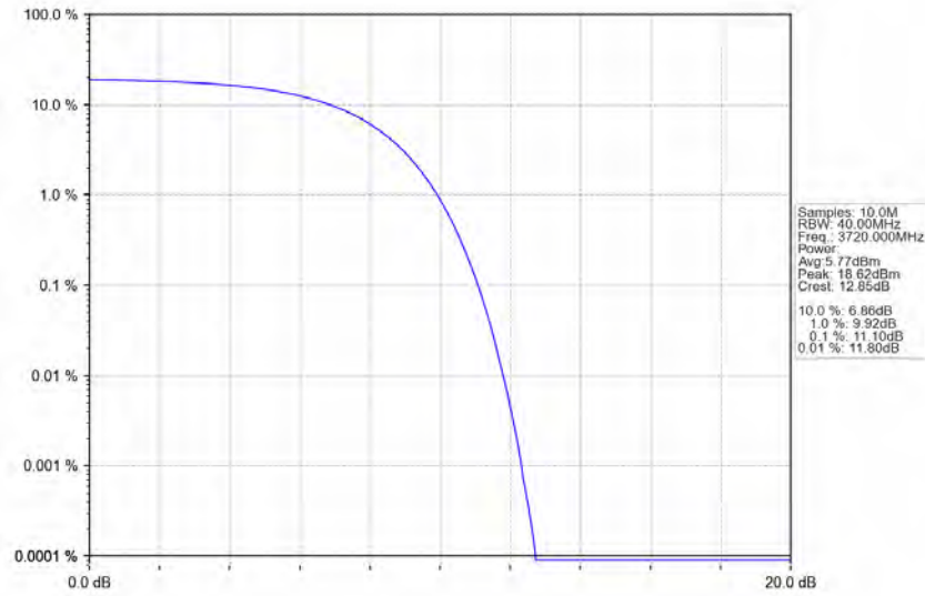
n77a_30kHz_SISO_NTNV_40MHz_CP-OFDM_16_QAM_3720MHz_Outer_Full_Ant1
