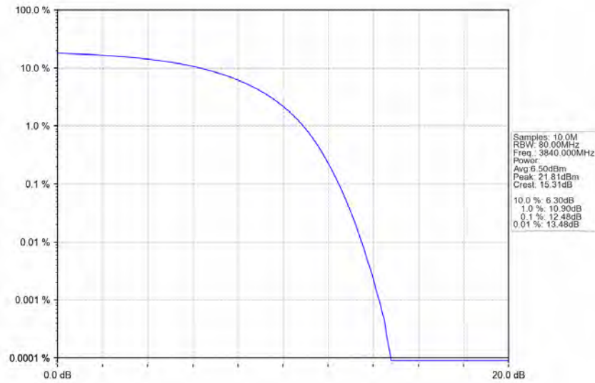
n77a_30kHz_SISO_NTNV_80MHz_DFT-s-OFDM_256_QAM_3840MHz_Outer_Full_Ant1
