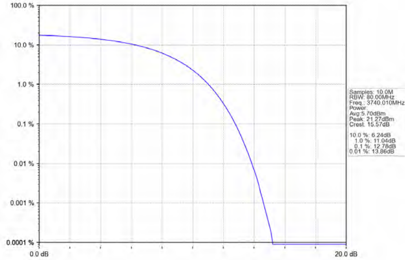
n77a 30kHz SISO NTN 80MHz CP-OFDM 256 QAM 3740.01MHz Outer Full Ant1
