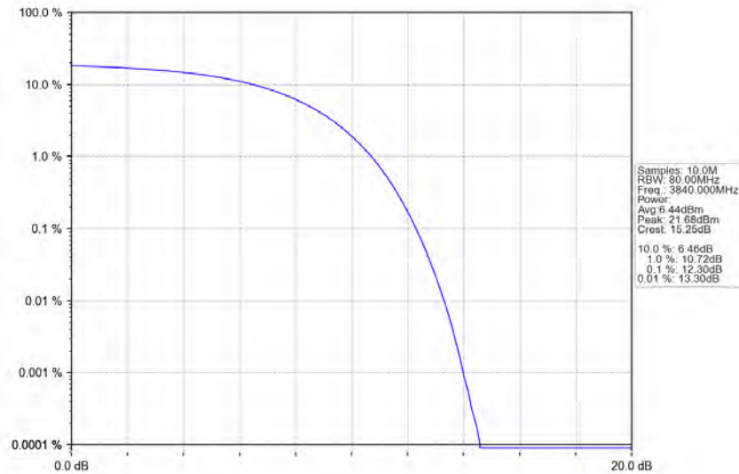
n77a_30kHz_SISO_NTNV_60MHz_CP-OFDM_16_QAM_3840MHz_Outer_Full_Ant1
