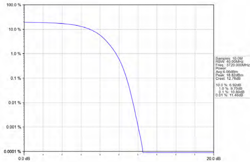
n77a_30kHz_SISO_NTNV_40MHz_DFT-s-OFDM_64_QAM_3720MHz_Outer_Full_Ant1
