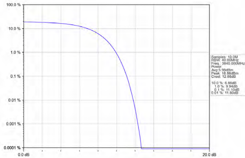
n77a_30kHz_SISO_NTNV_40MHz_CP-OFDM_16_QAM_3840MHz_Outer_Full_Ant1
