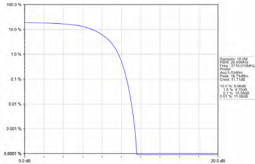
n77a_30kHz_SISO_NTNV_20MHz_CP-OFDM_16_QAM_3710.01MHz_Outer_Full_Ant1
