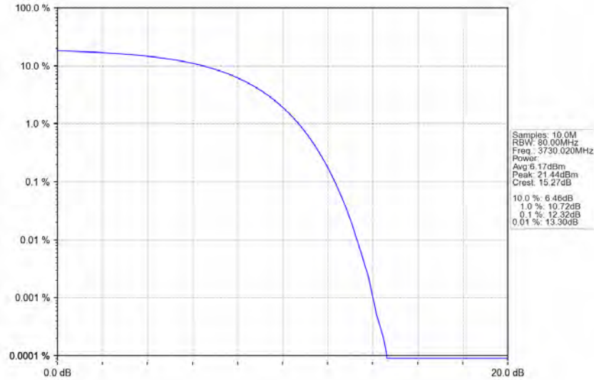
n77a_30kHz_SISO_NTNV_60MHz_CP-OFDM_16_QAM_3730.02MHz_Outer_Full_Ant1
