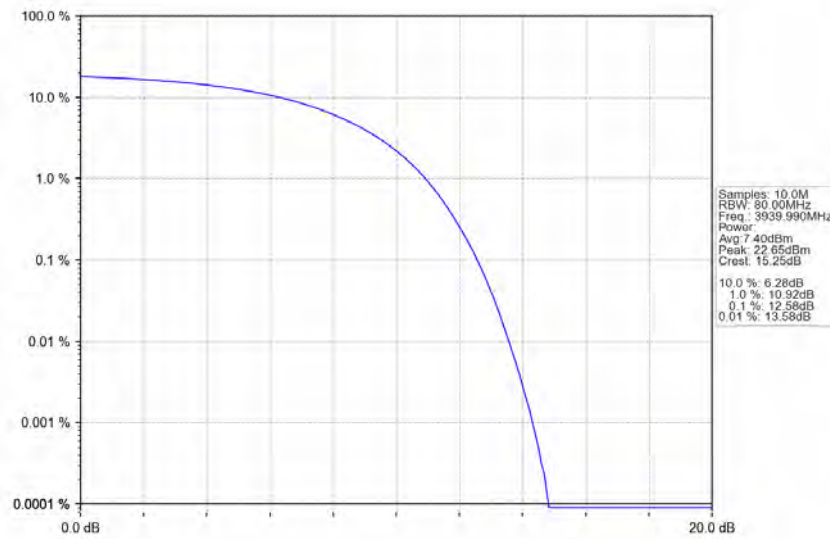
n77a_30kHz_SISO_NTNV_80MHz_DFT-s-OFDM_64_QAM_3939.99MHz_Outer_Full_Ant1
