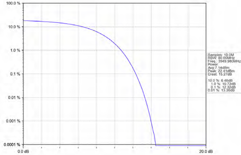
n77a_30kHz_SISO_NTNV_60MHz_CP-OFDM_16_QAM_3949.98MHz_Outer_Full_Ant1
