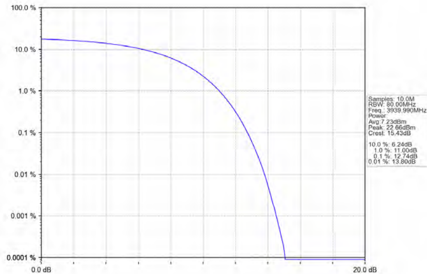
n77a 30kHz SISO NTN 80MHz CP-OFDM 16 QAM 3939.99MHz Outer Full Ant1
