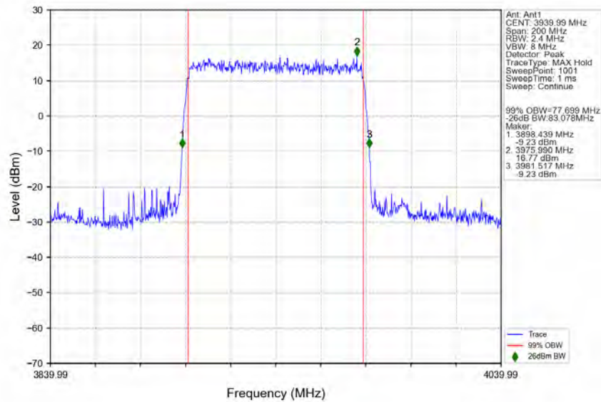
n77a 30kHz SISO NTN 80MHz DFT-s-OFDM QPSK 3939.99MHz Outer Full Ant1
