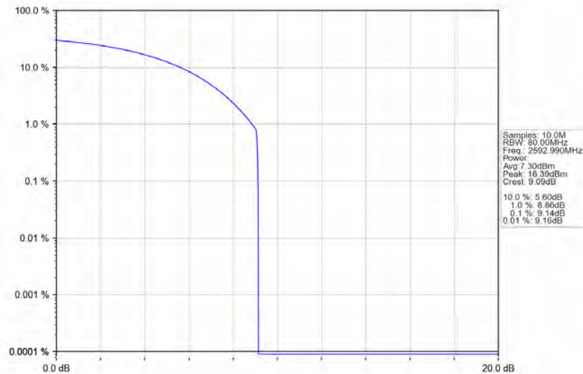
n41_30kHz_SISO_NTNV_80MHz_CP-OFDM_QPSK_2592.99MHz_Outer_Full_Ant1
