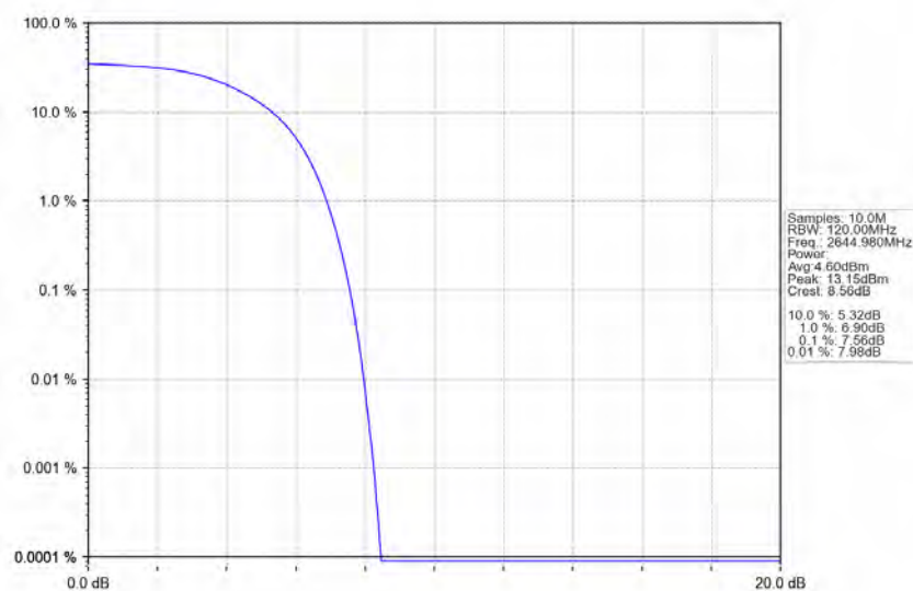
n41_30kHz_SISO_NTNV_90MHz_CP-OFDM_64_QAM_2644.98MHz_Outer_Full_Ant1
