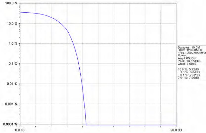
n41_30kHz_SISO_NTNV_100MHz_CP-OFDM_QPSK_2592.99MHz_Outer_Full_Ant1
