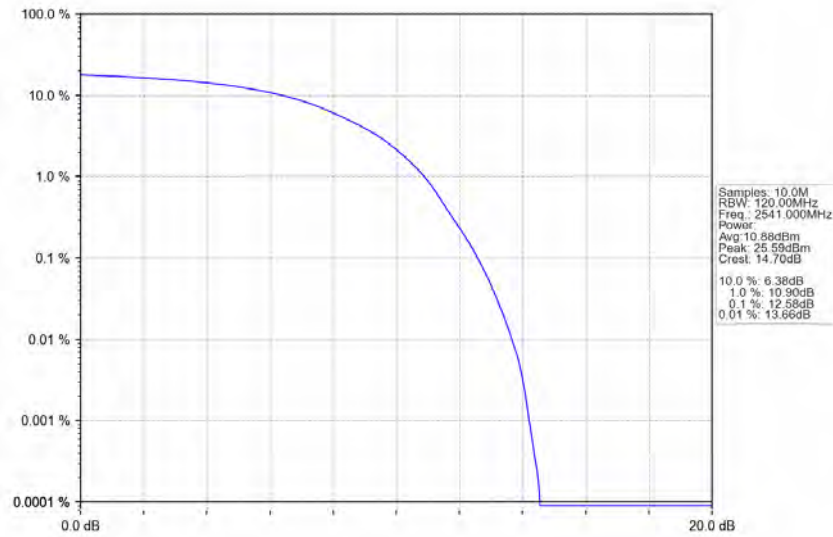
n41_30kHz_SISO_NTNV_90MHz_DFT-s-OFDM_64_QAM_2541MHz_Outer_Full_Ant1
