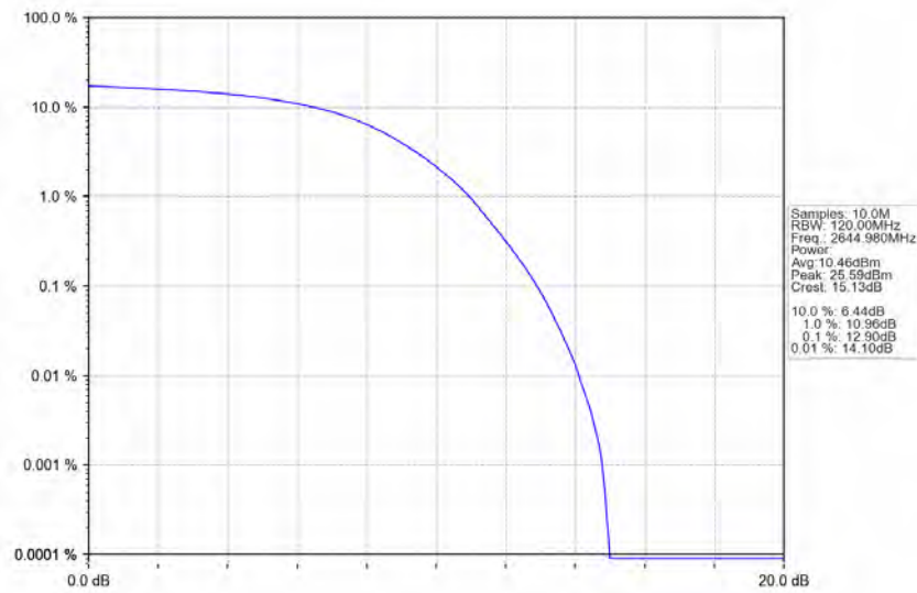
n41_30kHz_SISO_NTNV_90MHz_DFT-s-OFDM_64_QAM_2644.98MHz_Outer_Full_Ant1
