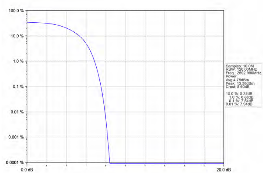
n41_30kHz_SISO_NTNV_90MHz_CP-OFDM_QPSK_2592.99MHz_Outer_Full_Ant1
