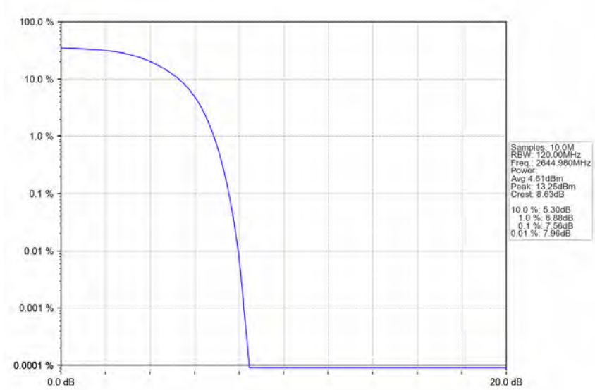
n41_30kHz_SISO_NTNV_90MHz_CP-OFDM_QPSK_2644.98MHz_Outer_Full_Ant1
