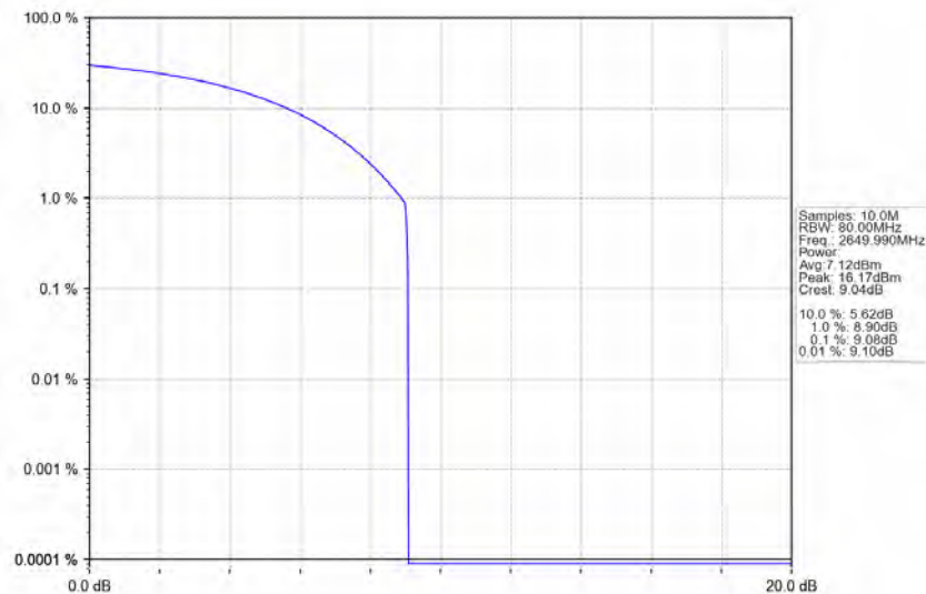
n41_30kHz_SISO_NTNV_80MHz_CP-OFDM_QPSK_2649.99MHz_Outer_Full_Ant1
