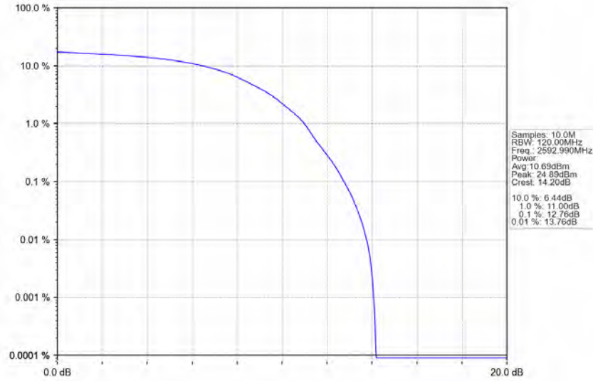
n41_30kHz_SISO_NTNV_90MHz_DFT-s-OFDM_64_QAM_2592.99MHz_Outer_Full_Ant1
