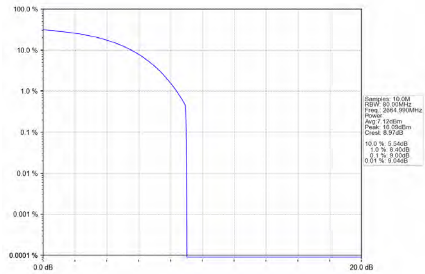
n41_30kHz_SISO_NTNV_50MHz_CP-OFDM_QPSK_2664.99MHz_Outer_Full_Ant1
