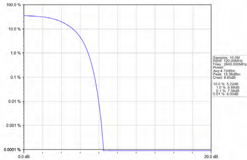
n41_30kHz_SISO_NTNV_100MHz_CP-OFDM_QPSK_2640MHz_Outer_Full_Ant1
