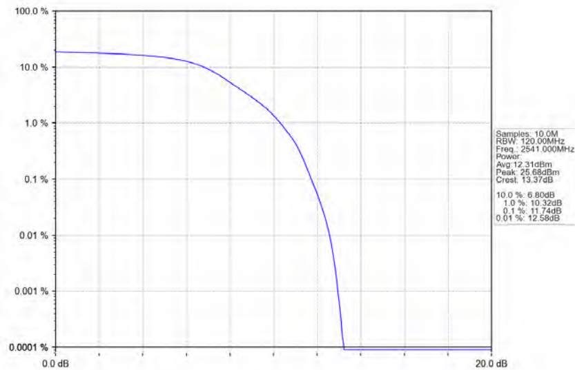
n41_30kHz_SISO_NTNV_90MHz_DFT-s-OFDM_QPSK_2541MHz_Outer_Full_Ant1
