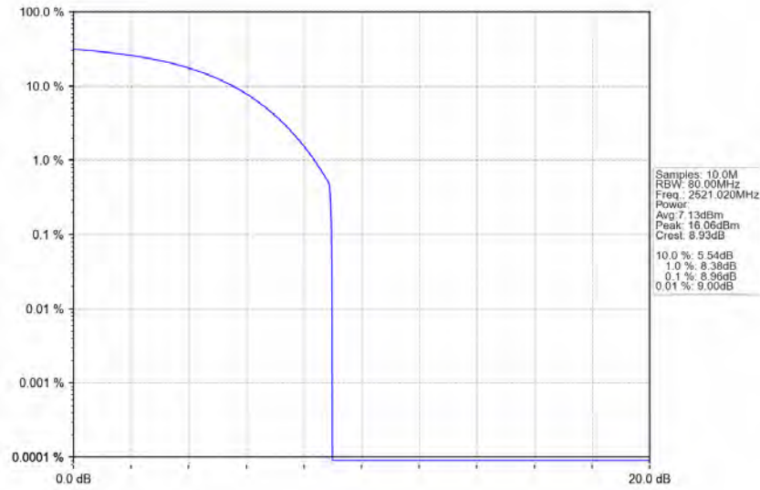
n41_30kHz_SISO_NTNV_50MHz_CP-OFDM_16QAM_2521.02MHz_Outer_Full_Ant1
