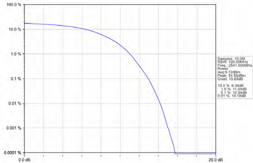
n41_30kHz_SISO_NTNV_90MHz_DFT-s-OFDM_256_QAM_2541MHz_Outer_Full_Ant1
