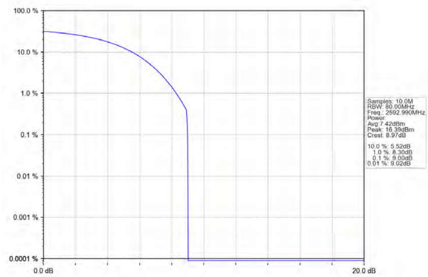
n41_30kHz_SISO_NTNV_50MHz_CP-OFDM_QPSK_2592.99MHz_Outer_Full_Ant1
