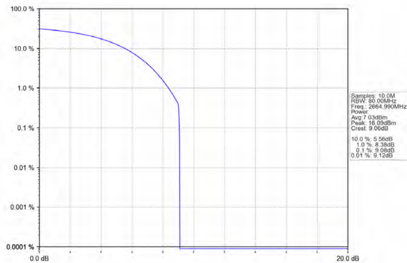
n41_30kHz_SISO_NTNV_50MHz_CP-OFDM_64_QAM_2664.99MHz_Outer_Full_Ant1
