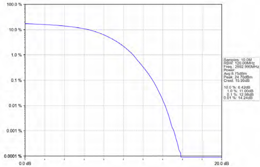
n41_30kHz_SISO_NTNV_90MHz_DFT-s-OFDM_256_QAM_2592.99MHz_Outer_Full_Ant1
