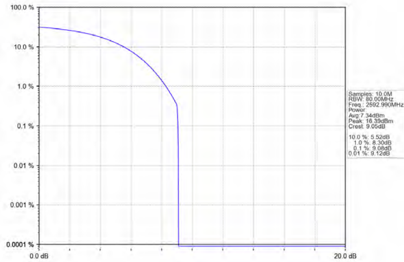
n41_30kHz_SISO_NTNV_50MHz_CP-OFDM_64_QAM_2592.99MHz_Outer_Full_Ant1
