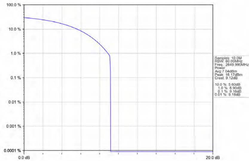
n41_30kHz_SISO_NTNV_80MHz_CP-OFDM_64_QAM_2649.99MHz_Outer_Full_Ant1
