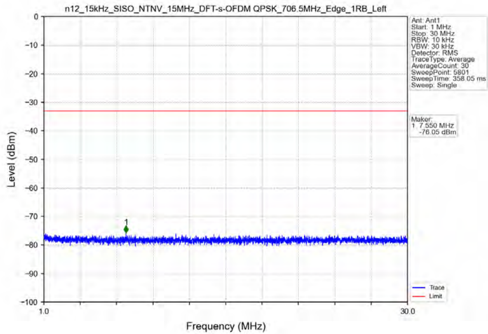
n12_15kHz_SISO_NTNV_15MHz_DFT-s-OFDM_QPSK_706.5MHz_Edge_1RB_Left
