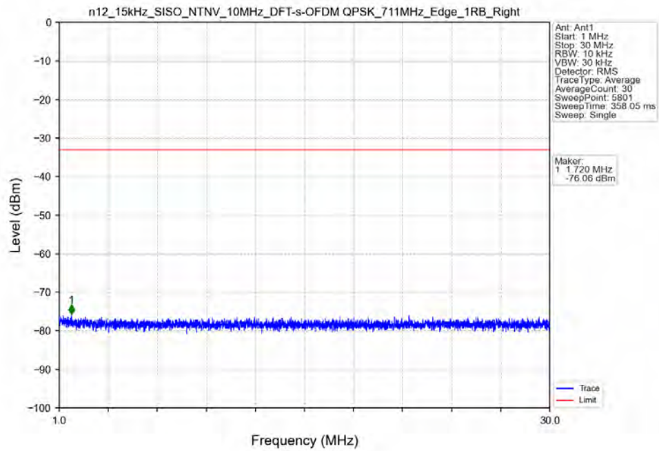
n12_15kHz_SISO_NTNV_10MHz_DFT-s-OFDM_QPSK_711MHz_Edge_1RB_Right
