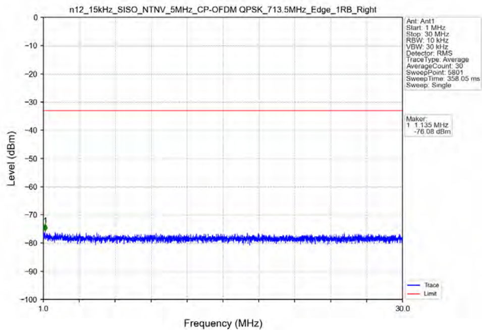
n12_15kHz_SISO_NTNV_5MHz_CP-OFDM QPSK_713.5MHz_Edge_1RB_Right
