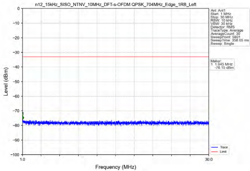
n12_15kHz_SISO_NTNV_10MHz_DFT-s-OFDM_QPSK_704MHz_Edge_1RB_Left
