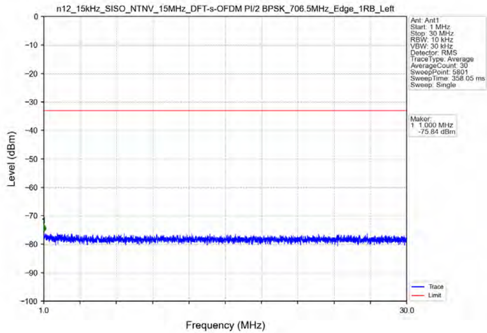
n12_15kHz_SISO_NTNV_15MHz_DFT-s-OFDM_PI/2_BPSK_706.5MHz_Edge_1RB_Left
