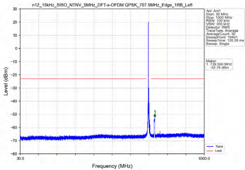
n12_15kHz_SISO_NTNV_5MHz_DFT-s-OFDM_QPSK_707.5MHz_Edge_1RB_Left
