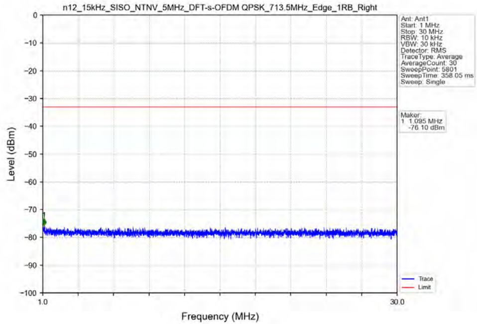
n12_15kHz_SISO_NTNV_5MHz_DFT-s-OFDM_QPSK_713.5MHz_Edge_1RB_Right
