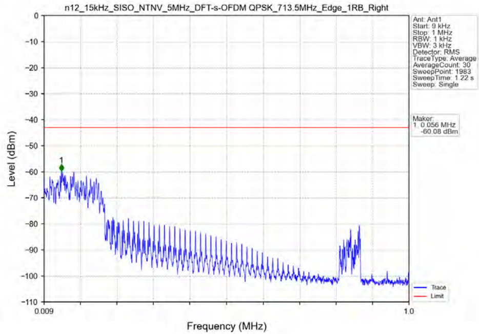
n12_15kHz_SISO_NTNV_5MHz_DFT-s-OFDM_QPSK_713.5MHz_Edge_1RB_Right
