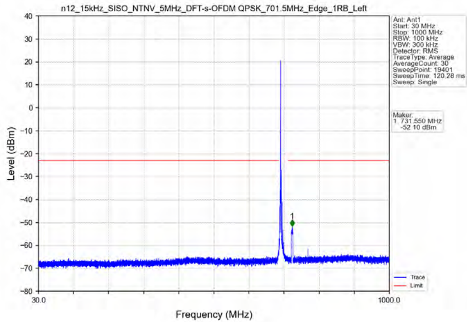
n12_15kHz_SISO_NTNV_5MHz_DFT-s-OFDM_QPSK_701.5MHz_Edge_1RB_Left
