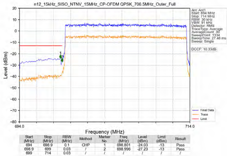
n12_15kHz_SISO_NTNV_15MHz_CP-OFDM_QPSK_706.5MHz_Outer_Full
