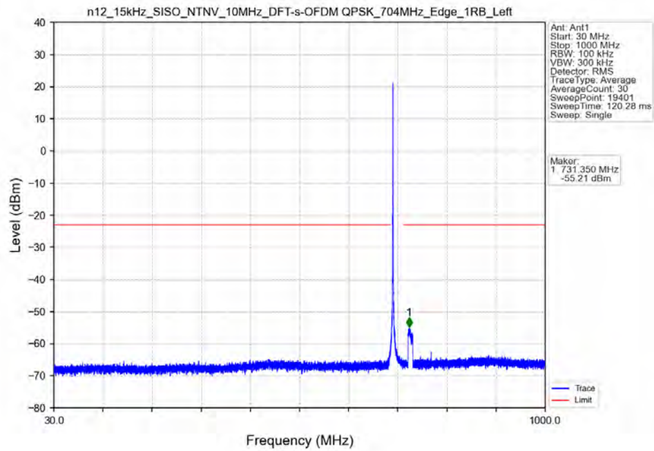
n12_15kHz_SISO_NTNV_10MHz_DFT-s-OFDM_QPSK_704MHz_Edge_1RB_Left
