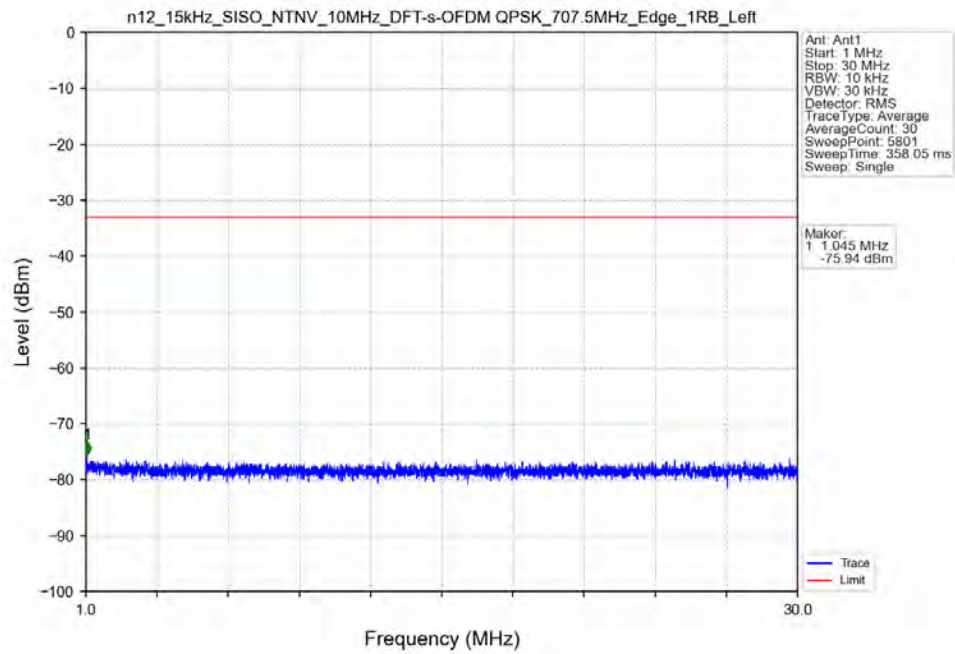
n12_15kHz_SISO_NTNV_10MHz_DFT-s-OFDM_QPSK_707.5MHz_Edge_1RB_Left
