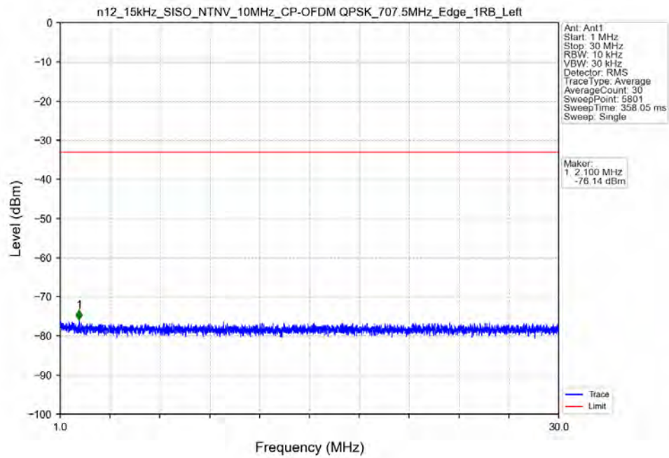
n12_15kHz_SISO_NTNV_10MHz_CP-OFDM_QPSK_707.5MHz_Edge_1RB_Left
