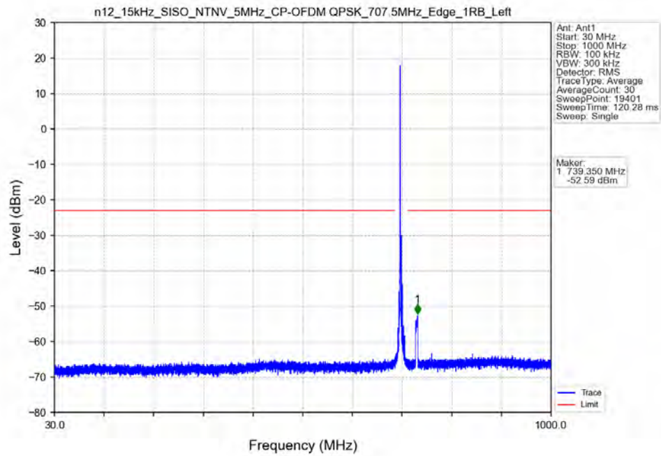
n12_15kHz_SISO_NTNV_5MHz_CP-OFDM_QPSK_707.5MHz_Edge_1RB_Left
