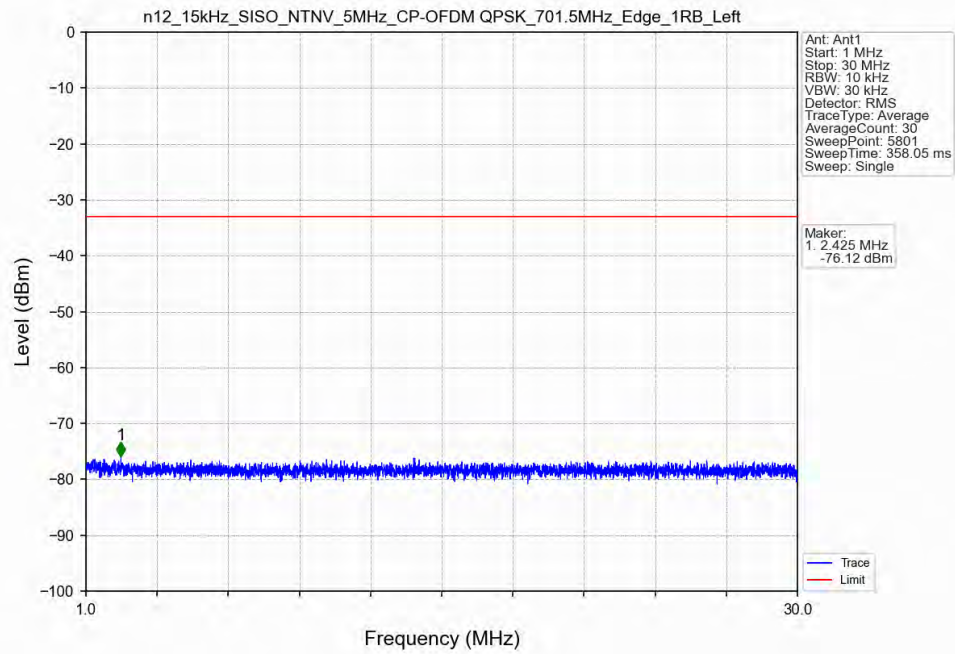
n12_15kHz_SISO_NTNV_5MHz_CP-OFDM_QPSK_701.5MHz_Edge_1RB_Left
