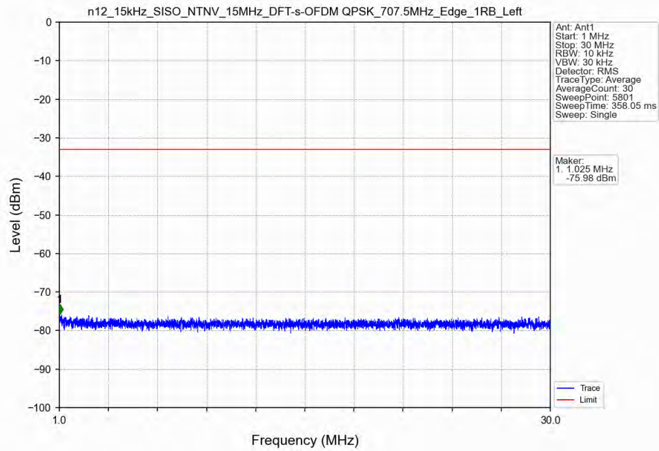
n12_15kHz_SISO_NTNV_15MHz_DFT-s-OFDM_QPSK_707.5MHz_Edge_1RB_Left
