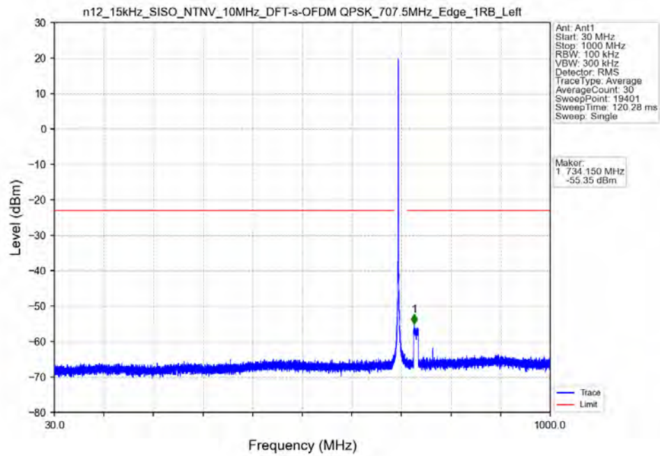
n12_15kHz_SISO_NTNV_10MHz_DFT-s-OFDM_QPSK_707.5MHz_Edge_1RB_Left
