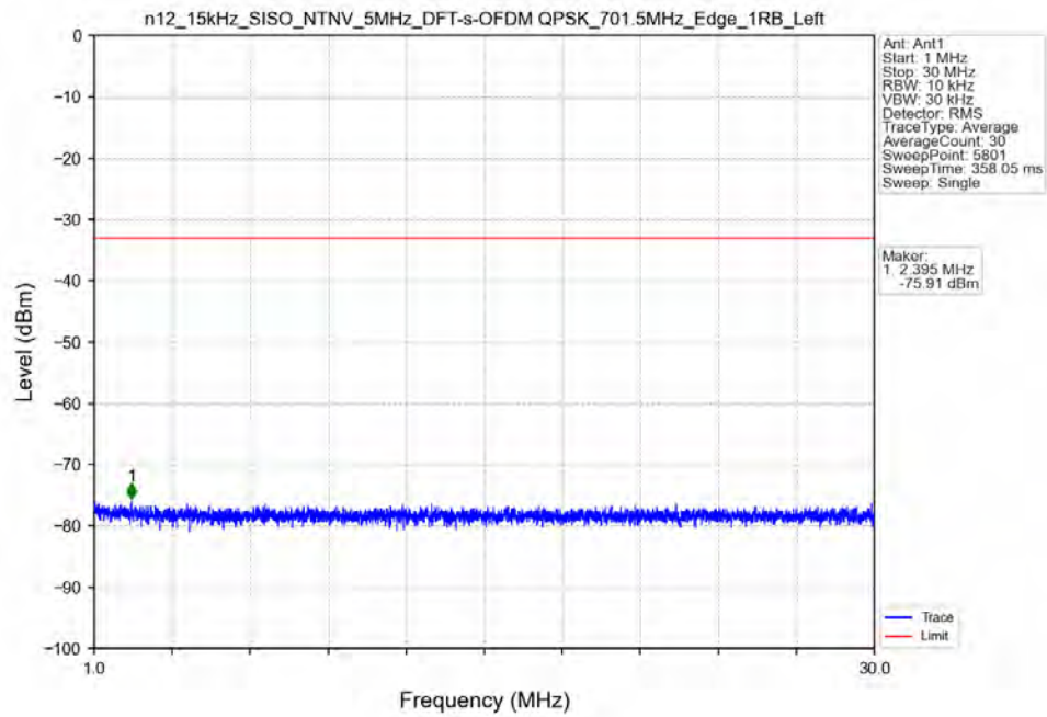
n12_15kHz_SISO_NTNV_5MHz_DFT-s-OFDM_QPSK_701.5MHz_Edge_1RB_Left
