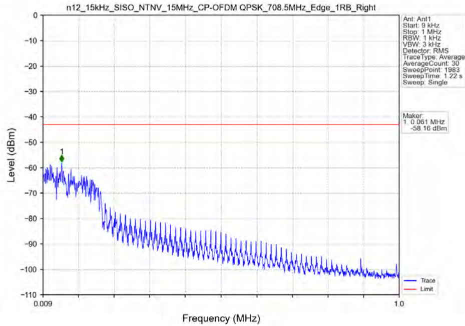
n12_15kHz_SISO_NTNV_15MHz_CP-OFDM_QPSK_708.5MHz_Edge_1RB_Right
