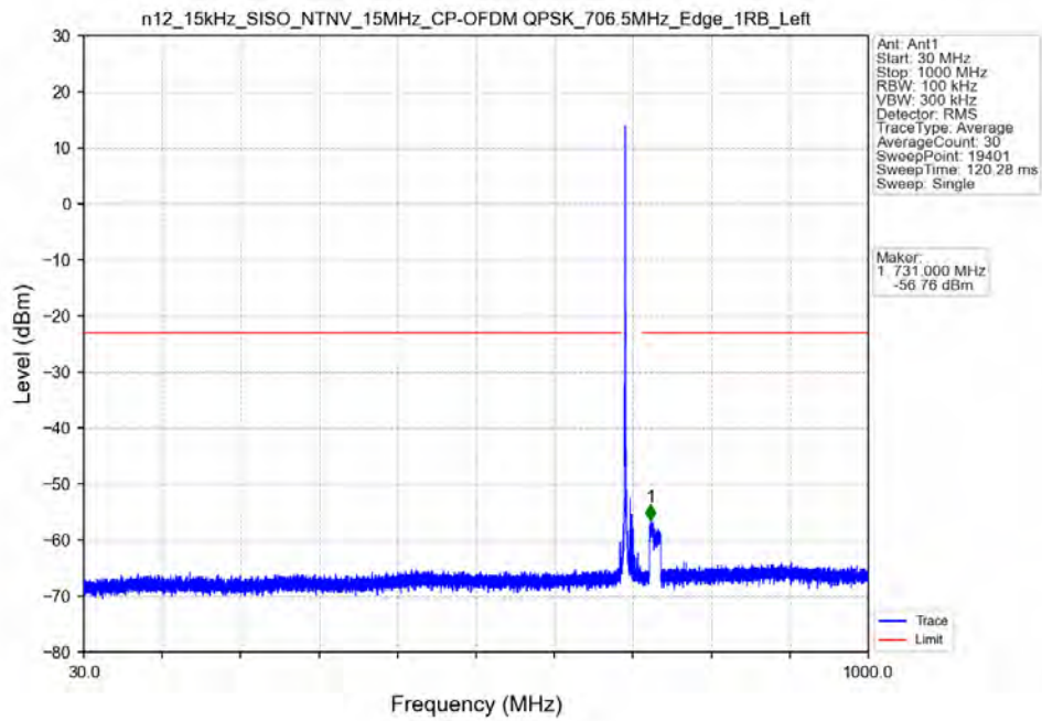
n12_15kHz_SISO_NTNV_15MHz_CP-OFDM_QPSK_706.5MHz_Edge_1RB_Left
