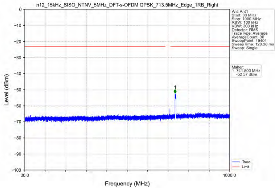
n12_15kHz_SISO_NTNV_5MHz_DFT-s-OFDM_QPSK_713.5MHz_Edge_1RB_Right
