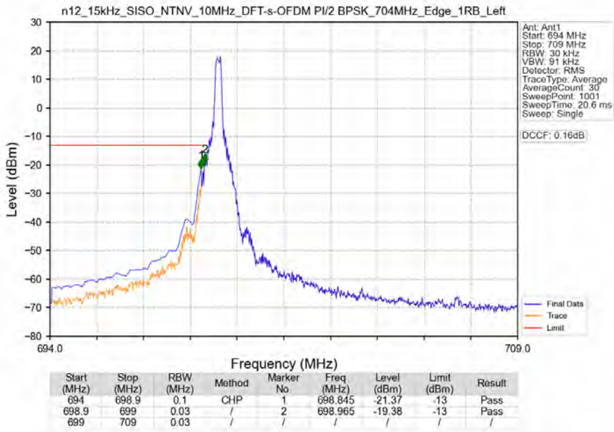
n12_15kHz_SISO_NTNV_10MHz_DFT-s-OFDM PI/2 BPSK_704MHz_Edge_1RB_Left
