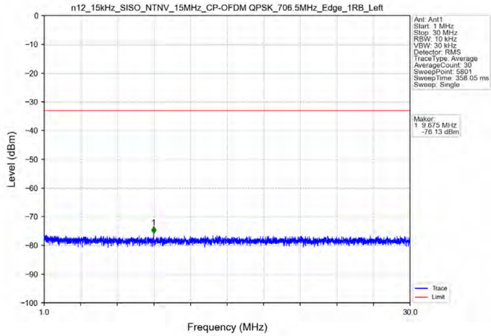
n12_15kHz_SISO_NTNV_15MHz_CP-OFDM_QPSK_706.5MHz_Edge_1RB_Left
