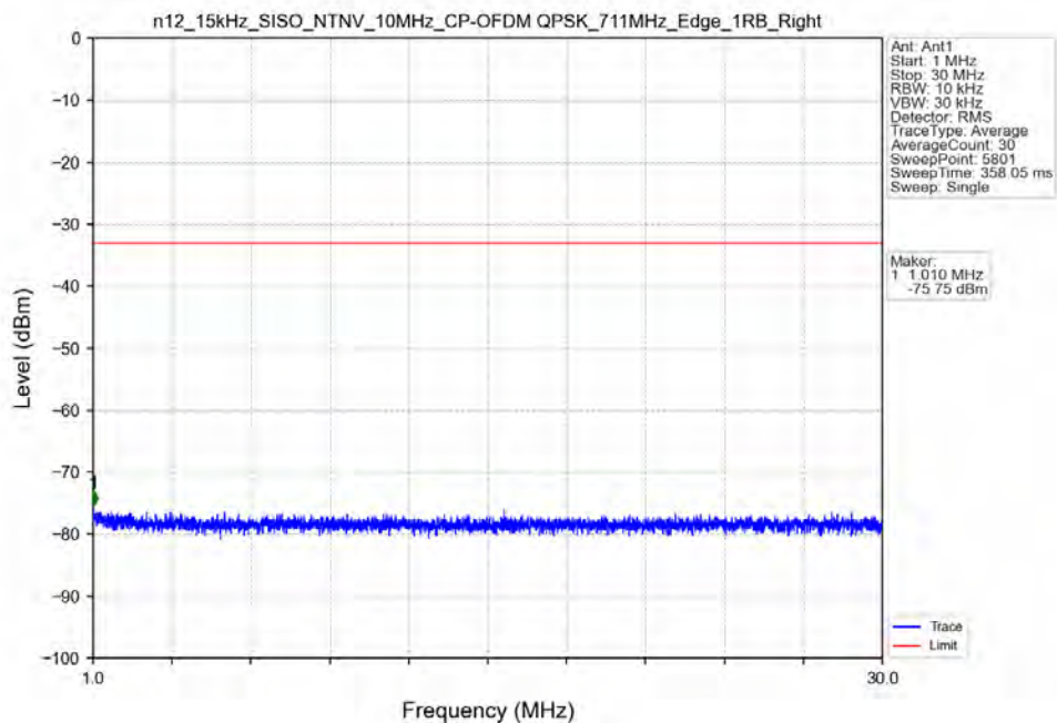
n12_15kHz_SISO_NTNV_10MHz_CP-OFDM_QPSK_711MHz_Edge_1RB_Right
