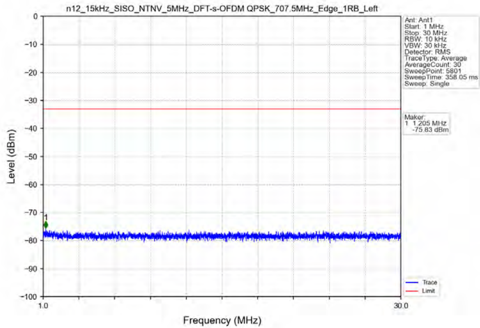
n12_15kHz_SISO_NTNV_5MHz_DFT-s-OFDM_QPSK_707.5MHz_Edge_1RB_Left
