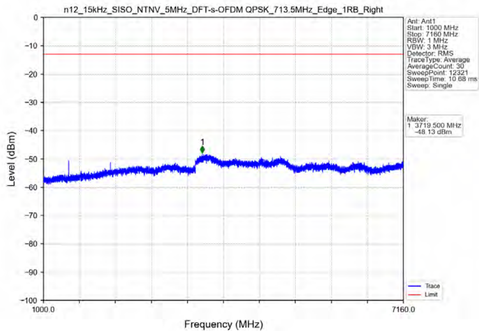
n12_15kHz_SISO_NTNV_5MHz_DFT-s-OFDM_QPSK_713.5MHz_Edge_1RB_Right
