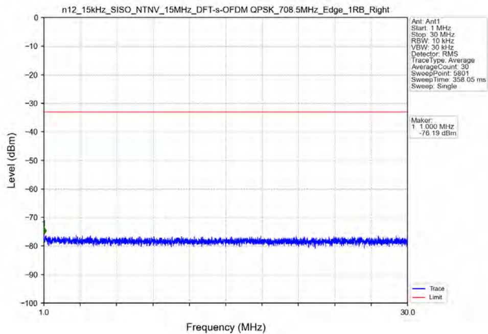
n12_15kHz_SISO_NTNV_15MHz_DFT-s-OFDM_QPSK_708.5MHz_Edge_1RB_Right
