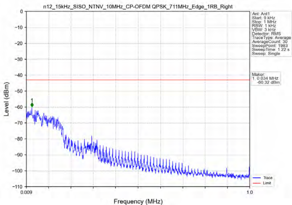
n12_15kHz_SISO_NTNV_10MHz_CP-OFDM_QPSK_711MHz_Edge_1RB_Right
