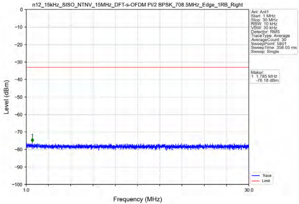
n12_15kHz_SISO_NTNV_15MHz_DFT-s-OFDM PI/2 BPSK_708.5MHz_Edge_1RB_Right
