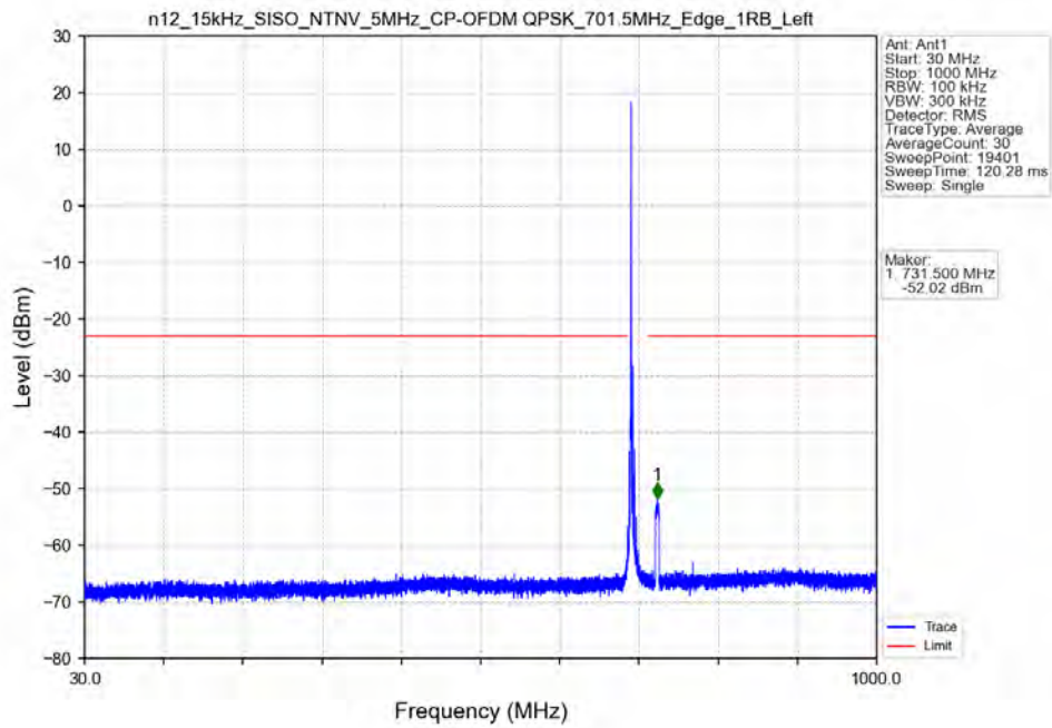
n12_15kHz_SISO_NTNV_5MHz_CP-OFDM_QPSK_701.5MHz_Edge_1RB_Left
