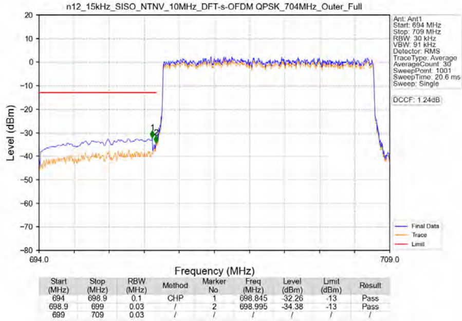
n12_15kHz_SISO_NTNV_10MHz_DFT-s-OFDM_QPSK_704MHz_Outer_Full
