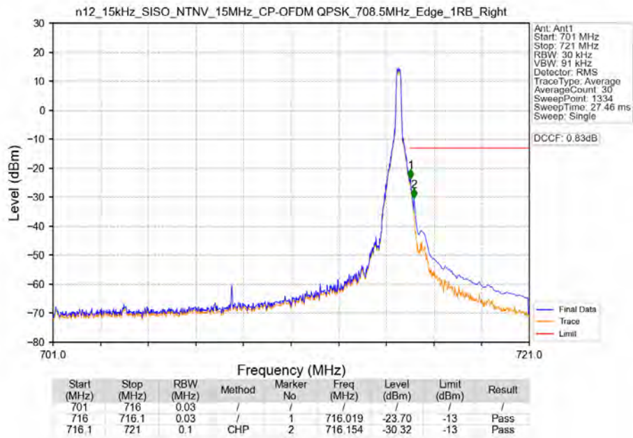
n12_15kHz_SISO_NTNV_15MHz_CP-OFDM_QPSK_708.5MHz_Edge_1RB_Right
