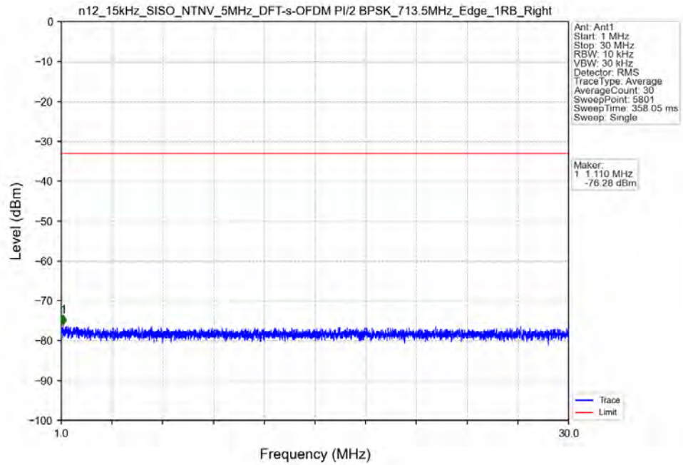
n12_15kHz_SISO_NTNV_5MHz_DFT-s-OFDM PI/2 BPSK_713.5MHz_Edge_1RB_Right
