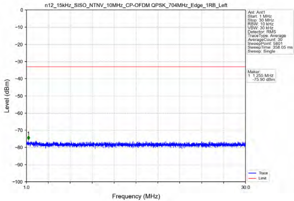
n12_15kHz_SISO_NTNV_10MHz_CP-OFDM_QPSK_704MHz_Edge_1RB_Left
