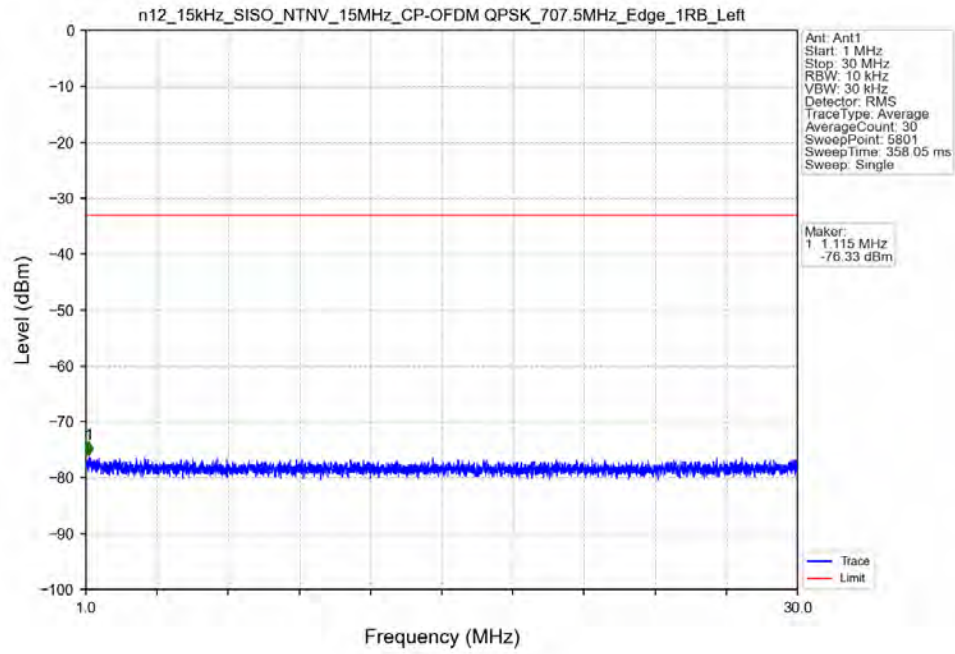
n12_15kHz_SISO_NTNV_15MHz_CP-OFDM_QPSK_707.5MHz_Edge_1RB_Left
