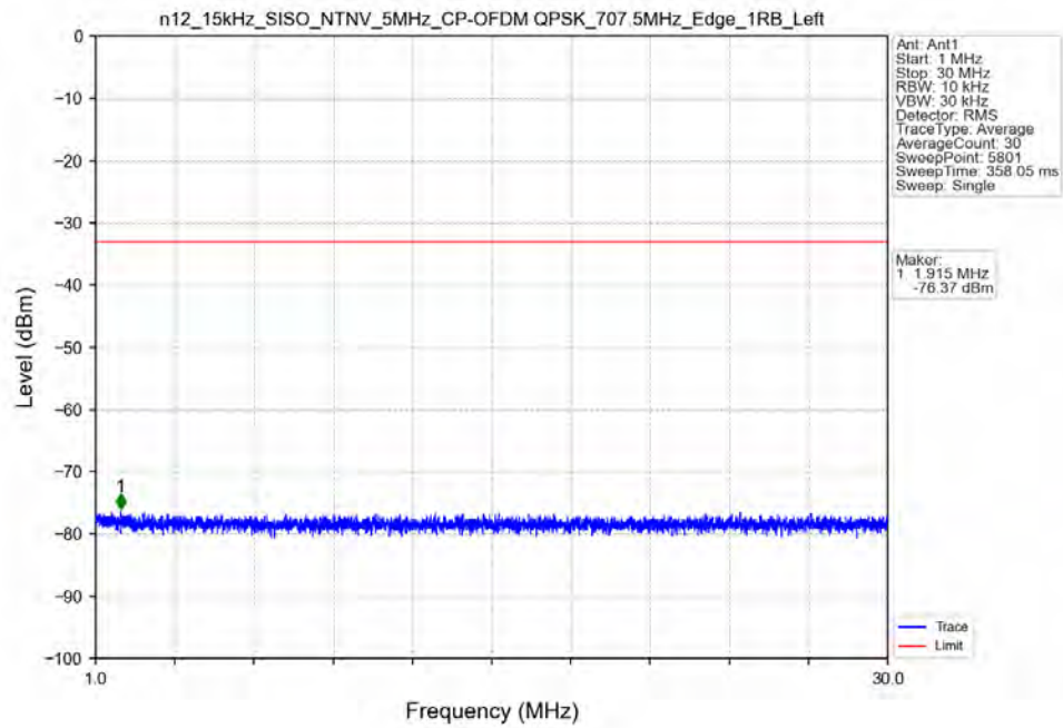
n12_15kHz_SISO_NTNV_5MHz_CP-OFDM_QPSK_707.5MHz_Edge_1RB_Left
