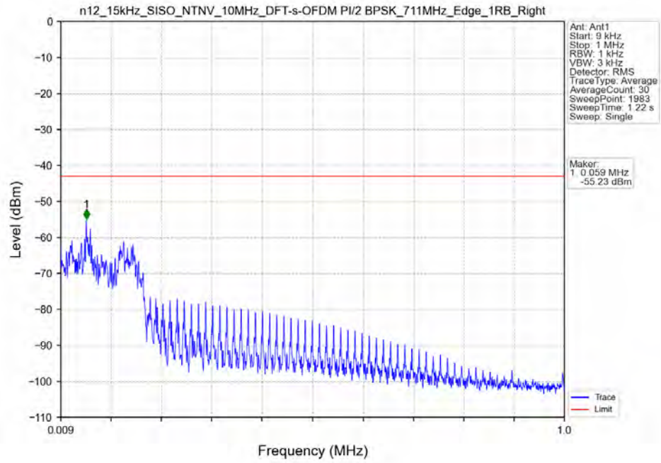
n12_15kHz_SISO_NTNV_10MHz_DFT-s-OFDM PI/2 BPSK_711MHz_Edge_1RB_Right
