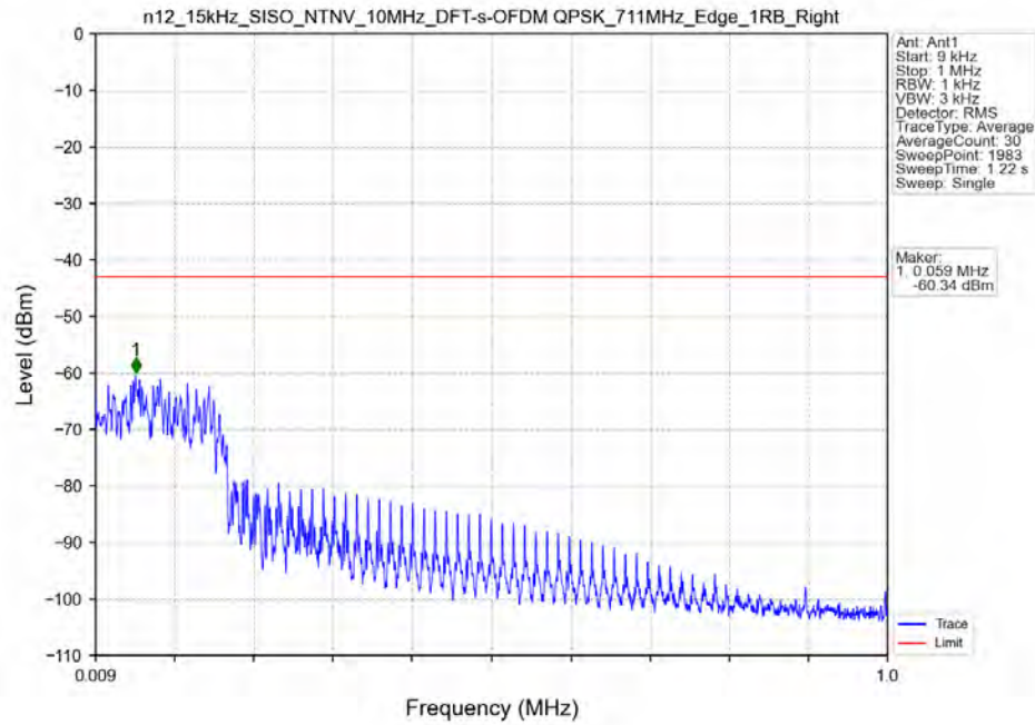
n12_15kHz_SISO_NTNV_10MHz_DFT-s-OFDM_QPSK_711MHz_Edge_1RB_Right
