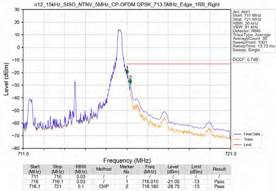
n12_15kHz_SISO_NTNV_5MHz_CP-OFDM_QPSK_713.5MHz_Edge_1RB_Right
