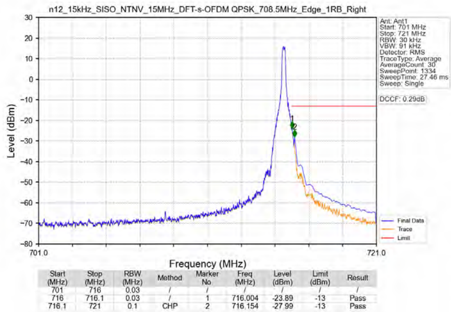
n12_15kHz_SISO_NTNV_15MHz_DFT-s-OFDM_QPSK_708.5MHz_Edge_1RB_Right
