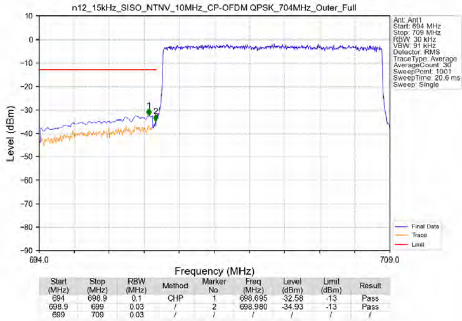
n12_15kHz_SISO_NTNV_10MHz_CP-OFDM_QPSK_704MHz_Outer_Full
