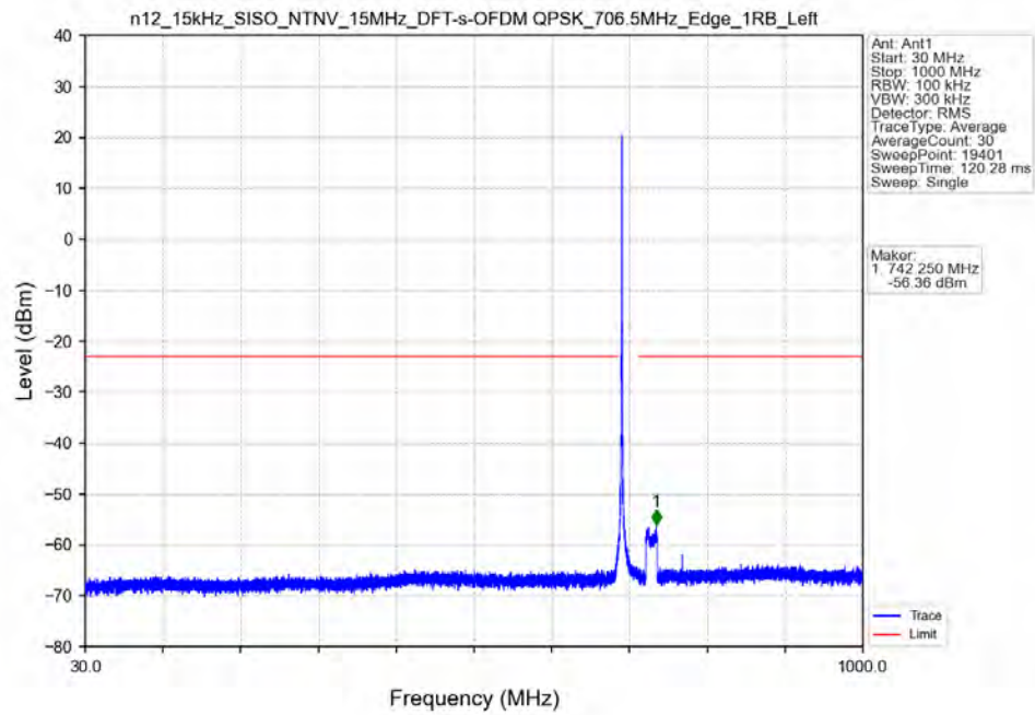
n12_15kHz_SISO_NTNV_15MHz_DFT-s-OFDM_QPSK_706.5MHz_Edge_1RB_Left
