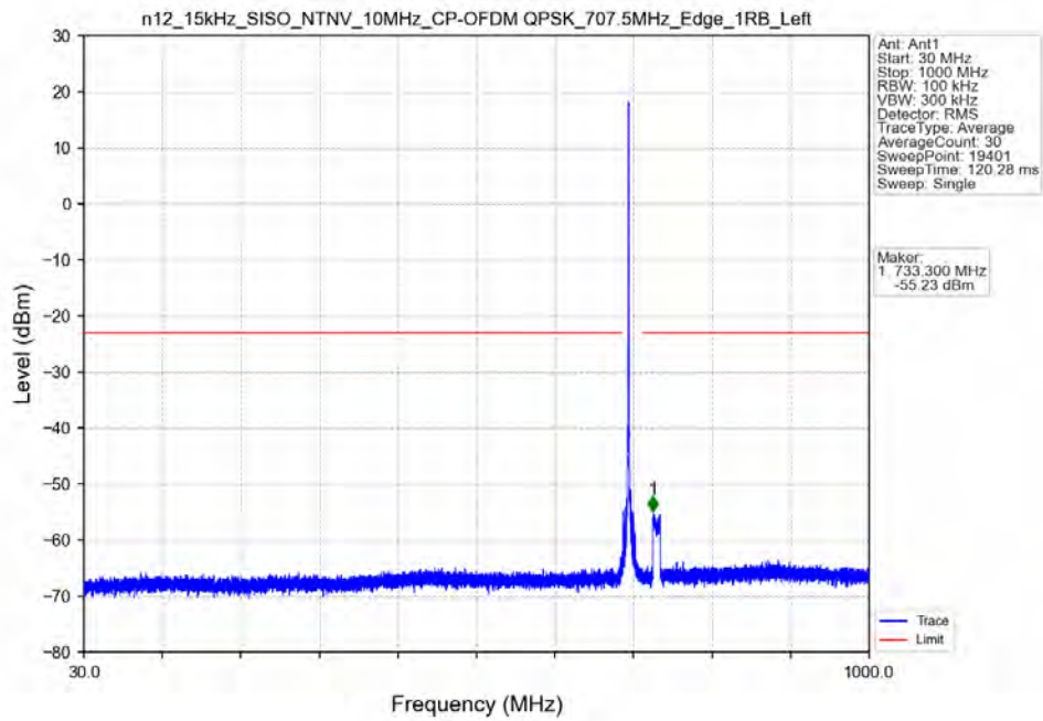
n12_15kHz_SISO_NTNV_10MHz_CP-OFDM_QPSK_707.5MHz_Edge_1RB_Left
