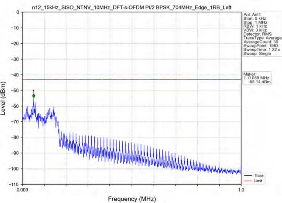
n12_15kHz_SISO_NTNV_10MHz_DFT-s-OFDM PI/2 BPSK_704MHz_Edge_1RB_Left
