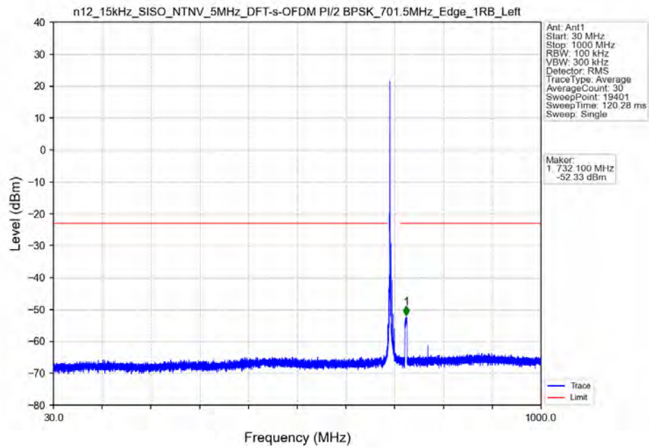
n12_15kHz_SISO_NTNV_5MHz_DFT-s-OFDM PI/2 BPSK 701.5MHz_Edge_1RB_Left
