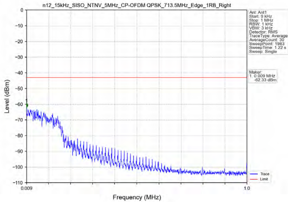
n12_15kHz_SISO_NTNV_5MHz_CP-OFDM QPSK_713.5MHz_Edge_1RB_Right
