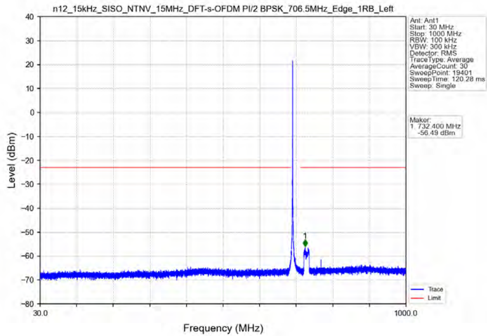
n12_15kHz_SISO_NTNV_15MHz_DFT-s-OFDM_PI/2_BPSK_706.5MHz_Edge_1RB_Left
