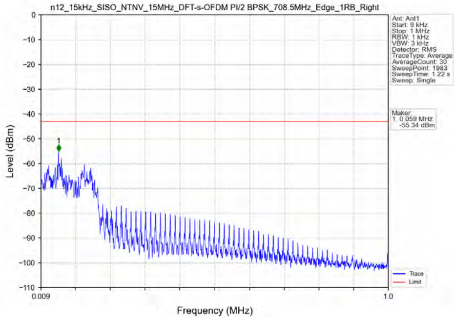
n12_15kHz_SISO_NTNV_15MHz_DFT-s-OFDM PI/2 BPSK_708.5MHz_Edge_1RB_Right
