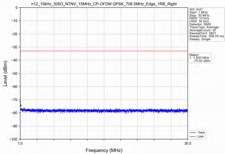
n12_15kHz_SISO_NTNV_15MHz_CP-OFDM_QPSK_708.5MHz_Edge_1RB_Right
