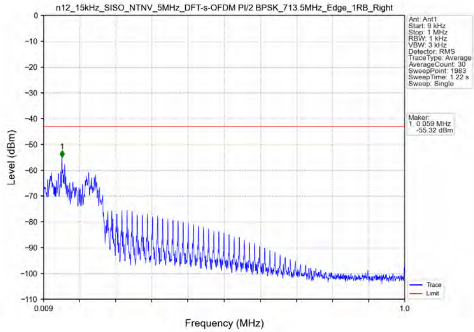
n12_15kHz_SISO_NTNV_5MHz_DFT-s-OFDM PI/2 BPSK_713.5MHz_Edge_1RB_Right
