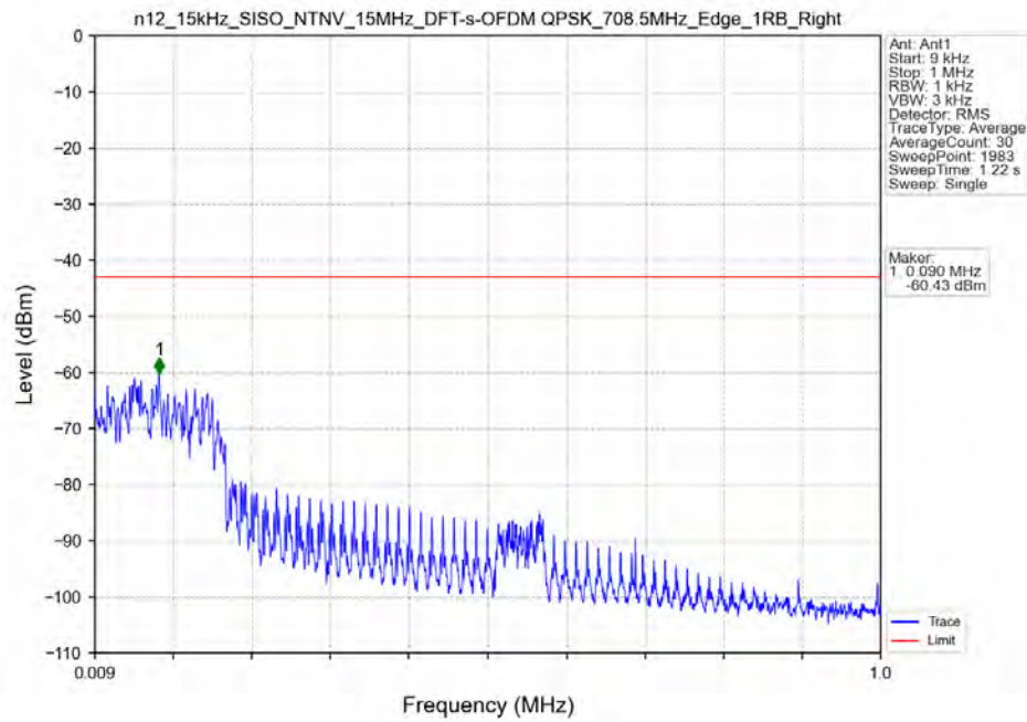
n12_15kHz_SISO_NTNV_15MHz_DFT-s-OFDM_QPSK_708.5MHz_Edge_1RB_Right
