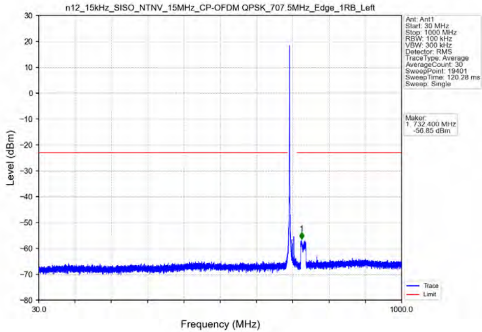
n12_15kHz_SISO_NTNV_15MHz_CP-OFDM_QPSK_707.5MHz_Edge_1RB_Left
