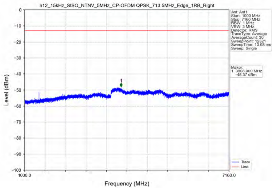
n12_15kHz_SISO_NTNV_5MHz_CP-OFDM QPSK_713.5MHz_Edge_1RB_Right
