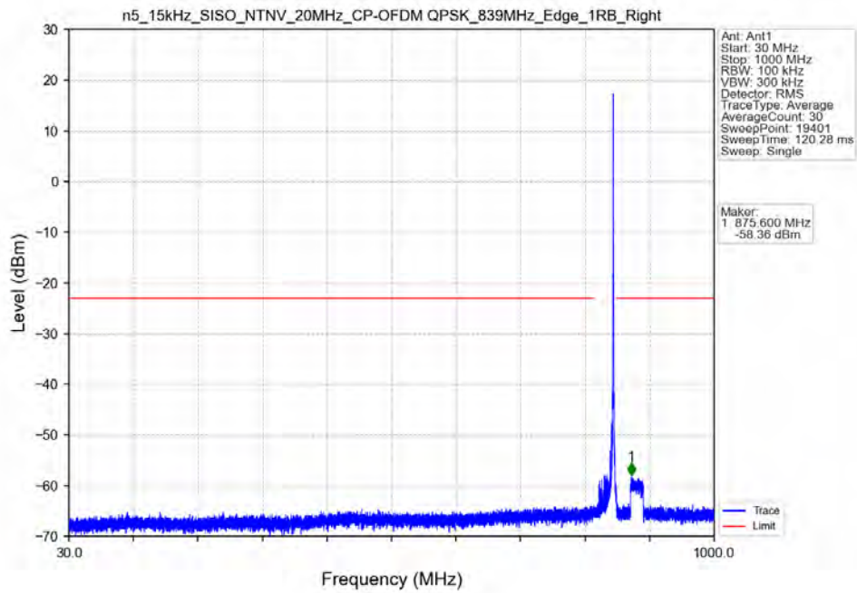
n5_15kHz_SISO_NTNV_20MHz_CP-OFDM_QPSK_839MHz_Edge_1RB_Right
