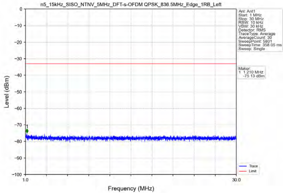
n5_15kHz_SISO_NTNV_5MHz_DFT-s-OFDM_QPSK_836.5MHz_Edge_1RB_Left
