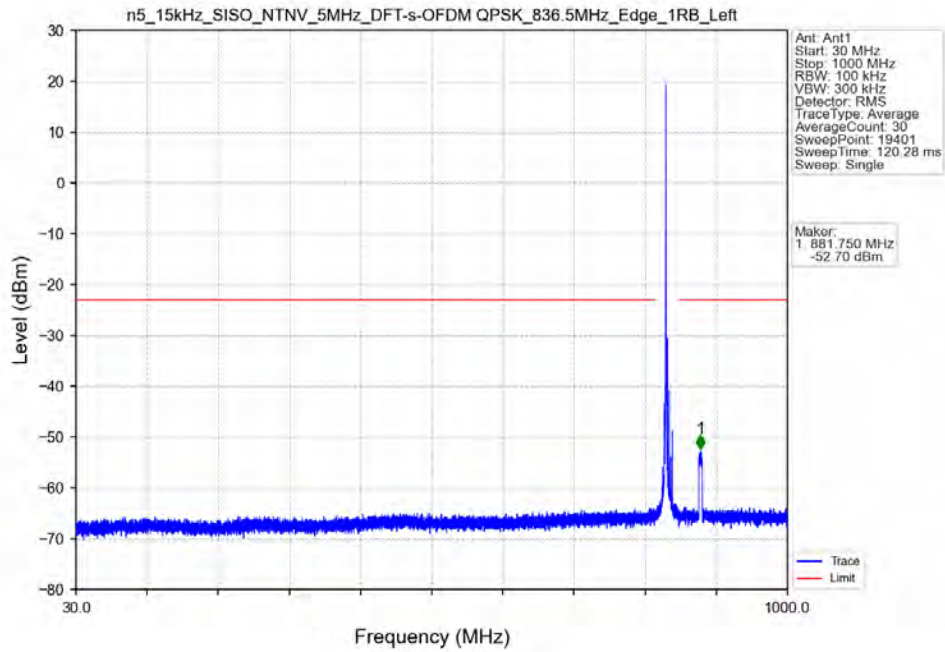
n5_15kHz_SISO_NTNV_5MHz_DFT-s-OFDM_QPSK_836.5MHz_Edge_1RB_Left
