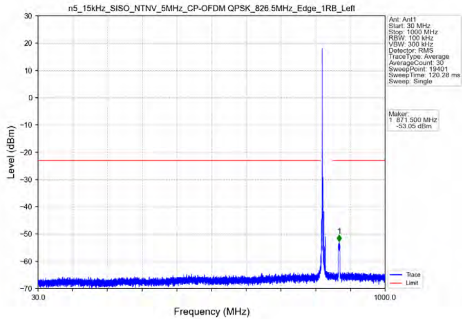
n5_15kHz_SISO_NTNV_5MHz_CP-OFDM_QPSK_826.5MHz_Edge_1RB_Left
