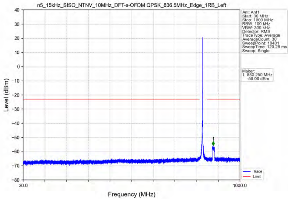
n5_15kHz_SISO_NTNV_10MHz_DFT-s-OFDM_QPSK_836.5MHz_Edge_1RB_Left
