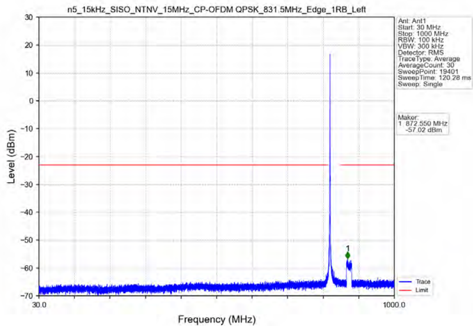
n5_15kHz_SISO_NTNV_15MHz_CP-OFDM_QPSK_831.5MHz_Edge_1RB_Left
