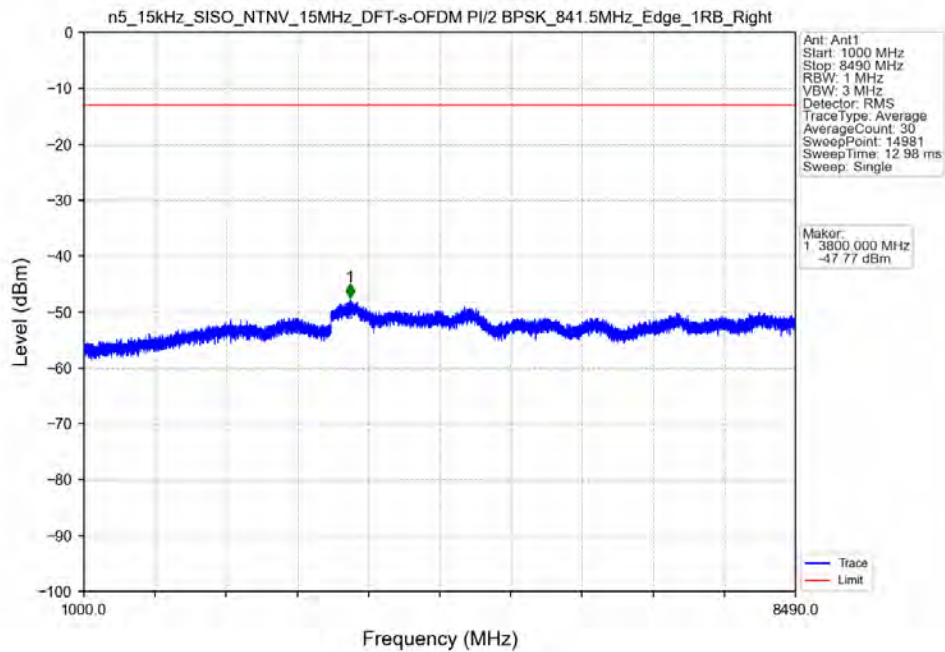
n5_15kHz_SISO_NTNV_15MHz_DFT-s-OFDM_PI/2_BPSK_841.5MHz_Edge_1RB_Right
