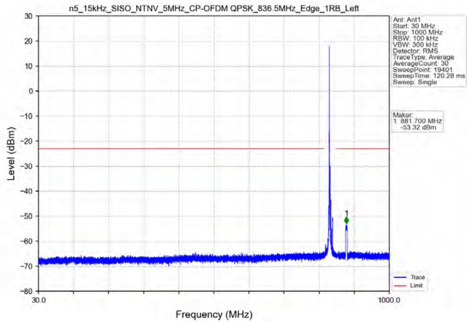
n5_15kHz_SISO_NTNV_5MHz_CP-OFDM_QPSK_836.5MHz_Edge_1RB_Left
