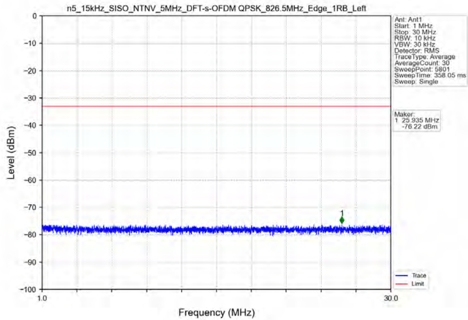
n5_15kHz_SISO_NTNV_5MHz_DFT-s-OFDM_QPSK_826.5MHz_Edge_1RB_Left
