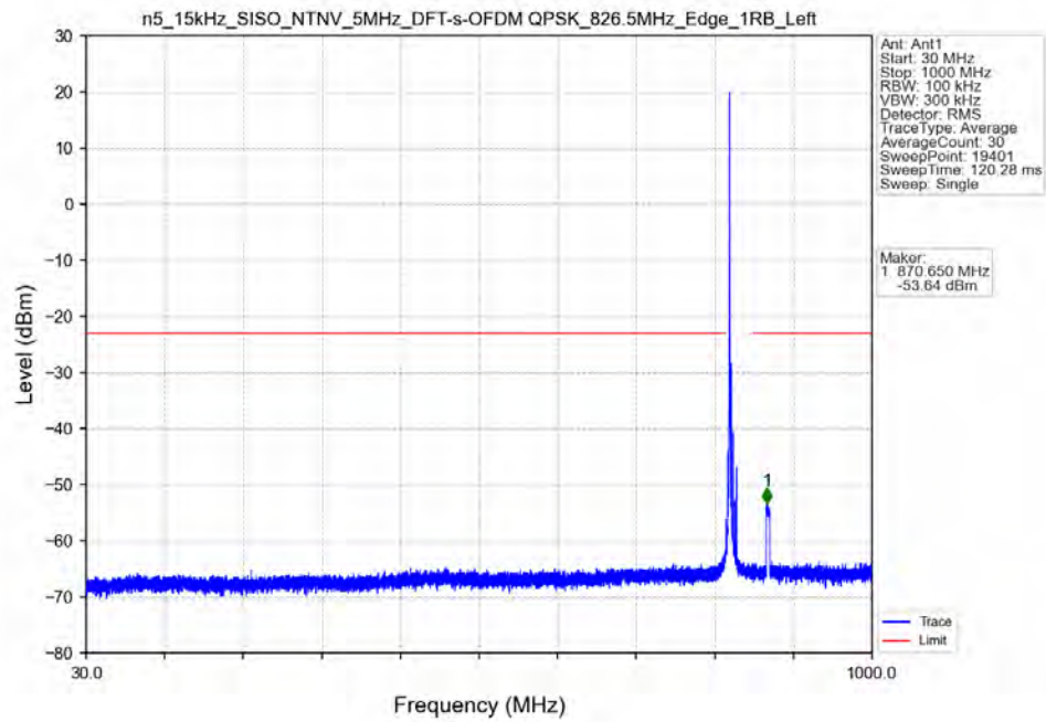
n5_15kHz_SISO_NTNV_5MHz_DFT-s-OFDM_QPSK_826.5MHz_Edge_1RB_Left
