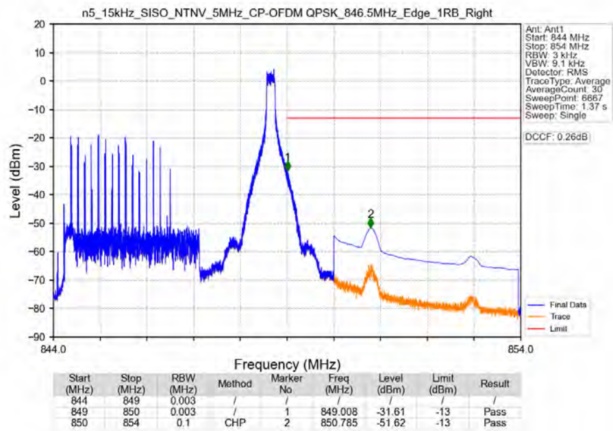
n5_15kHz_SISO_NTNV_5MHz_CP-OFDM_QPSK_846.5MHz_Edge_1RB_Right
