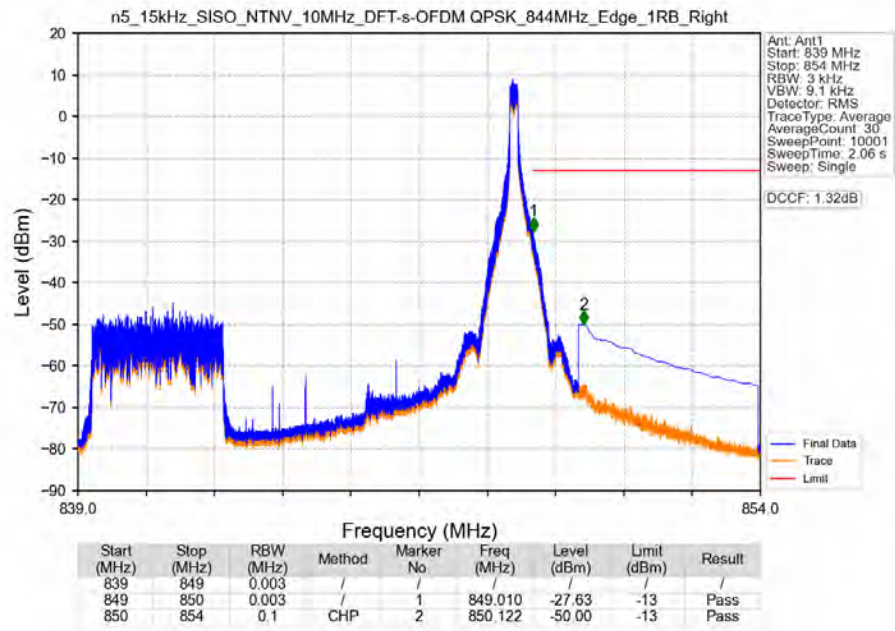
n5_15kHz_SISO_NTNV_10MHz_DFT-s-OFDM_QPSK_844MHz_Edge_1RB_Right
