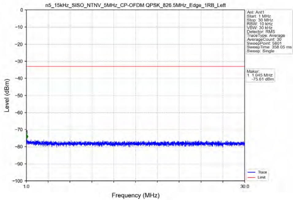
n5_15kHz_SISO_NTNV_5MHz_CP-OFDM_QPSK_826.5MHz_Edge_1RB_Left
