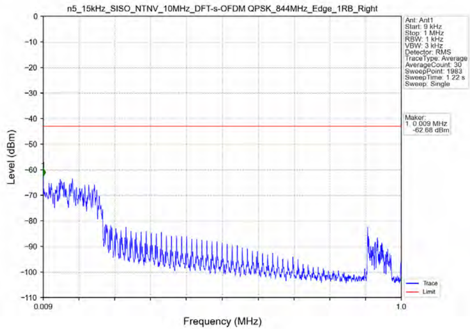
n5_15kHz_SISO_NTNV_10MHz_DFT-s-OFDM_QPSK_844MHz_Edge_1RB_Right
