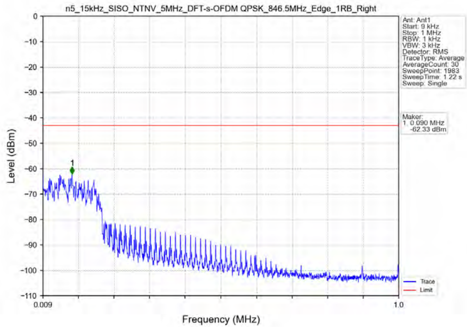
n5_15kHz_SISO_NTNV_5MHz_DFT-s-OFDM_QPSK_846.5MHz_Edge_1RB_Right
