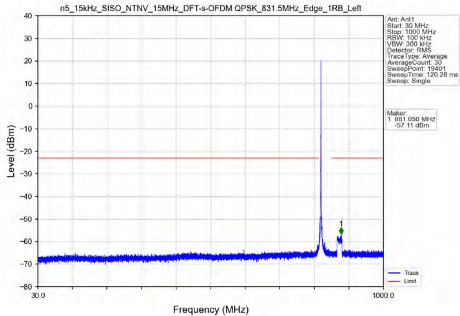
n5_15kHz_SISO_NTNV_15MHz_DFT-s-OFDM_QPSK_831.5MHz_Edge_1RB_Left
