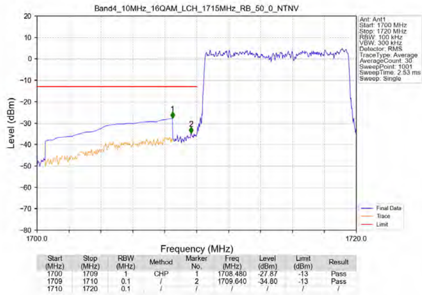
Band4_10MHz_16QAM_LCH_1715MHz_RB_50_0_NTNV
