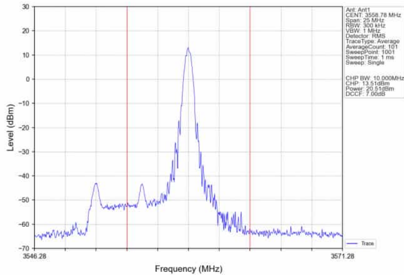
n48_30kHz_SISO_NTNV_10MHz_DFT-s-OFDM_QPSK_3555MHz_Inner_1RB_Right
