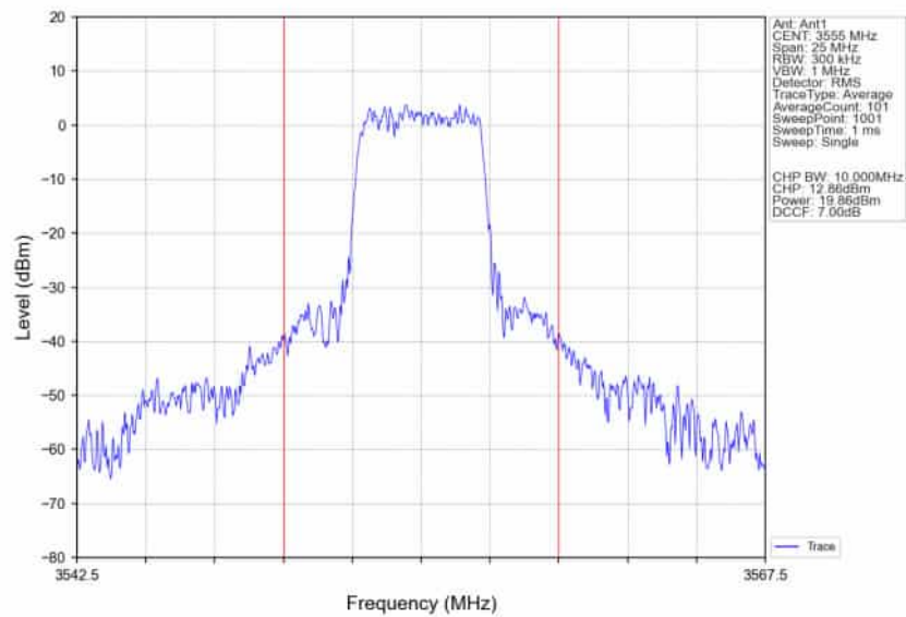
n48 30kHz SISO NTN 10MHz DFT-s-OFDM PI/2 BPSK 3555MHz Inner Full
