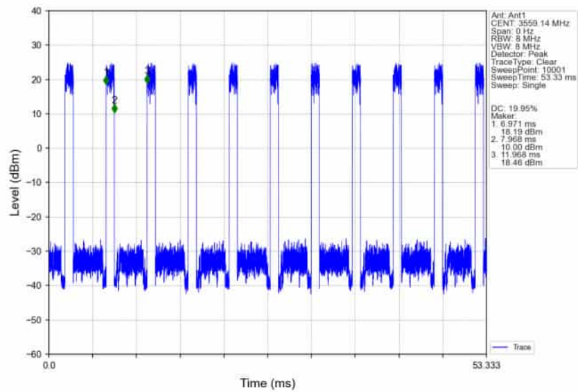
n48_30kHz_SISO_NTNV_10MHz_DFT-s-OFDM_64_QAM_3555MHz_Edge_1RB_Right
