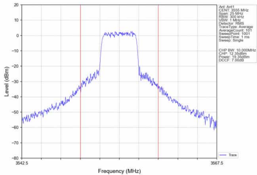
n48_30kHz_SISO_NTNV_10MHz_CP-OFDM_QPSK_3555MHz_Inner_Full
