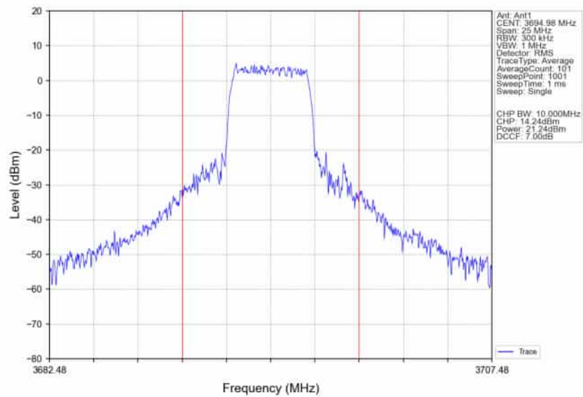
n48_30kHz_SISO_NTNV_10MHz_CP-OFDM_QPSK_3694.98MHz_Inner_Full
