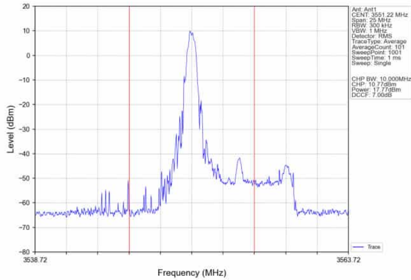
n48_30kHz_SISO_NTNV_10MHz_CP-OFDM_16_QAM_3555MHz_Inner_1RB_Right
