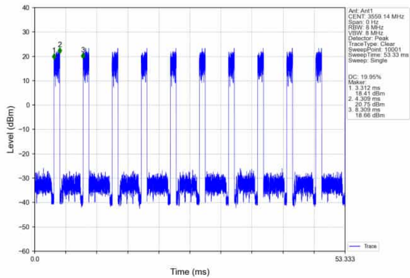
n48_30kHz_SISO_NTNV_10MHz_CP-OFDM_256_QAM_3555MHz_Edge_1RB_Right
