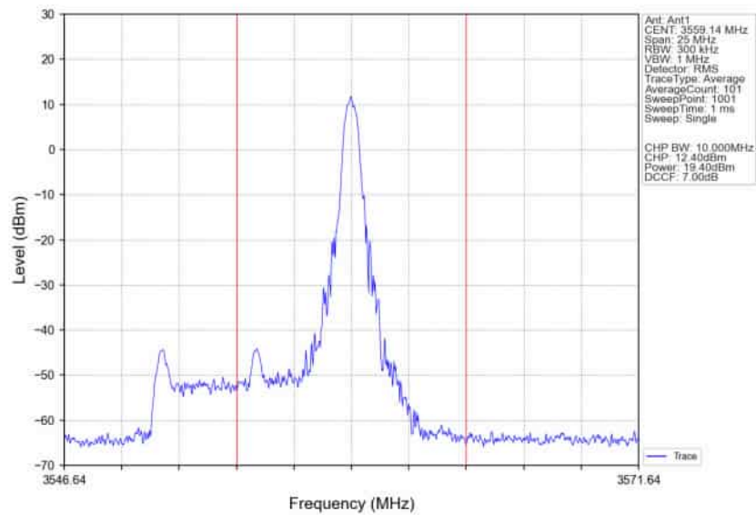
n48_30kHz_SISO_NTNV_10MHz_DFT-s-OFDM_QPSK_3555MHz_Edge_1RB_Right
