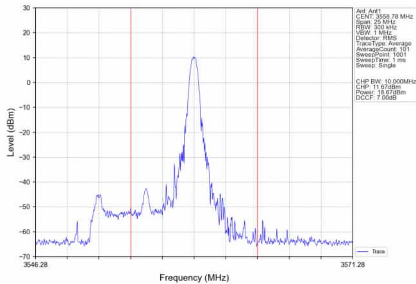
n48_30kHz_SISO_NTNV_10MHz_CP-OFDM_16_QAM_3555MHz_Inner_1RB_Right
