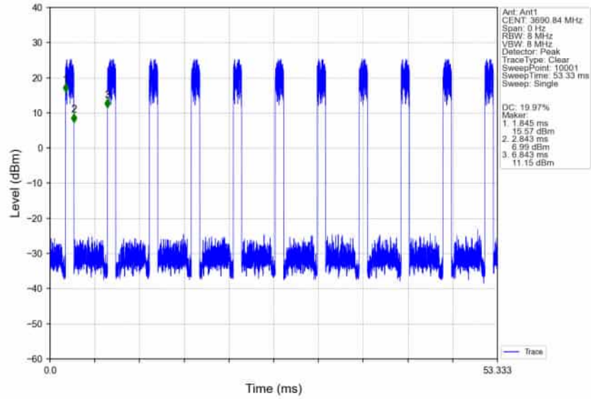
n48_30kHz_SISO_NTNV_10MHz_CP-OFDM_64_QAM_3694.98MHz_Edge_1RB_Right
