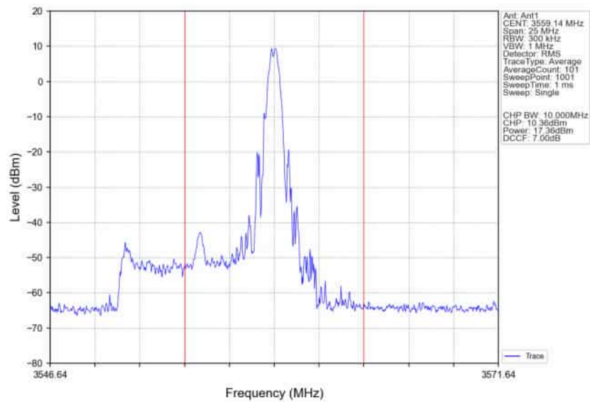
n48_30kHz_SISO_NTNV_10MHz_CP-OFDM_64_QAM_3555MHz_Edge_1RB_Right
