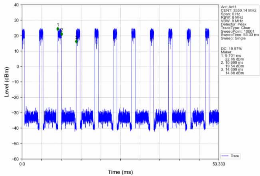
n48_30kHz_SISO_NTNV_10MHz_DFT-s-OFDM_16_QAM_3555MHz_Edge_1RB_Right
