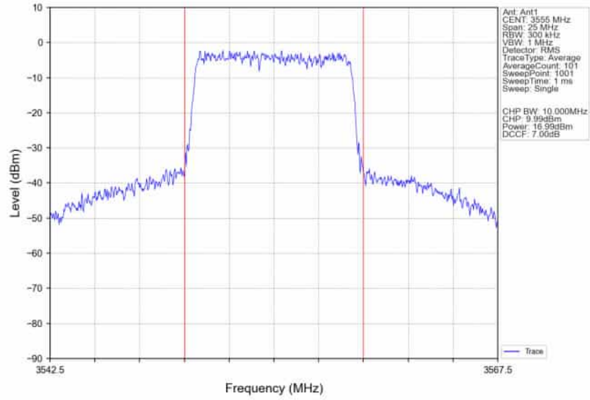
n48_30kHz_SISO_NTNV_10MHz_CP-OFDM_QPSK_3555MHz_Inner_Full
