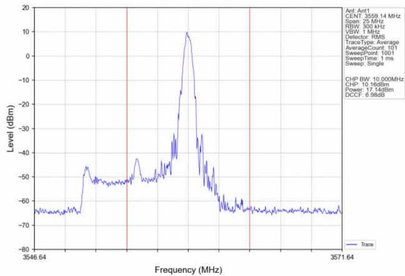
n48_30kHz_SISO_NTNV_10MHz_CP-OFDM_16_QAM_3555MHz_Edge_1RB_Right
