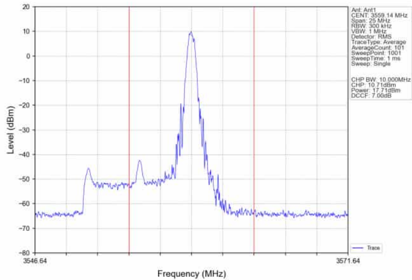
n48_30kHz_SISO_NTNV_10MHz_DFT-s-OFDM_64_QAM_3555MHz_Edge_1RB_Right
