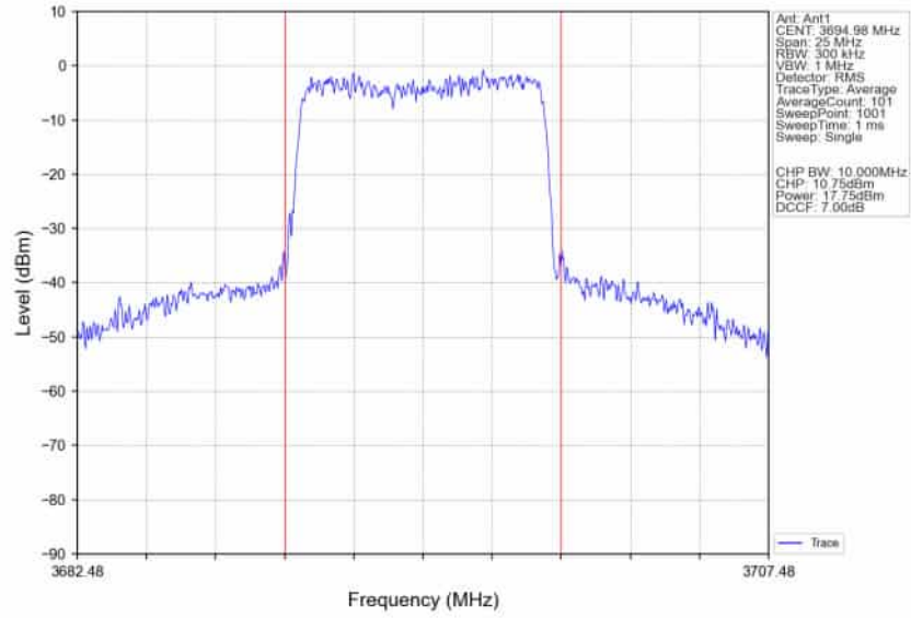
n48_30kHz_SISO_NTNV_10MHz_CP-OFDM_QPSK_3694.98MHz_Inner_Full
