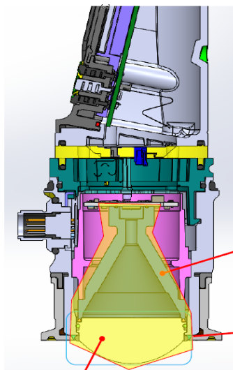
Horn & Lens antenna (Yellow zone)
