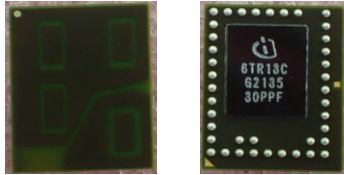
Wireless IC side (Black center IC is wireless IC)
