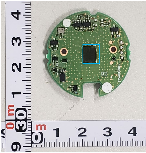
Wireless IC side (Black center IC is wireless IC)
