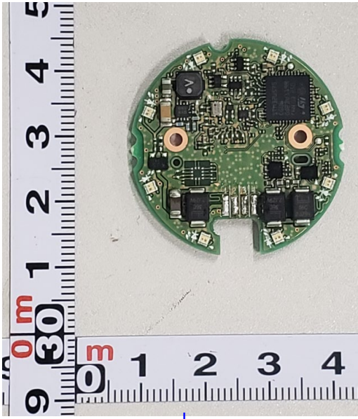
Below internal photo is back side of board.
