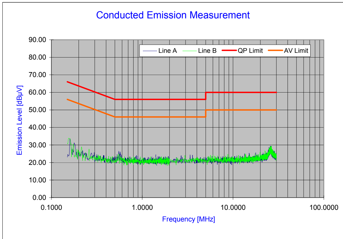
Plot 8-2. Line-Conducted Test Plot
