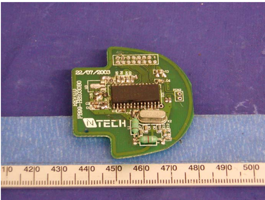
EUT – Solder View, Top PCB
