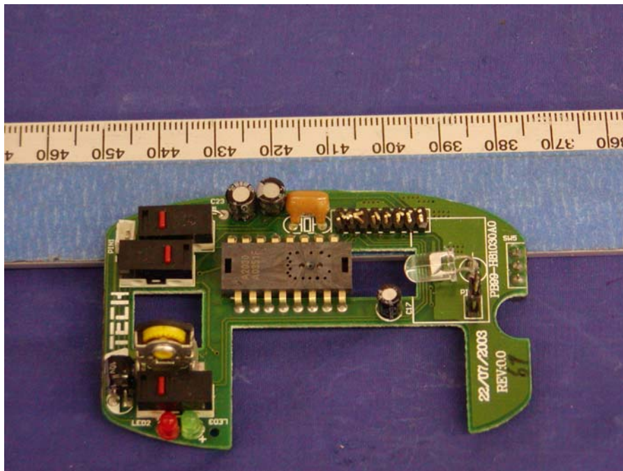
EUT – Component View, Bottom PCB
