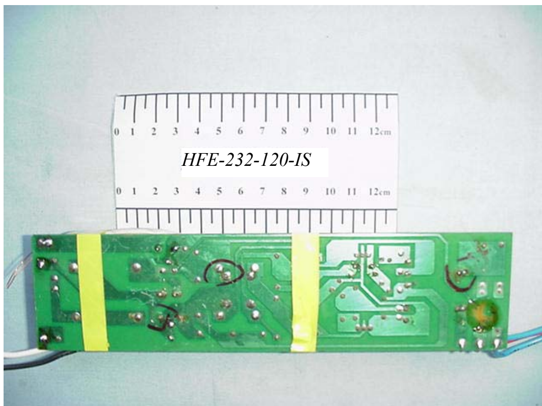
FIGURE 3 ENERGY SAVING LAMP (M/N: HFE-232-120-IS) MAIN BOARD (SOLDERED SIDE)
