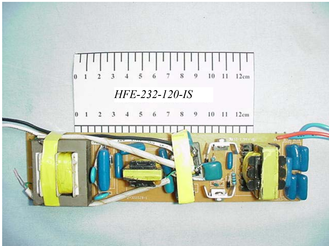
FIGURE 2 ENERGY SAVING LAMP (M/N: HFE-232-120-IS) MAIN BOARD (COMPONENT SIDE)
