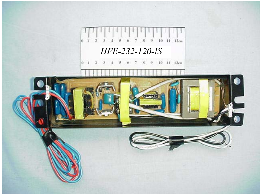
FIGURE 1 ENERGY SAVING LAMP (M/N: HFE-232-120-IS) COVER REMOVED
