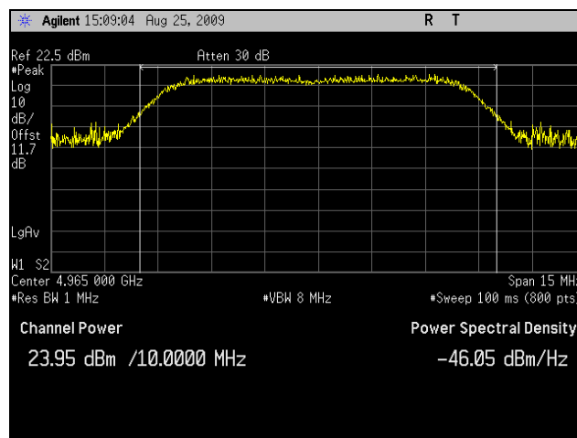
Plot 5. RF Power Output, Mid Channel, 802.11a, Mid Channel, 10 MHz
