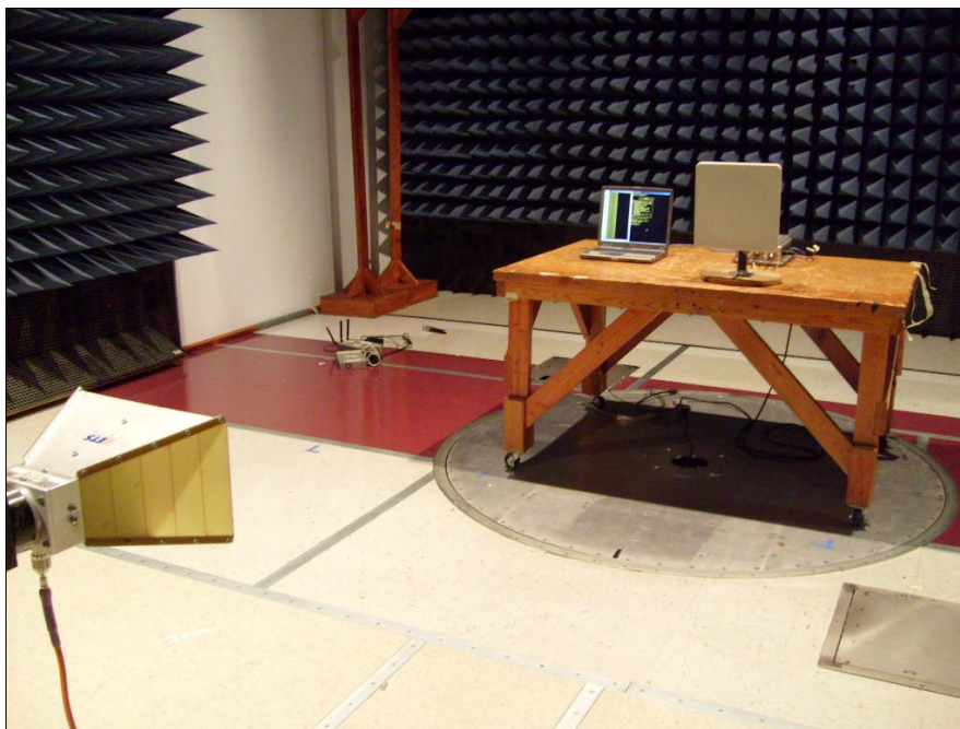
Photograph 10. Test Equipment and Setup for Various Radiated Measurements – 19 dBi Panel
