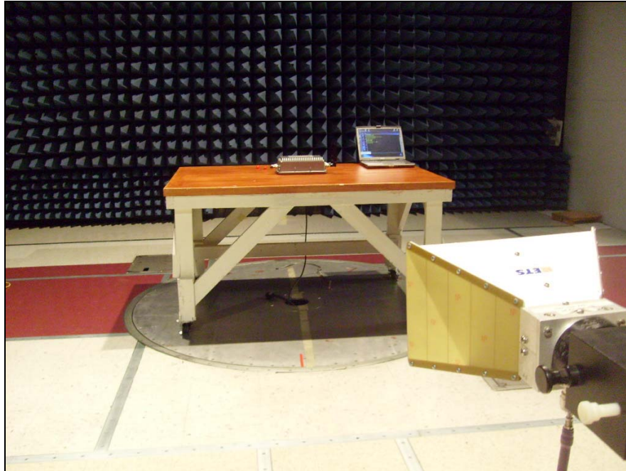
Photograph 6. Test Equipment and Setup for Various Radiated Measurements – 5 dBi Omni
