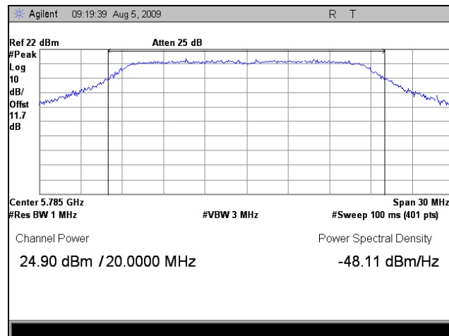
Plot 70. Peak Output Power, Mid Channel, 5 GHz, Port 3, 802.11n 20MHz
