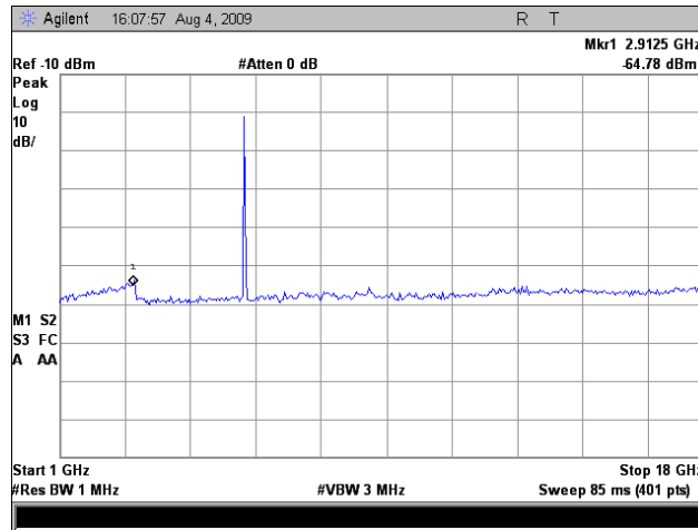
Plot 97. Radiated Spurious Emissions, Mid Channel, 5 GHz, Combined Ports, 802.11n 20MHz, 9 dBi Omni
