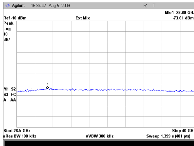
Plot 181. Conducted Emissions, Mid Channel, 5 GHz, Port 1, 802.11n 20MHz, 26.5 GHz – 40 GHz
