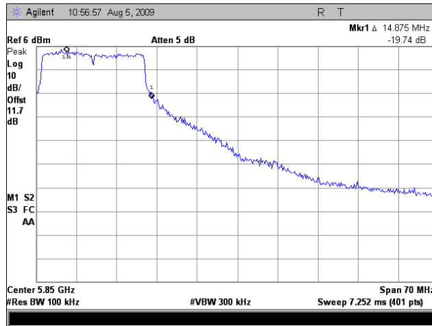
Plot 228. Upper Conducted Band Edge, 5 GHz, Port 2, 802.11n 20MHz
