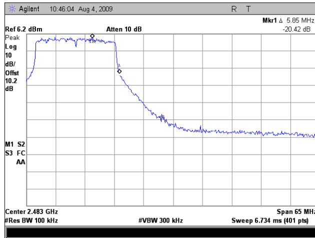
Plot 164. Upper Conducted Band Edge, 2.4 GHz, Port 3, 802.11n 20MHz
