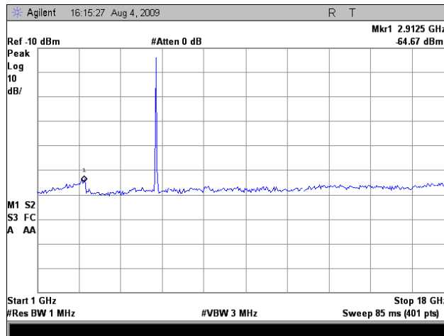
Plot 106. Radiated Spurious Emissions, High Channel, 5 GHz, Combined Ports, 802.11n 20MHz, 16 dBi Sector
