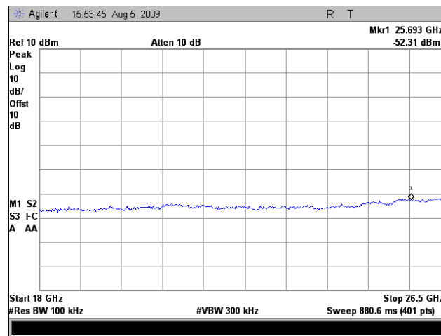
Plot 186. Conducted Emissions, Low Channel, 5 GHz, Port 1, 802.11n 40MHz, 18 GHz – 26.5 GHz
