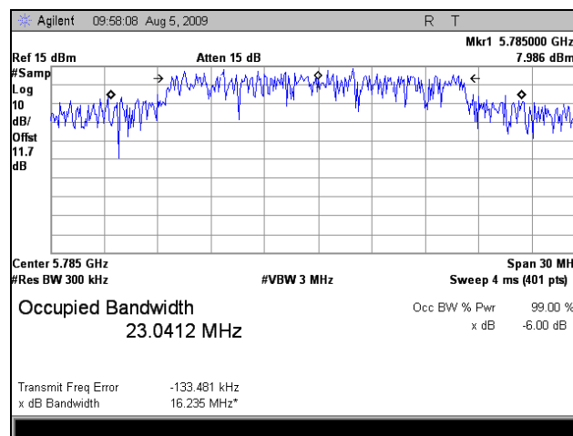
Plot 24. Occupied Band Width, Mid Channel, 5 GHz, Port 1, 802.11a
