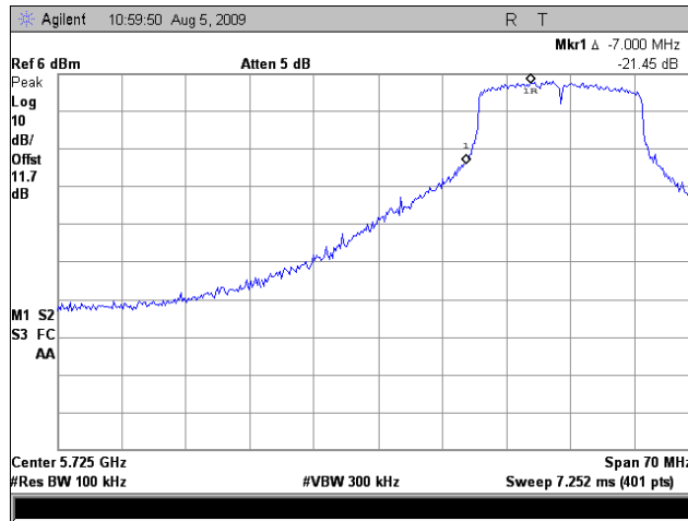
Plot 231. Lower Conducted Band Edge, 5 GHz, Port 3, 802.11n 20MHz
