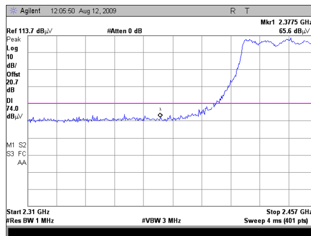
Plot 90. Lower Band Edge, Peak, 2.4 GHz, Combined Ports, 802.11n 40MHz, 13 dBi Sector
