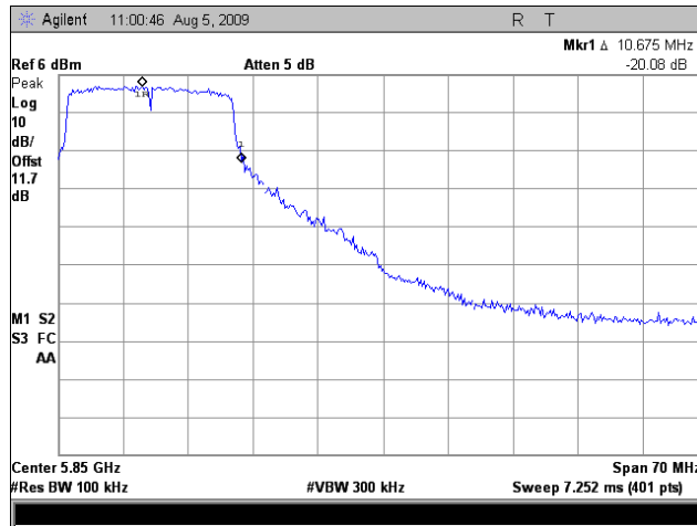
Plot 232. Upper Conducted Band Edge, 5 GHz, Port 3, 802.11n 20MHz
