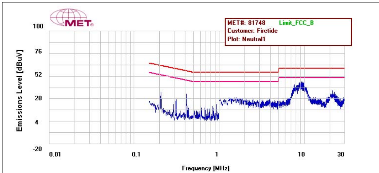
Plot 2. Conducted Emission, Neutral Line Plot
