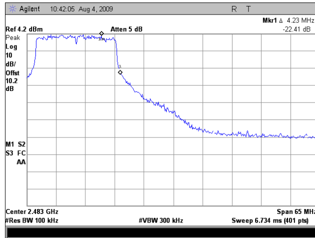
Plot 160. Upper Conducted Band Edge, 2.4 GHz, Port 2, 802.11n 20MHz
