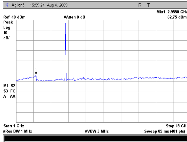
Plot 113. Radiated Spurious Emissions, Mid Channel, 5 GHz, Combined Ports, 802.11n 20MHz, 19 dBi Panel
