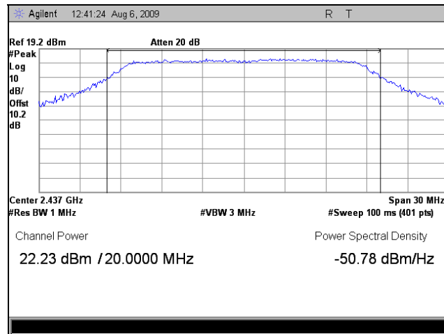
Plot 49. Peak Output Power, Mid Channel, 2.4 GHz, Port 2, 802.11n 20MHz
