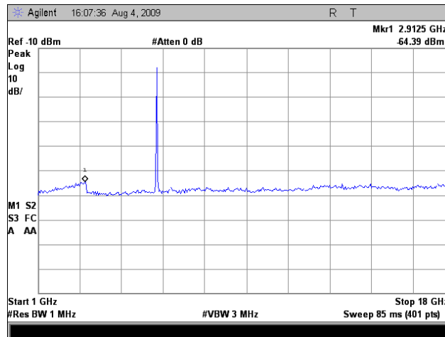
Plot 98. Radiated Spurious Emissions, High Channel, 5 GHz, Combined Ports, 802.11n 20MHz, 9 dBi Omni
