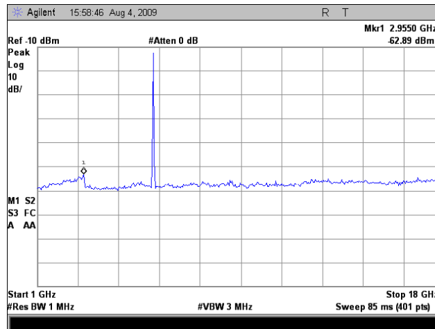
Plot 114. Radiated Spurious Emissions, High Channel, 5 GHz, Combined Ports, 802.11n 20MHz, 19 dBi Panel
