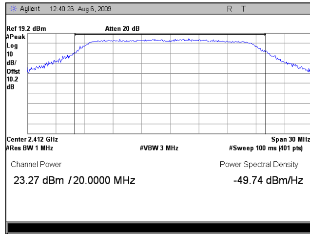
Plot 52. Peak Output Power, Low Channel, 2.4 GHz, Port 3, 802.11n 20MHz
