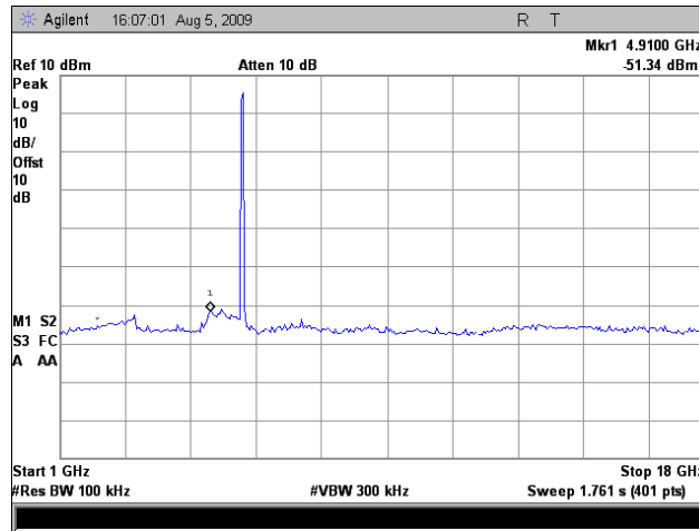
Plot 206. Conducted Emissions, Low Channel, 5 GHz, Port 3, 802.11n 20MHz, 1 GHz – 18 GHz
