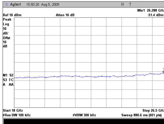
Plot 180. Conducted Emissions, Mid Channel, 5 GHz, Port 1, 802.11n 20MHz, 18 GHz – 26.5 GHz
