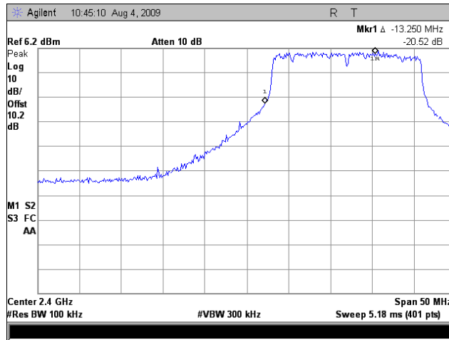
Plot 163. Lower Conducted Band Edge, 2.4 GHz, Port 3, 802.11n 20MHz
