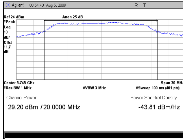
Plot 56. Peak Output Power, Low Channel, 5 GHz, Port 1, 802.11a
