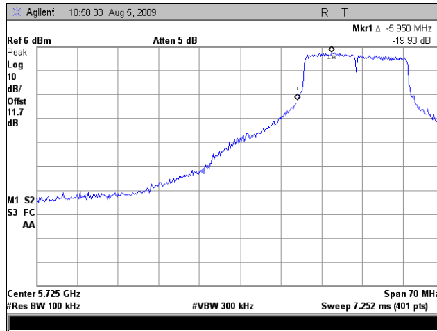
Plot 227. Lower Conducted Band Edge, 5 GHz, Port 2, 802.11n 20MHz
