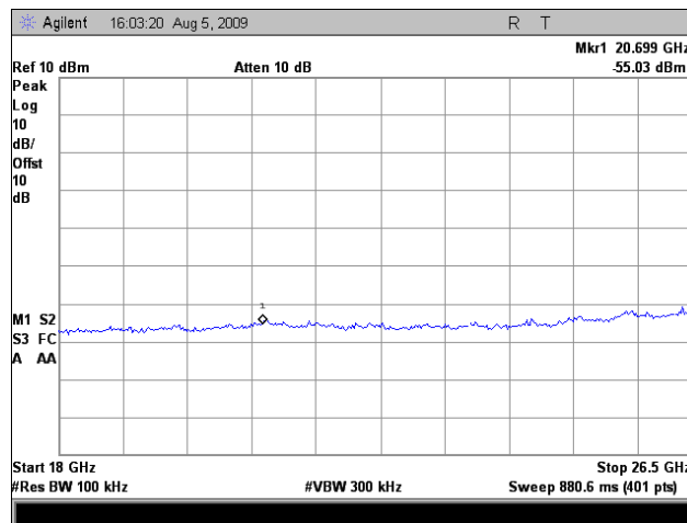
Plot 207. Conducted Emissions, Low Channel, 5 GHz, Port 3, 802.11n 20MHz, 18 GHz – 26.5 GHz
