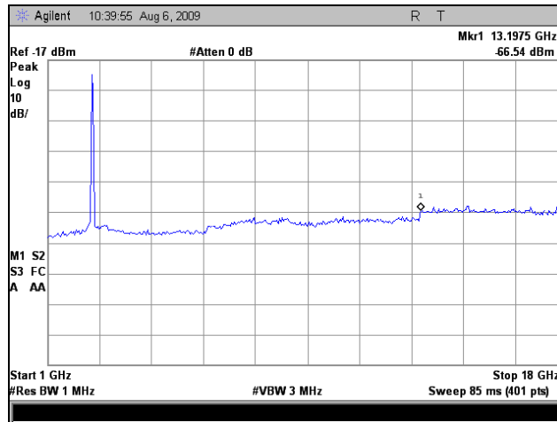
Plot 75. Radiated Spurious Emissions, Mid Channel, 2.4 GHz, 802.11g, 13 dBi Sector
