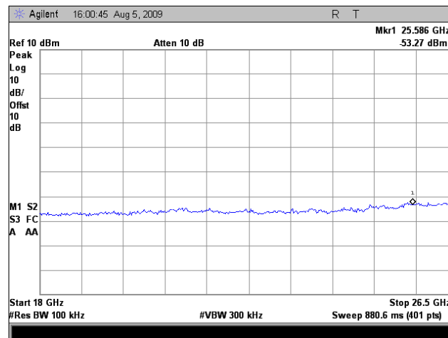
Plot 195. Conducted Emissions, Mid Channel, 5 GHz, Port 2, 802.11n 20MHz, 18 GHz – 26.5 GHz
