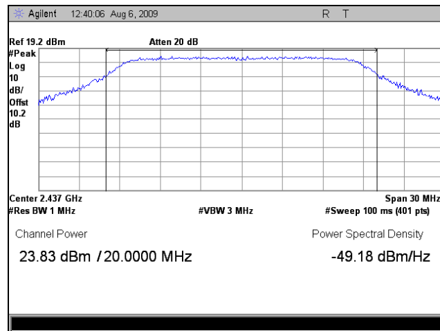
Plot 53. Peak Output Power, Mid Channel, 2.4 GHz, Port 3, 802.11n 20MHz
