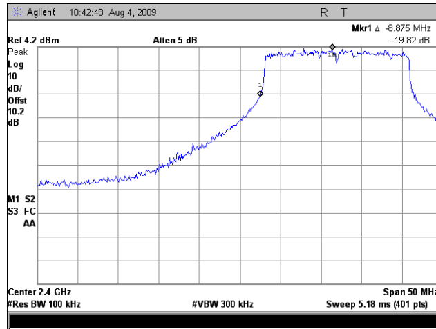
Plot 159. Lower Conducted Band Edge, 2.4 GHz, Port 2, 802.11n 20MHz
