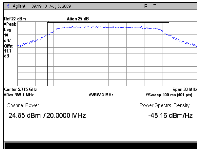
Plot 69. Peak Output Power, Low Channel, 5 GHz, Port 3, 802.11n 20MHz
