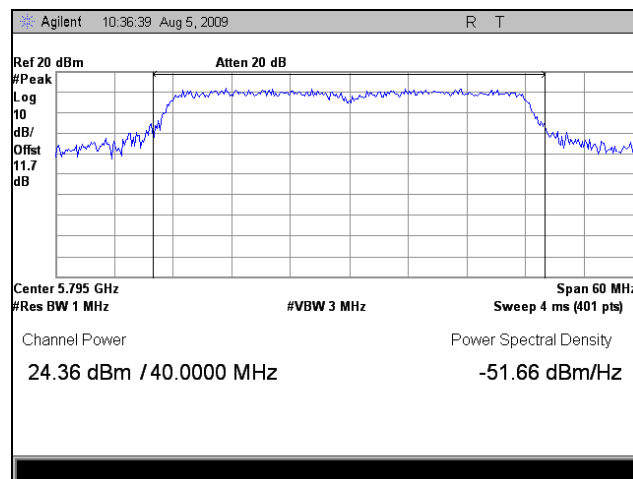
Plot 68. Peak Output Power, High Channel, 5 GHz, Port 2, 802.11n 40MHz
