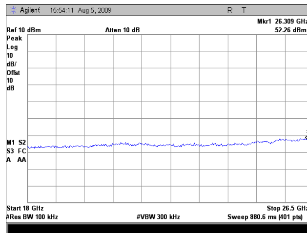
Plot 189. Conducted Emissions, High Channel, 5 GHz, Port 1, 802.11n 40MHz, 18 GHz – 26.5 GHz
