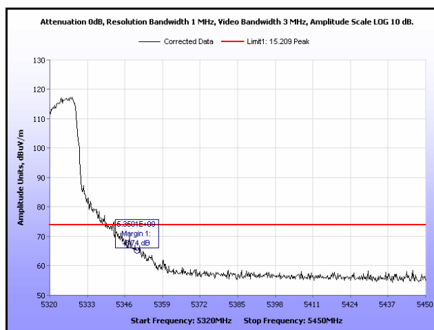
Plot 102. Restricted Band Edge, 802.11n 20 MHz, 5320 MHz, Peak, 9 dBi Antenna
