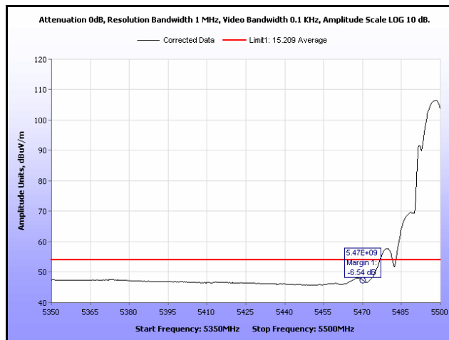
Plot 91. Restricted Band Edge, 802.11a 20 MHz, 5500 MHz, Average, 9 dBi Antenna
