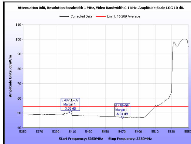
Plot 183. Restricted Band Edge, 802.11n 40 MHz, 5550 MHz, Average, 19 dBi Antenna
