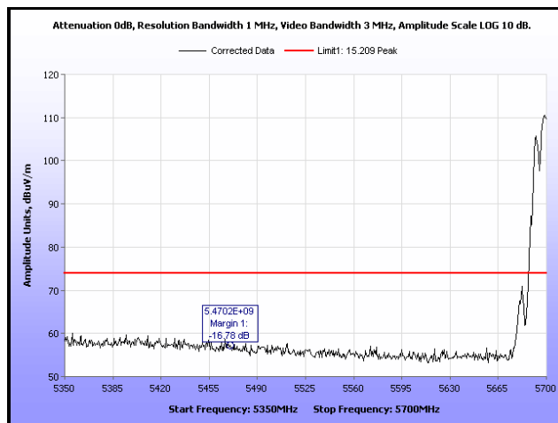
Plot 164. Restricted Band Edge, 802.11a 20 MHz, 5700 MHz, Peak, 19 dBi Antenna
