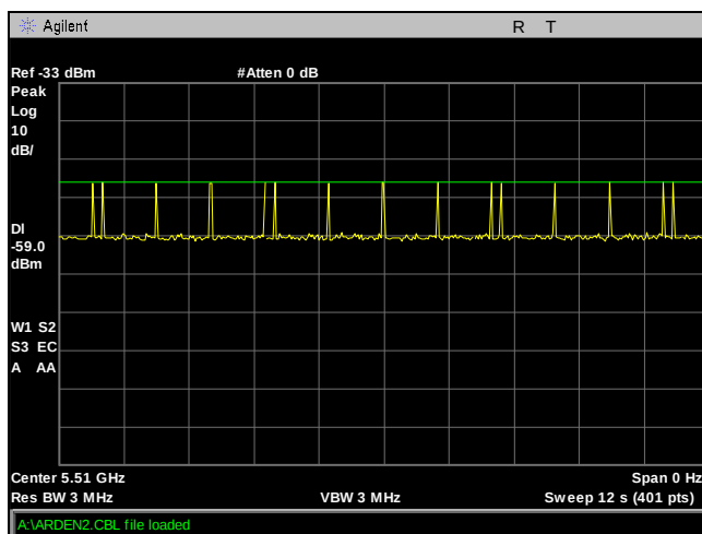
Plot 200. Radar Waveform Calibration, Radar Type 5, 5510 MHz, PS 15.8 dBm
