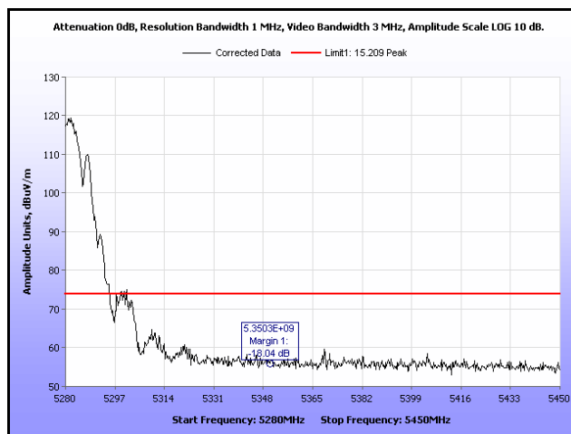
Plot 88. Restricted Band Edge, 802.11a 20 MHz, 5280 MHz, Peak, 9 dBi Antenna
