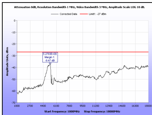
Plot 82. Radiated Spurious Emissions, 802.11n 40 MHz, 5510 MHz, 1 GHz – 18 GHz, 19 dBi Antenna
