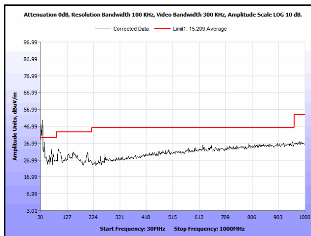
Plot 26. Radiated Spurious Emissions, 802.11n 40 MHz, 5510 MHz, 30 MHz – 1 GHz, Average, 16 dBi Antenna
