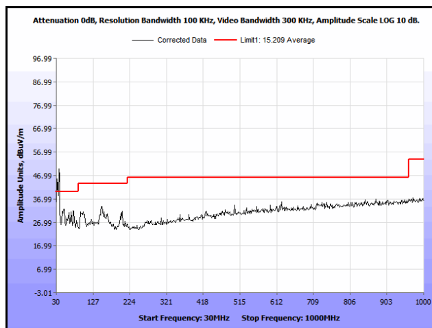
Plot 31. Radiated Spurious Emissions, 802.11n 40 MHz, 5510 MHz, 30 MHz – 1 GHz, Average, 19 dBi Antenna
