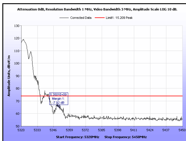
Plot 90. Restricted Band Edge, 802.11a 20 MHz, 5320 MHz, Peak, 9 dBi Antenna
