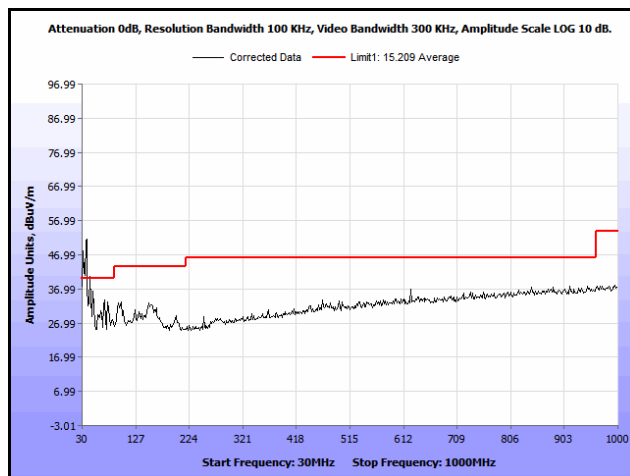
Plot 19. Radiated Spurious Emissions, 802.11n 40 MHz, 5270 MHz, 30 MHz – 1 GHz, Average, 9 dBi Antenna
