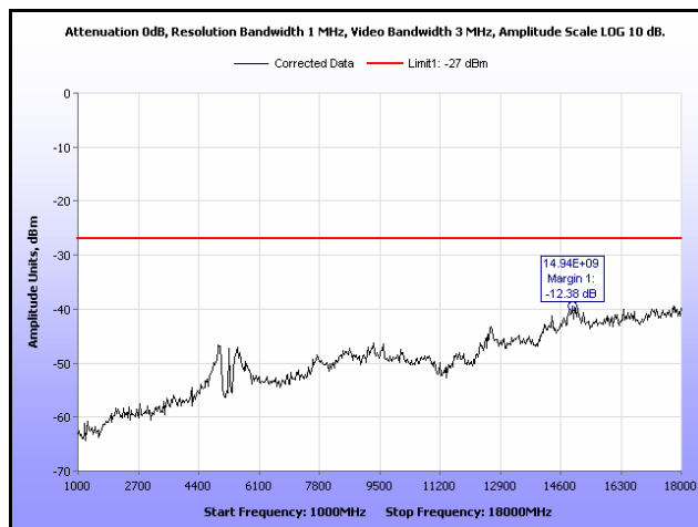
Plot 51. Radiated Spurious Emissions, 802.11a 20 MHz, 5260 MHz, 1 GHz – 18 GHz, 16 dBi Antenna
