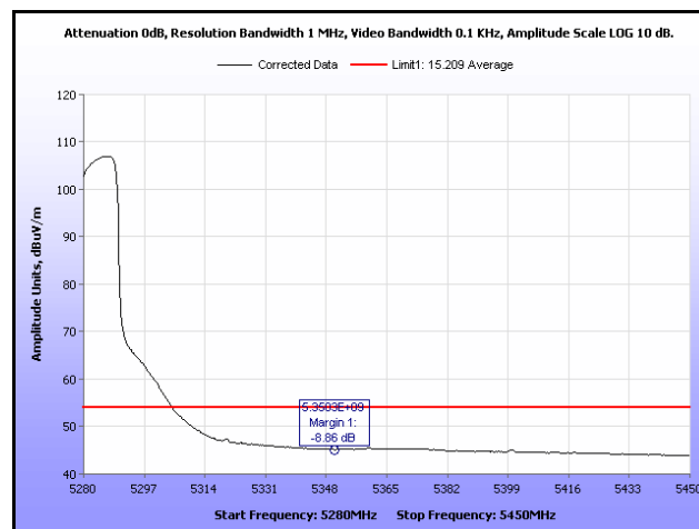
Plot 99. Restricted Band Edge, 802.11n 20 MHz, 5280 MHz, Average, 9 dBi Antenna
