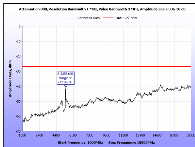
Plot 76. Radiated Spurious Emissions, 802.11n 20 MHz, 5320 MHz, 1 GHz – 18 GHz, 19 dBi Antenna
