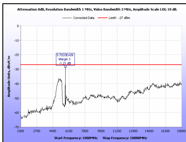
Plot 45. Radiated Spurious Emissions, 802.11n 20 MHz, 5700 MHz, 1 GHz – 18 GHz, 9 dBi Antenna
