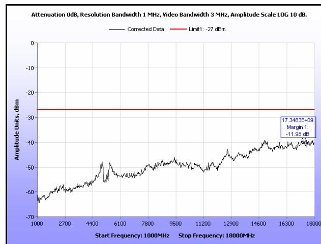
Plot 75. Radiated Spurious Emissions, 802.11n 20 MHz, 5280 MHz, 1 GHz – 18 GHz, 19 dBi Antenna
