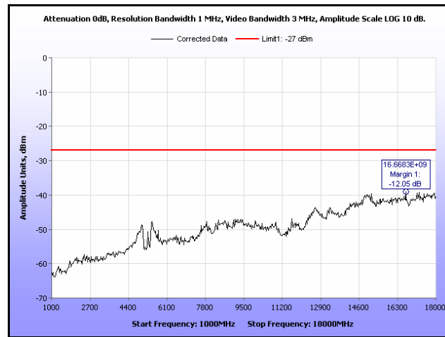
Plot 74. Radiated Spurious Emissions, 802.11n 20 MHz, 5260 MHz, 1 GHz – 18 GHz, 19 dBi Antenna
