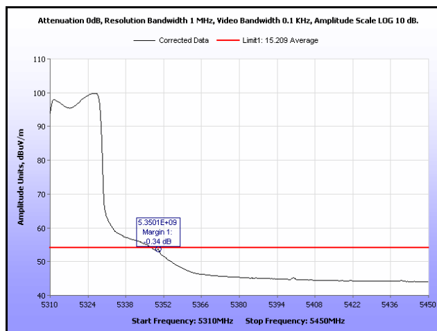
Plot 145. Restricted Band Edge, 802.11n 40 MHz, 5310 MHz, Average, 16 dBi Antenna
