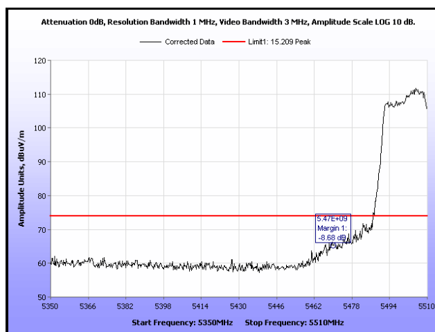
Plot 182. Restricted Band Edge, 802.11n 40 MHz, 5510 MHz, Peak, 19 dB Antenna
