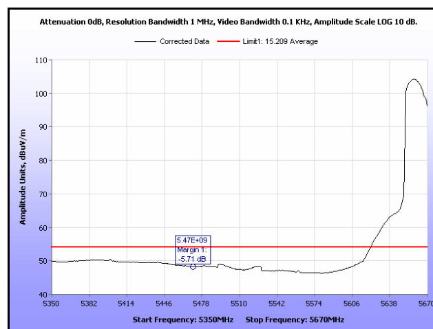
Plot 151. Restricted Band Edge, 802.11n 40 MHz, 5670 MHz, Average, 16 dBi Antenna
