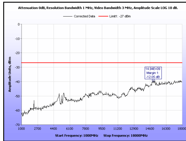
Plot 68. Radiated Spurious Emissions, 802.11a 20 MHz, 5260 MHz, 1 GHz – 18 GHz, 19 dBi Antenna
