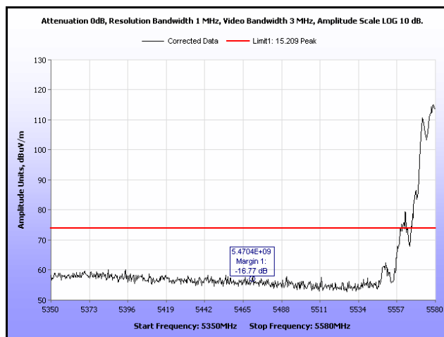
Plot 94. Restricted Band Edge, 802.11a 20 MHz, 5580 MHz, Peak, 9 dBi Antenna
