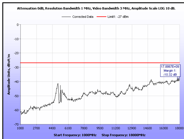
Plot 40. Radiated Spurious Emissions, 802.11n 20 MHz, 5260 MHz, 1 GHz – 18 GHz, 9 dBi Antenna
