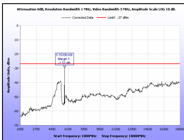
Plot 56. Radiated Spurious Emissions, 802.11a 20 MHz, 5700 MHz, 1 GHz – 18 GHz, 16 dBi Antenna
