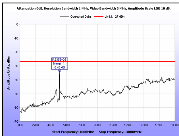
Plot 53. Radiated Spurious Emissions, 802.11a 20 MHz, 5320 MHz, 1 GHz – 18 GHz, 16 dBi Antenna
