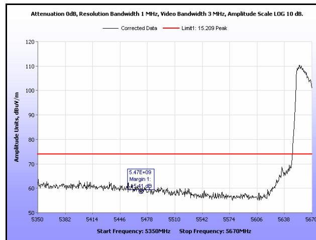
Plot 186. Restricted Band Edge, 802.11n 40 MHz, 5670 MHz, Peak, 19 dBi Antenna
