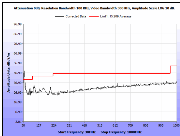
Plot 24. Radiated Spurious Emissions, 802.11n 40 MHz, 5270 MHz, 30 MHz – 1 GHz, Average, 16 dBi Antenna
