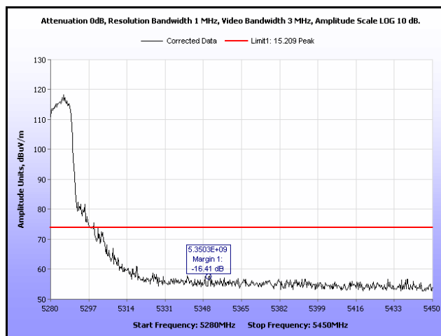
Plot 100. Restricted Band Edge, 802.11n 20 MHz, 5280 MHz, Peak, 9 dBi Antenna
