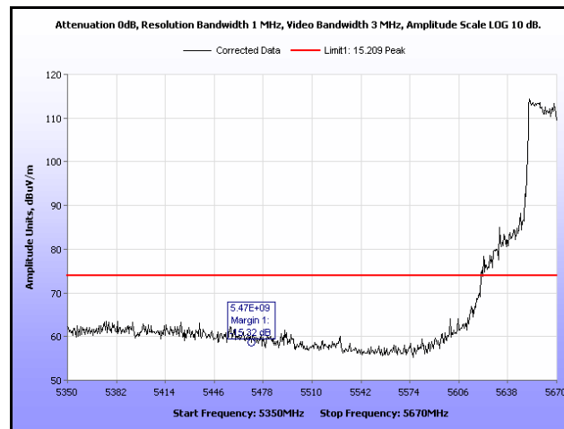
Plot 118. Restricted Band Edge, 802.11n 40 MHz, 5670 MHz, Peak, 9 dBi Antenna
