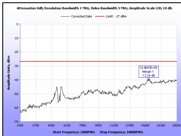
Plot 80. Radiated Spurious Emissions, 802.11n 40 MHz, 5270 MHz, 1 GHz – 18 GHz, 19 dBi Antenna
