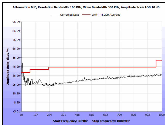
Plot 22. Radiated Spurious Emissions, 802.11n 40 MHz, 5590 MHz, 30 MHz – 1 GHz, Average, 9 dBi Antenna
