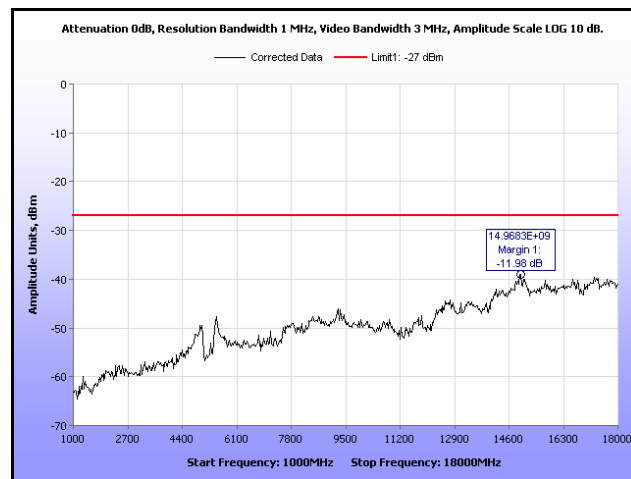
Plot 69. Radiated Spurious Emissions, 802.11a 20 MHz, 5280 MHz, 1 GHz – 18 GHz, 19 dBi Antenna
