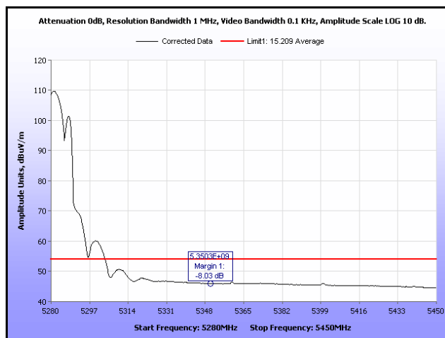
Plot 87. Restricted Band Edge, 802.11a 20 MHz, 5280 MHz, Average, 9 dBi Antenna
