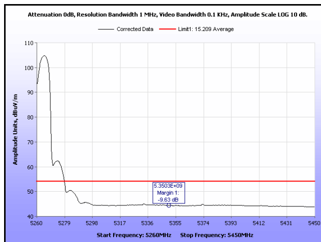
Plot 119. Restricted Band Edge, 802.11a 20 MHz, 5260 MHz, Average, 16 dBi Antenna
