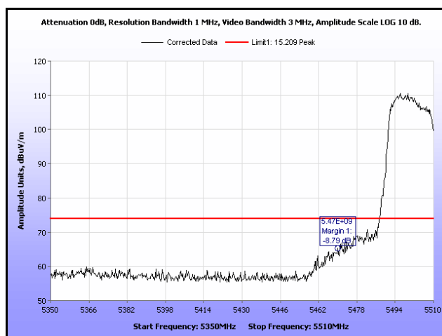
Plot 148. Restricted Band Edge, 802.11n 40 MHz, 5510 MHz, Peak, 16 dBi Antenna
