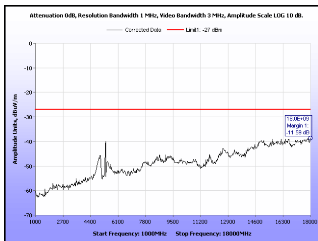
Plot 47. Radiated Spurious Emissions, 802.11n 40 MHz, 5310 MHz, 1 GHz – 18 GHz, 9 dBi Antenna
