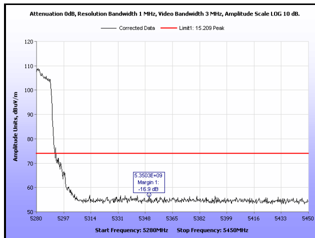
Plot 168. Restricted Band Edge, 802.11n 20 MHz, 5280 MHz, Peak, 19 dBi Antenna
