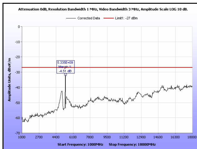
Plot 36. Radiated Spurious Emissions, 802.11a 20 MHz, 5320 MHz, 1 GHz – 18 GHz, 9 dBi Antenna
