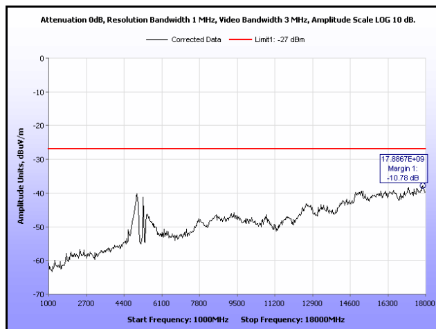
Plot 34. Radiated Spurious Emissions, 802.11a 20 MHz, 5260 MHz, 1 GHz – 18 GHz, 9 dBi Antenna
