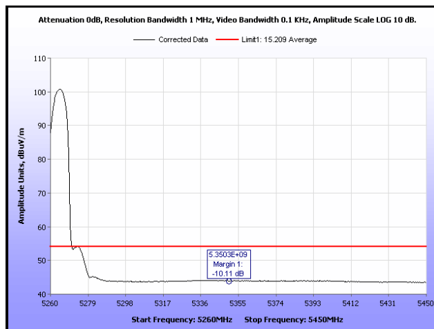
Plot 153. Restricted Band Edge, 802.11a 20 MHz, 5260 MHz, Average, 19 dBi Antenna
