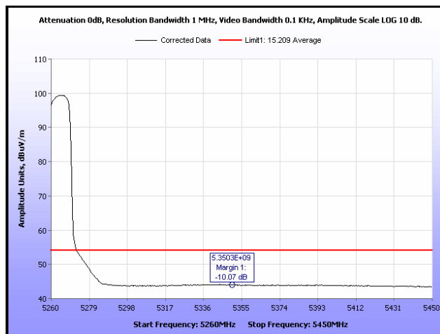
Plot 165. Restricted Band Edge, 802.11n 20 MHz, 5260 MHz, Average, 19 dBi Antenna
