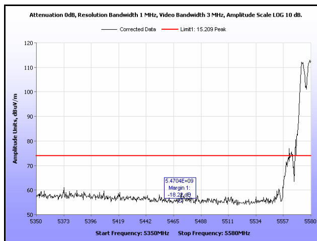
Plot 128. Restricted Band Edge, 802.11a 20 MHz, 5580 MHz, Peak, 16 dBi Antenna
