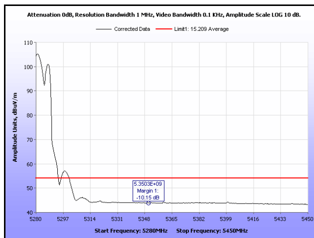
Plot 121. Restricted Band Edge, 802.11a 20 MHz, 5280 MHz, Average, 16 dBi Antenna
