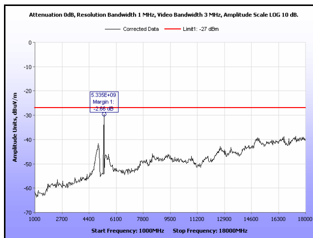
Plot 42. Radiated Spurious Emissions, 802.11n 20 MHz, 5320 MHz, 1 GHz – 18 GHz, 9 dBi Antenna
