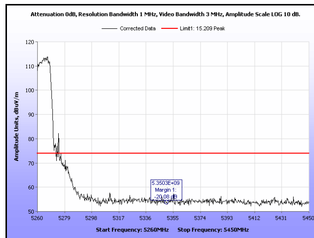
Plot 132. Restricted Band Edge, 802.11n 20 MHz, 5260 MHz, Peak, 16 dBi Antenna
