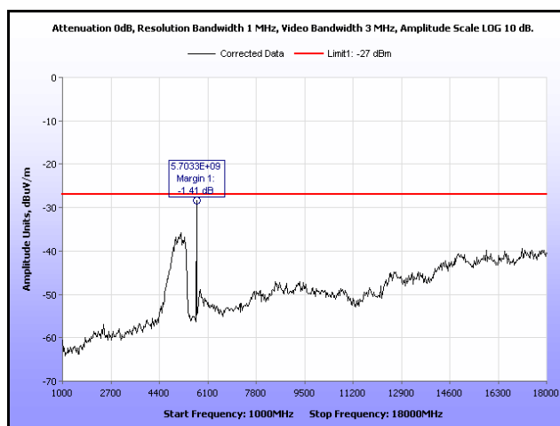
Plot 39. Radiated Spurious Emissions, 802.11a 20 MHz, 5700 MHz, 1 GHz – 18 GHz, 9 dBi Antenna
