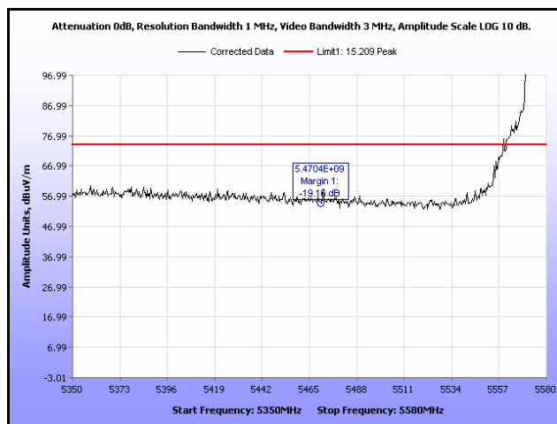
Plot 106. Restricted Band Edge, 802.11n 20 MHz, 5580 MHz, Peak, 9 dBi Antenna
