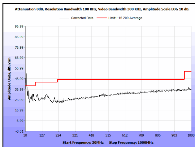
Plot 21. Radiated Spurious Emissions, 802.11n 40 MHz, 5510 MHz, 30 MHz – 1 GHz, Average, 9 dBi Antenna
