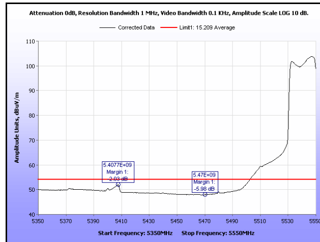
Plot 149. Restricted Band Edge, 802.11n 40 MHz, 5550 MHz, Average, 16 dBi Antenna
