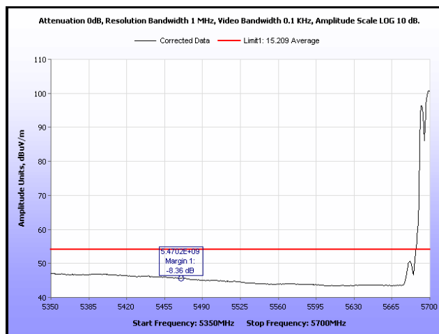
Plot 163. Restricted Band Edge, 802.11a 20 MHz, 5700 MHz, Average, 19 dBi Antenna
