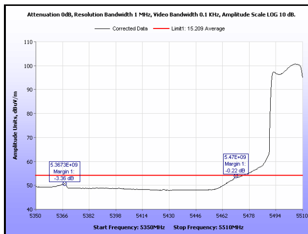
Plot 181. Restricted Band Edge, 802.11n 40 MHz, 5510 MHz, Average, 19 dB Antenna
