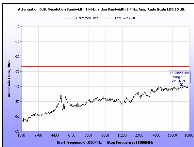
Plot 58. Radiated Spurious Emissions, 802.11n 20 MHz, 5280 MHz, 1 GHz – 18 GHz, 16 dBi Antenna
