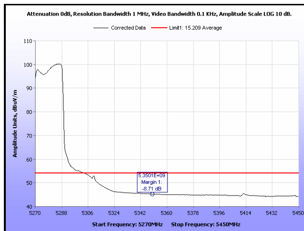
Plot 177. Restricted Band Edge, 802.11n 40 MHz, 5270 MHz, Average, 19 dBi Antenna
