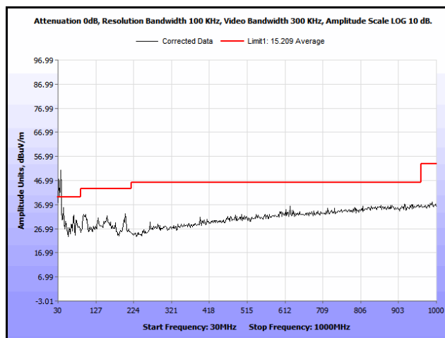
Plot 27. Radiated Spurious Emissions, 802.11n 40 MHz, 5590 MHz, 30 MHz – 1 GHz, Average, 16 dBi Antenna
