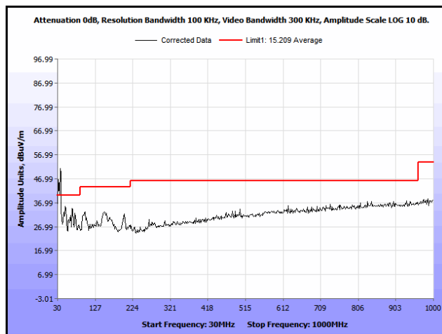
Plot 29. Radiated Spurious Emissions, 802.11n 40 MHz, 5270 MHz, 30 MHz – 1 GHz, Average, 19 dBi Antenna
