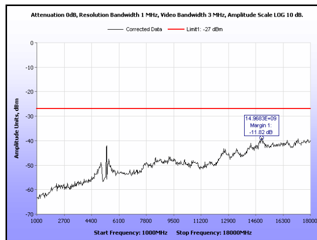
Plot 70. Radiated Spurious Emissions, 802.11a 20 MHz, 5320 MHz, 1 GHz – 18 GHz, 19 dBi Antenna
