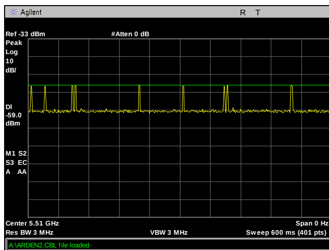
Plot 202. Radar Waveform Calibration, Radar Type 6, 5510 MHz, PS 15.8 dBm
