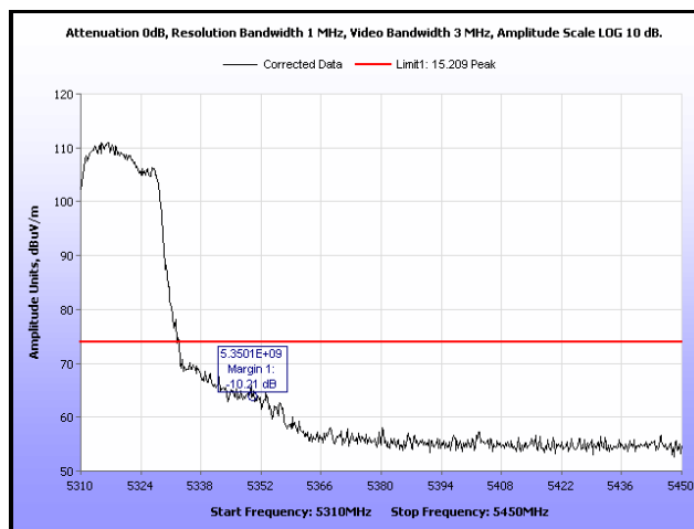
Plot 180. Restricted Band Edge, 802.11n 40 MHz, 5310 MHz, Peak, 19 dB Antenna
