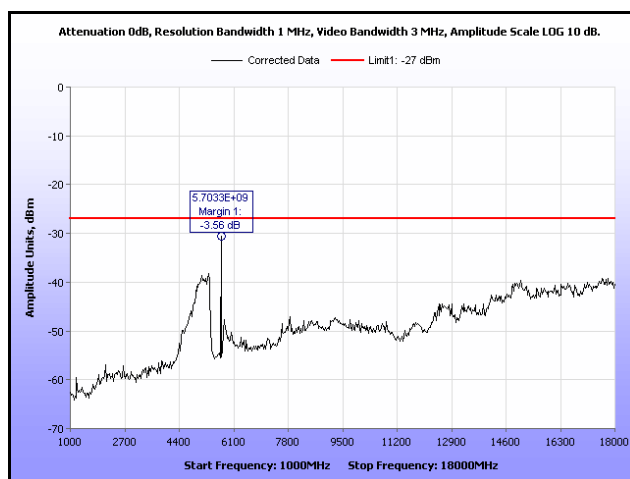
Plot 62. Radiated Spurious Emissions, 802.11n 20 MHz, 5700 MHz, 1 GHz – 18 GHz, 16 dBi Antenna
