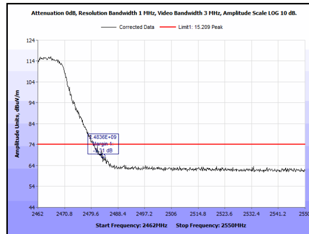
Plot 224. Radiated Restricted Band Edge, High Channel, 802.11n 20 MHz, Peak, 13 dBi Antenna
