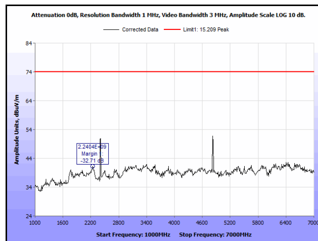
Plot 79. Radiated Spurious Emissions, Low Channel, 802.11b, 1 GHz – 7 GHz, Peak, 9 dBi Antenna
