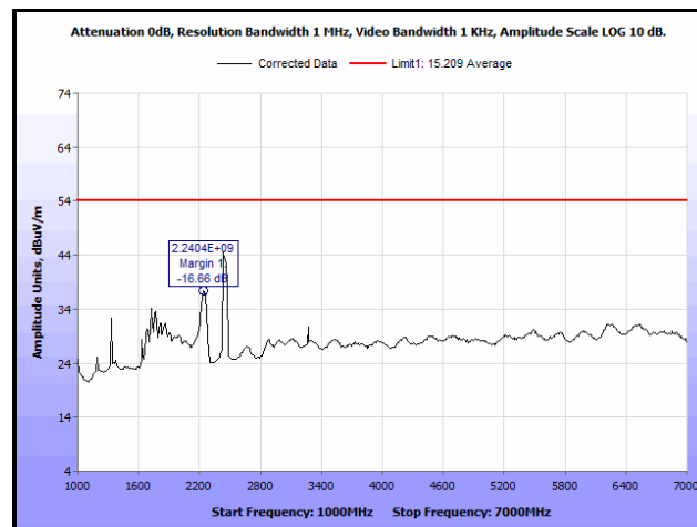
Plot 193. Radiated Spurious Emissions, High Channel, 802.11n 40 MHz, 1 GHz – 7 GHz, Average, 13 dBi Antenna
