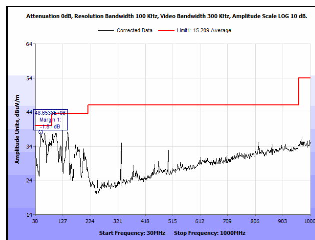
Plot 157. Radiated Spurious Emissions, Mid Channel, 802.11g, 30 MHz – 1 GHz, 13 dBi Antenna
