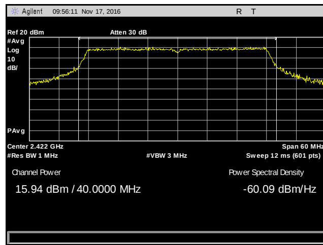
Plot 38. Peak Power Output, Low Channel, 802.11n 40 MHz, Antenna 1, 9 dBi Antenna
