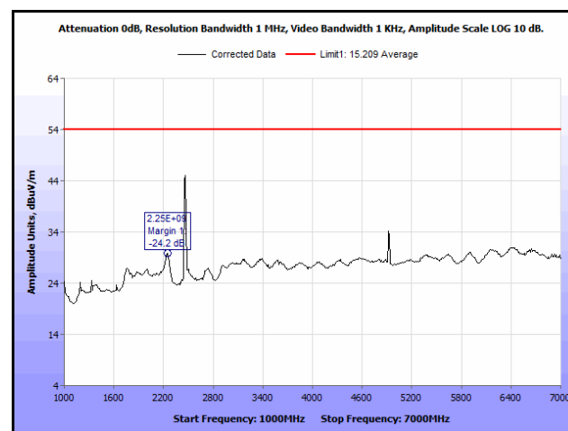
Plot 88. Radiated Spurious Emissions, High Channel, 802.11b, 1 GHz – 7 GHz, Average, 9 dBi Antenna
