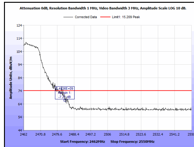
Plot 204. Radiated Restricted Band Edge, High Channel, 802.11g, Peak, 9 dBi Antenna
