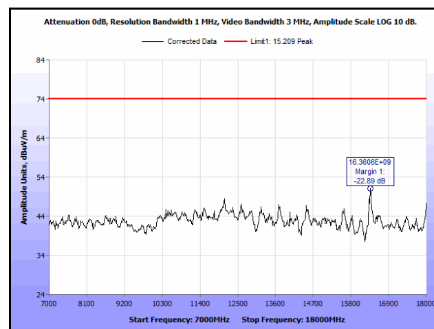
Plot 136. Radiated Spurious Emissions, High Channel, 802.11n 40 MHz, 7 GHz – 18 GHz, Peak, 9 dBi Antenna
