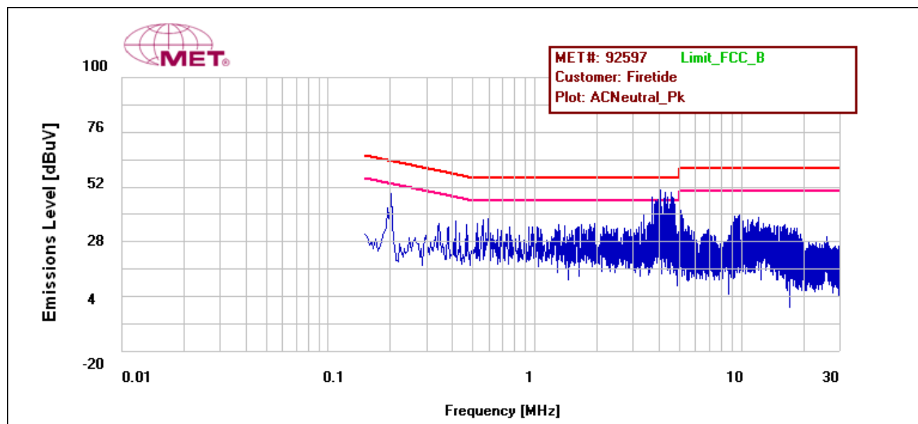
Plot 2. Conducted Emissions, 15.207(a), Neutral Line, 9 dBi Antenna
