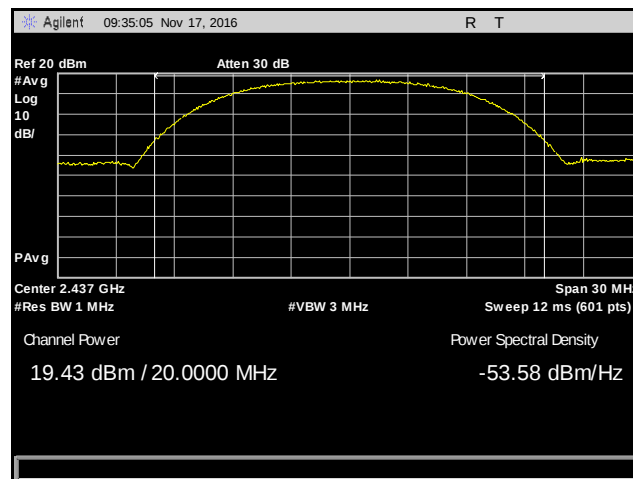
Plot 30. Peak Power Output, Mid Channel, 802.11b, Antenna 1, 9 dBi Antenna
