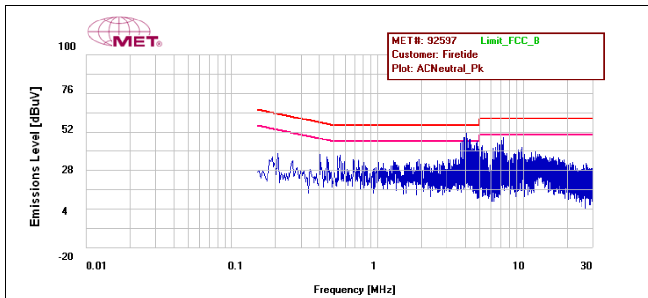
Plot 4. Conducted Emissions, 15.207(a), Neutral Line, 13 dBi Antenna
