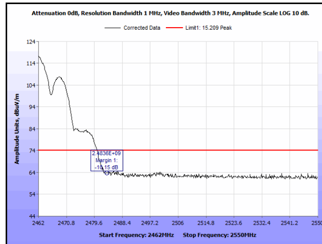
Plot 216. Radiated Restricted Band Edge, High Channel, 802.11b, Peak, 13 dBi Antenna
