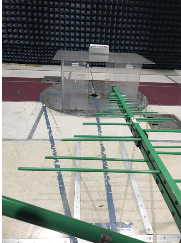
Photograph 1. Radiated Spurious Emissions, Test Setup, 30 MHz – 1 GHz
