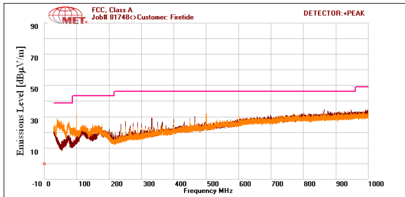
Plot 3. Radiated Emissions, Pre-Scan, FCC Limits, 30 MHz – 1 GHz
