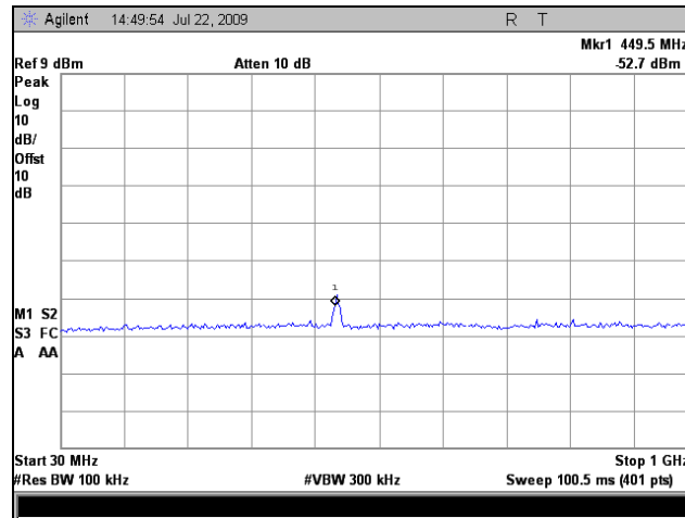
Plot 101. Conducted Emissions, Low Channel, 2.4 GHz, 802.11g, Port 1, 30 MHz – 1 GHz
