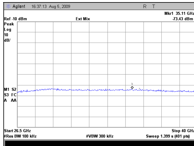
Plot 183. Conducted Emissions, High Channel, 5 GHz, Port 2, 802.11n 20MHz, 26.5 GHz – 40 GHz
