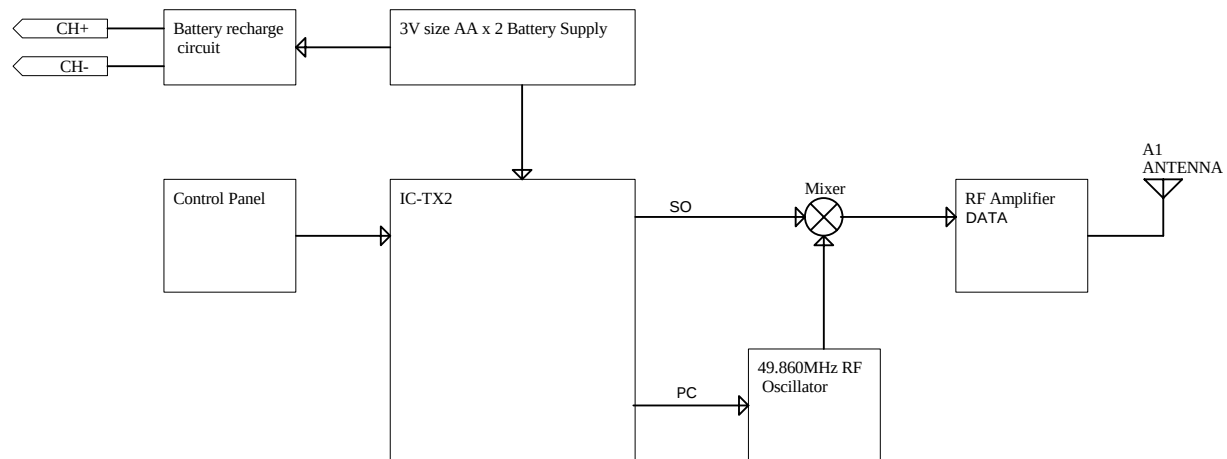
Block diagram
