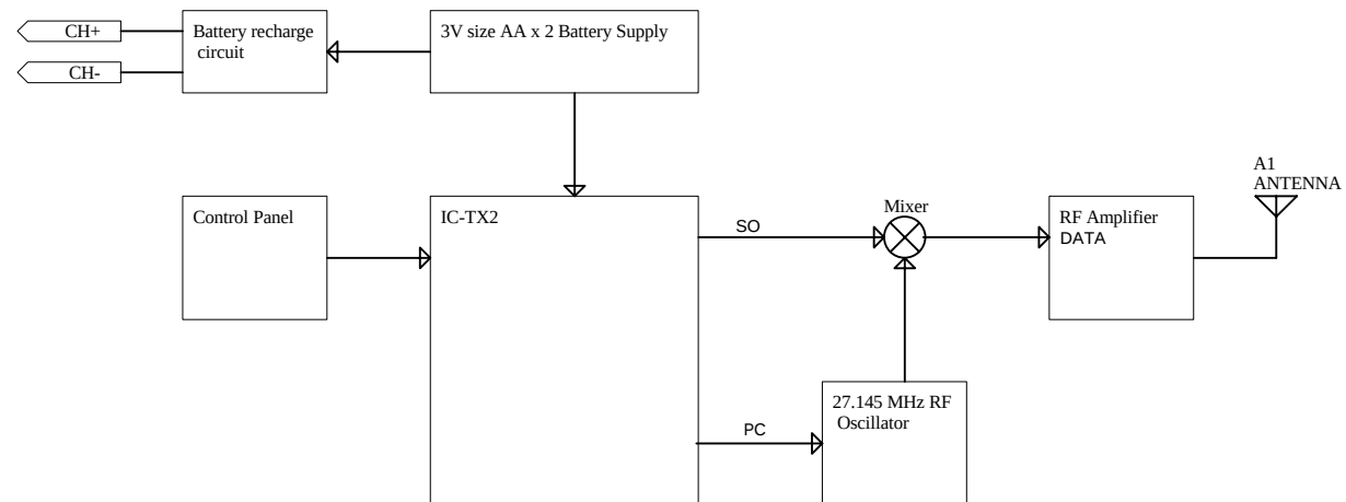
Block diagram
