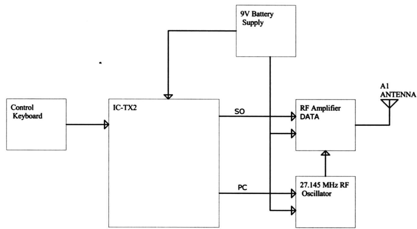
Block diagram
