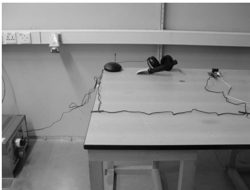
Photograph 1: Set-up for Conducted Emission on AC Mains
