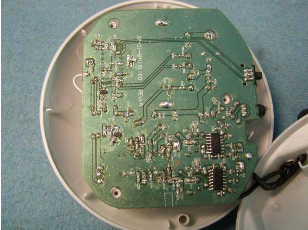
SP1291, SP1091, SP1191A, SP2091 and SP2191 internal photo
